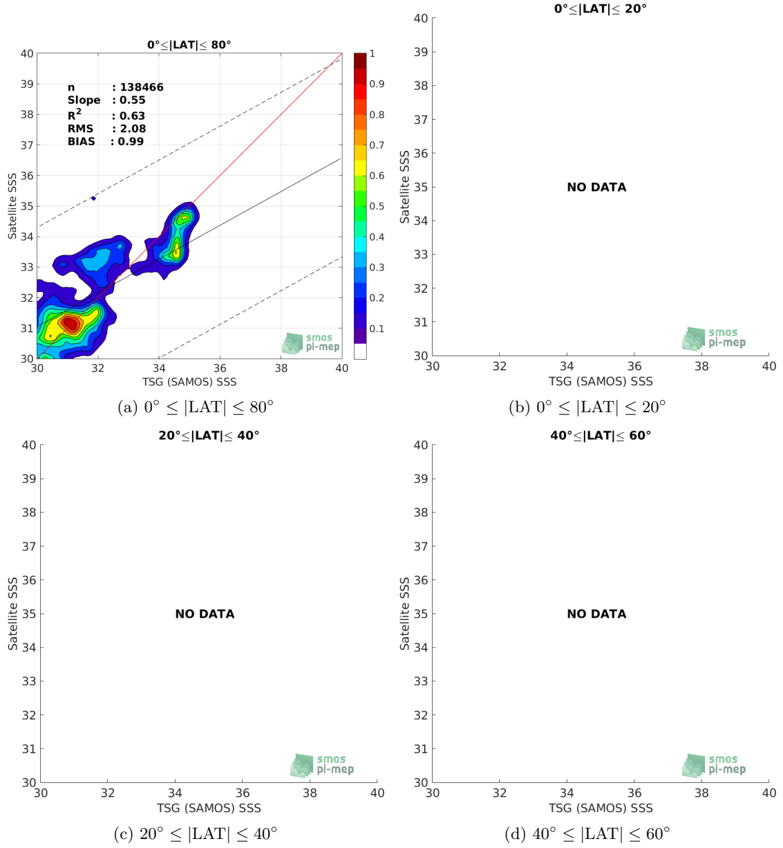
Figure 9: Contour maps of the concentration of SMOS L3 v2 - 9-Days (BEC) SSS (y-axis) versus TSG (SAMOS) SSS (x-axis) at match-up pairs for different latitude bands. For each plot, the red line shows x=y . The black thin and dashed lines indicate a linear fit through the data cloud and the \pm 95\% confidence levels, respectively. The number match-up pairs n , the slope and R^2 coefficient of the linear fit, the root mean square (RMS) and the mean bias between satellite and in situ data are indicated for each latitude band in each plots.
