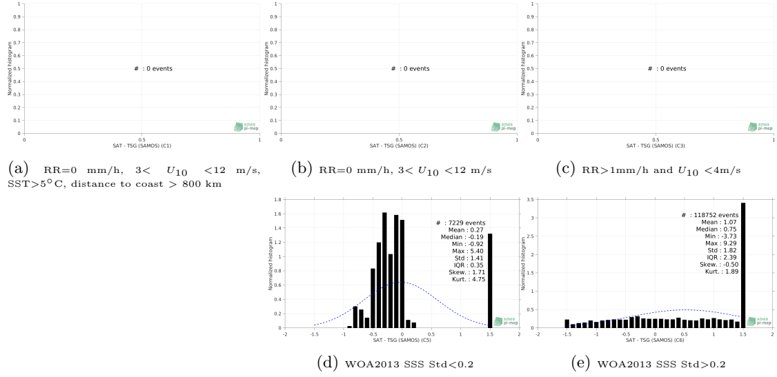
Figure 13: Normalized histogram of \Delta\text{SSS} (SMOS L3 v2 - 9-Days (BEC) - TSG (SAMOS)) for 5 different subdatasets corresponding to: RR=0 mm/h, 3 < U_{10} < 12 m/s, SST > 5^\circ\text{C} , distance to coast > 800 km (a), RR=0 mm/h, 3 < U_{10} < 12 m/s (b), RR > 1 mm/h and U_{10} < 4 m/s (c), WOA2013 SSS Std < 0.2 (d), WOA2013 SSS Std > 0.2 (e).
