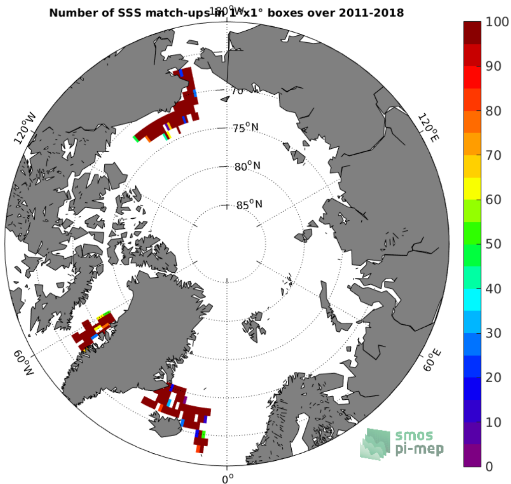
Figure 4: Number of SSS match-ups between TSG (SAMOS) SSS and the SMOS L3 v2 - 9-Days (BEC) SSS product for the Arctic Ocean Pi-MEP region over 1°x1° boxes and for the full satellite product period.
