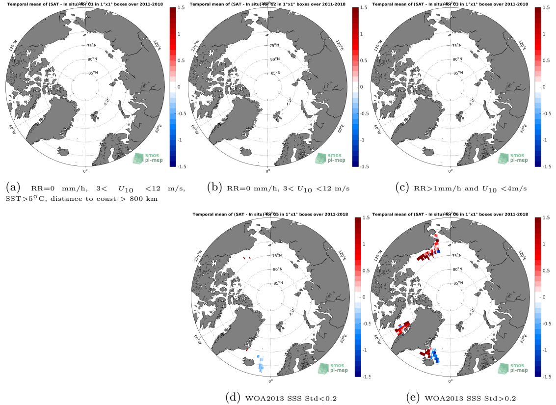
Figure 12: Temporal mean gridded over spatial boxes of size 1^{\circ}\times 1^{\circ} of \Delta\text{SSS} (SMOS L3 v2 - 9-Days (BEC) - TSG (SAMOS)) for 5 different subdatasets corresponding to:RR=0 mm/h, 3 < U_{10} < 12 m/s, SST >5^{\circ}\text{C} , distance to coast > 800 km (a), RR=0 mm/h, 3 < U_{10} < 12 m/s (b), RR >1 mm/h and U_{10} < 4 m/s (c), WOA2013 SSS Std <0.2 (d), WOA2013 SSS Std >0.2 (e).
