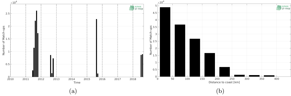
Figure 1: Number of match-ups between TSG (SAMOS) and SMOS L3 v2 - 9-Days (BEC) SSS as a function of time (a) and as function of the distance to coast (b) over the Arctic Ocean Pi-MEP region and for the full satellite product period.
