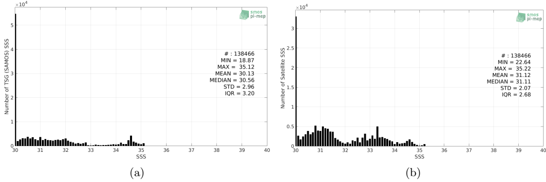
Figure 2: Histograms of SSS from TSG (SAMOS) (a) and SMOS L3 v2 - 9-Days (BEC) (b) considering all match-up pairs per bins of 0.1 over the Arctic Ocean Pi-MEP region and for the full satellite product period.
