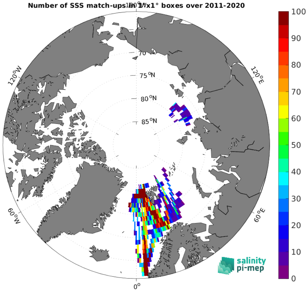
Figure 5: Number of SSS match-ups between TSG (Polarstern) SSS and the SMOS SSS L3 v2 - 9-Days (BEC) SSS product for the Arctic Ocean Pi-MEP region over 1^\circ \times 1^\circ boxes and for the full satellite product period.
