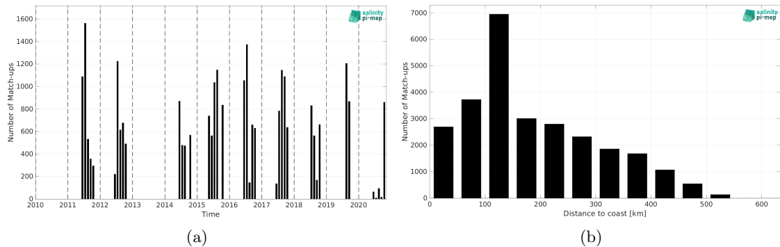
Figure 2: Number of match-ups between TSG (Polarstern) and SMOS SSS L3 v2 - 9-Days (BEC) SSS as a function of time (a) and as function of the distance to coast (b) over the Arctic Ocean Pi-MEP region and for the full satellite product period.
