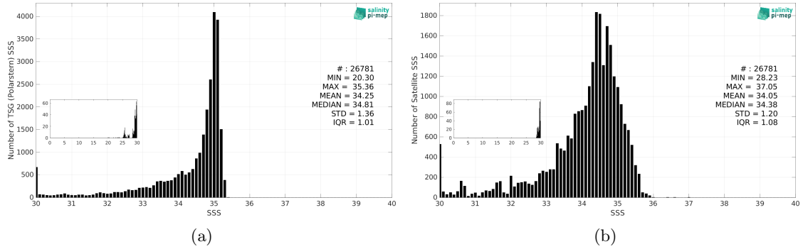
Figure 3: Histograms of SSS from TSG (Polarstern) (a) and SMOS SSS L3 v2 - 9-Days (BEC) (b) considering all match-up pairs per bins of 0.1 over the Arctic Ocean Pi-MEP region and for the full satellite product period.
