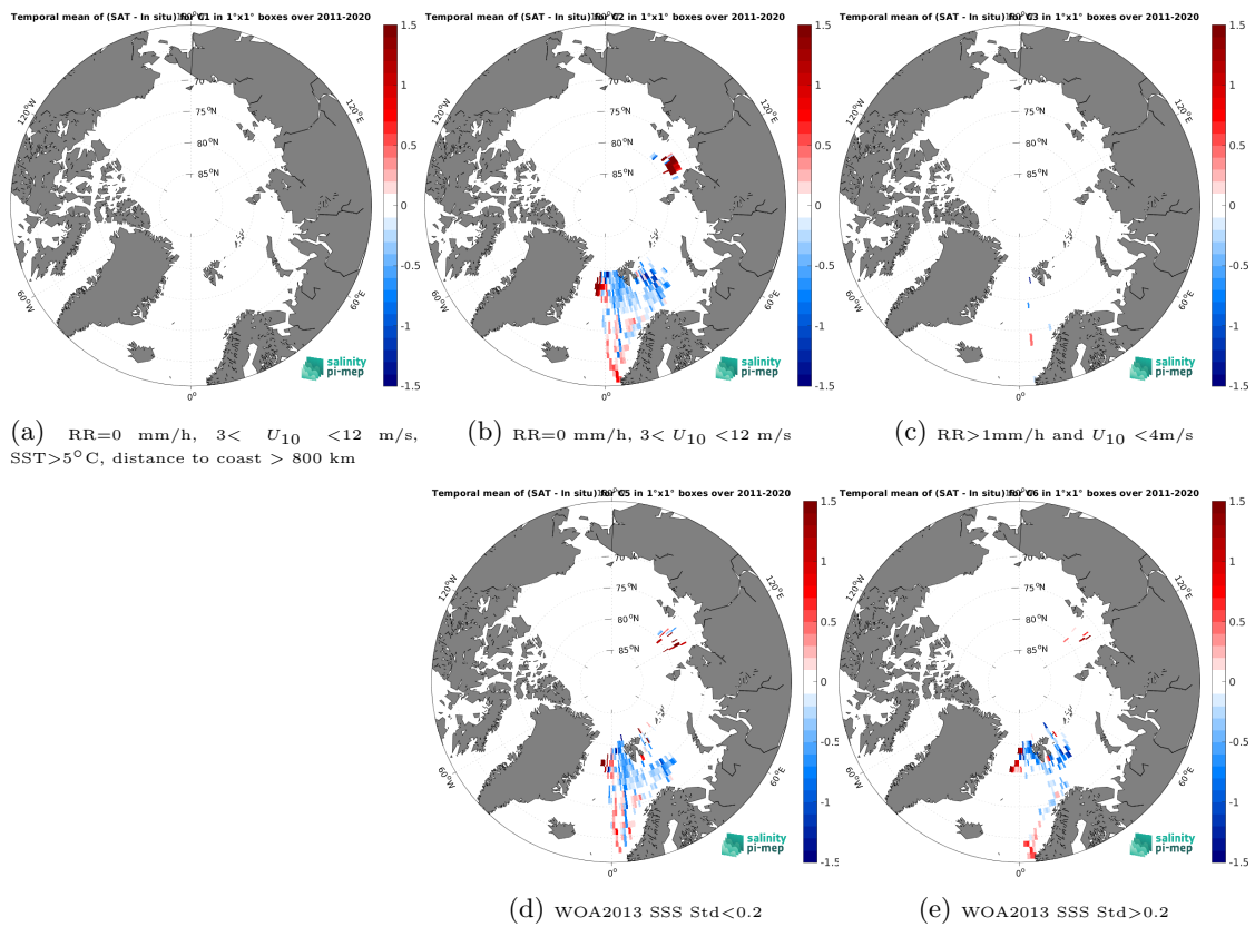
Figure 14: Temporal mean gridded over spatial boxes of size 1^\circ \times 1^\circ of \Delta SSS (SMOS SSS L3 v2 - 9-Days (BEC) - TSG (Polarstern)) for 5 different subdatasets corresponding to:RR=0 mm/h, 3 < U_{10} < 12 m/s, SST>5°C, distance to coast > 800 km (a), RR=0 mm/h, 3 < U_{10} < 12 m/s (b), RR>1mm/h and U_{10} < 4 m/s (c), WOA2013 SSS Std<0.2 (d), WOA2013 SSS Std>0.2 (e).
