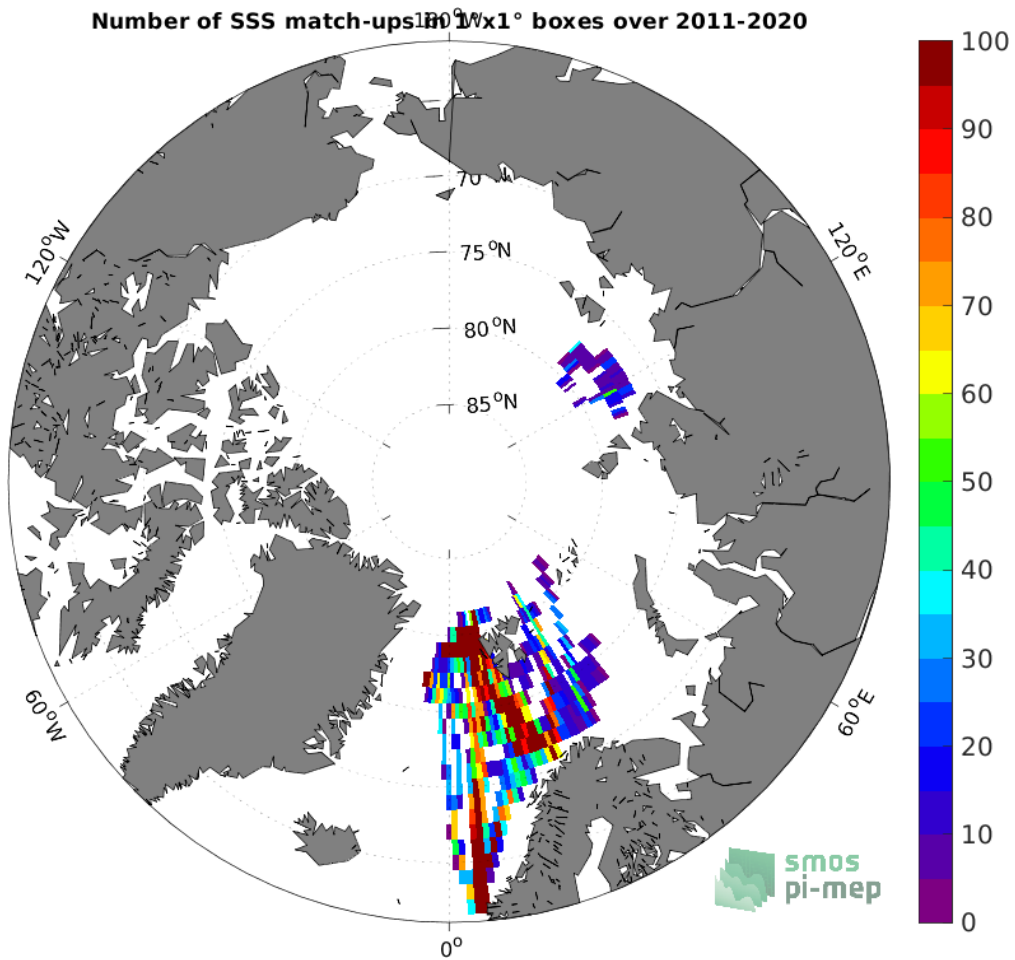
Figure 4: Number of SSS match-ups between TSG (Polarstern) SSS and the SMOS SSS L3 v2 - 9-Days (BEC) SSS product for the Arctic Ocean Pi-MEP region over 1^{\circ} \times 1^{\circ} boxes and for the full satellite product period.
