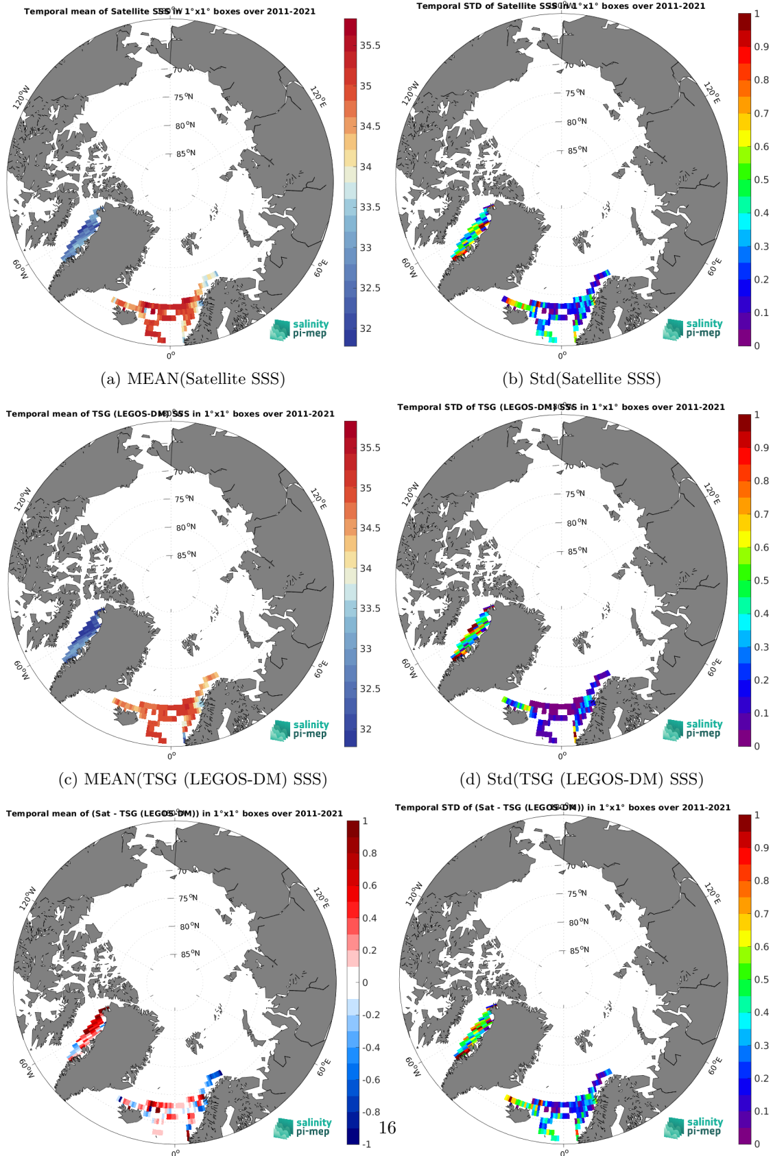
(e) MEAN( \Delta SSS) (Satellite - TSG (LEGOS-DM)) (f) Std( \Delta SSS) (Satellite - TSG (LEGOS-DM)) Figure 7: Temporal mean (left) and Std (right) of SSS from SMOS SSS L3 v2 - 9-Days (BEC) (top), TSG (LEGOS-DM) (middle), and of \Delta SSS (Satellite - TSG (LEGOS-DM)). Only match-up pairs are used to generate these maps.
