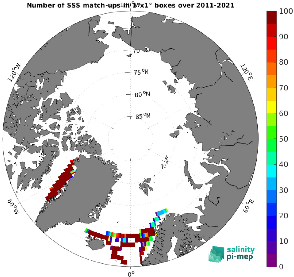
Figure 5: Number of SSS match-ups between TSG (LEGOS-DM) SSS and the SMOS SSS L3 v2 - 9-Days (BEC) SSS product for the Arctic Ocean Pi-MEP region over 1^\circ \times 1^\circ boxes and for the full satellite product period.
