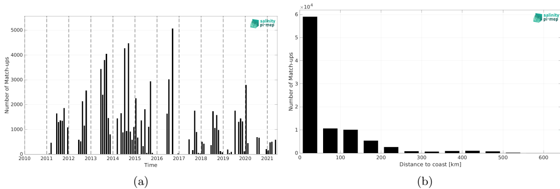
Figure 2: Number of match-ups between TSG (LEGOS-DM) and SMOS SSS L3 v2 - 9-Days (BEC) SSS as a function of time (a) and as function of the distance to coast (b) over the Arctic Ocean Pi-MEP region and for the full satellite product period.
