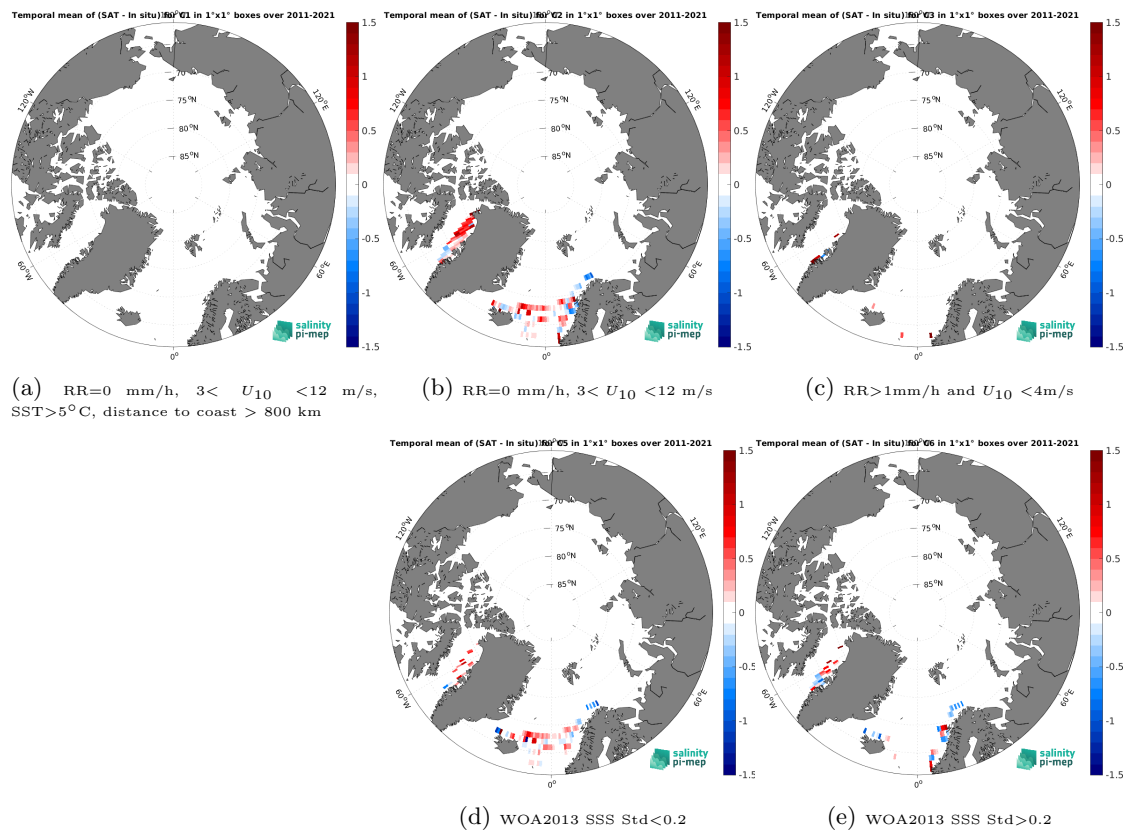
Figure 14: Temporal mean gridded over spatial boxes of size 1^\circ \times 1^\circ of \Delta\text{SSS} (SMOS SSS L3 v2 - 9-Days (BEC) - TSG (LEGOS-DM)) for 5 different subdatasets corresponding to:RR=0 mm/h, 3 < U_{10} < 12 m/s, SST>5°C, distance to coast > 800 km (a), RR=0 mm/h, 3 < U_{10} < 12 m/s (b), RR>1mm/h and U_{10} < 4 m/s (c), WOA2013 SSS Std<0.2 (d), WOA2013 SSS Std>0.2 (e).
