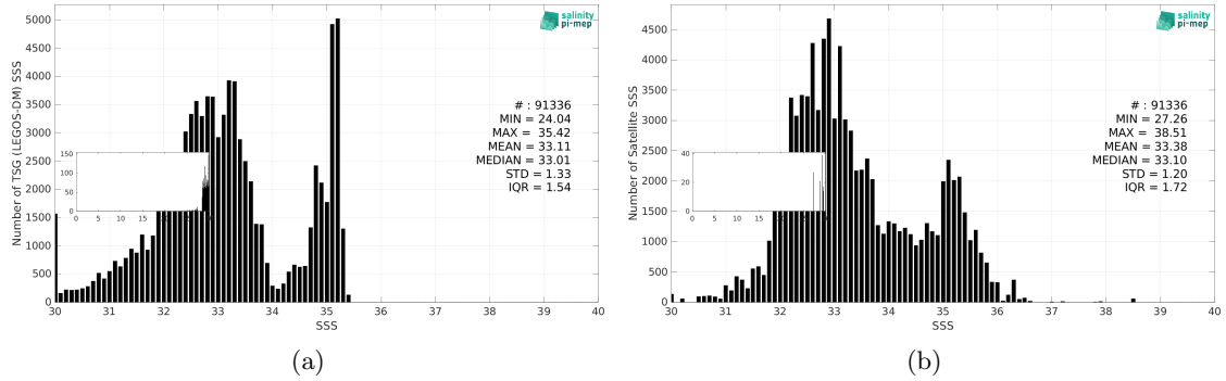
Figure 3: Histograms of SSS from TSG (LEGOS-DM) (a) and SMOS SSS L3 v2 - 9-Days (BEC) (b) considering all match-up pairs per bins of 0.1 over the Arctic Ocean Pi-MEP region and for the full satellite product period.
