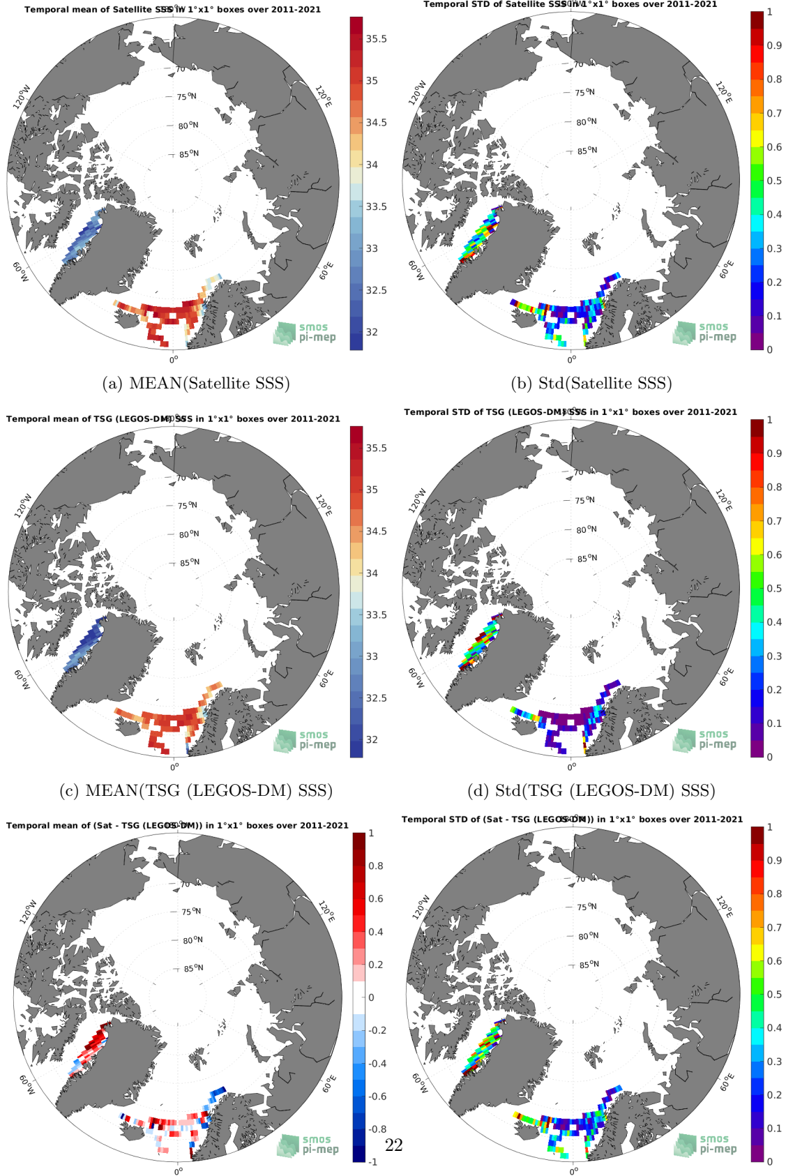
(e) MEAN( \Delta SSS) (Satellite - TSG (LEGOS-DM)) (f) Std( \Delta SSS) (Satellite - TSG (LEGOS-DM)) Figure 6: Temporal mean (left) and Std (right) of SSS from SMOS SSS L3 v2 - 9-Days (BEC) (top), TSG (LEGOS-DM) (middle), and of \Delta SSS (Satellite - TSG (LEGOS-DM)). Only match-up pairs are used to generate these maps.
