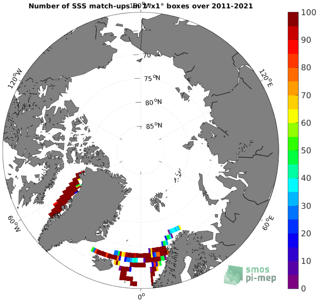
Figure 4: Number of SSS match-ups between TSG (LEGOS-DM) SSS and the SMOS SSS L3 v2 - 9-Days (BEC) SSS product for the Arctic Ocean Pi-MEP region over 1^{\circ} \times 1^{\circ} boxes and for the full satellite product period.
