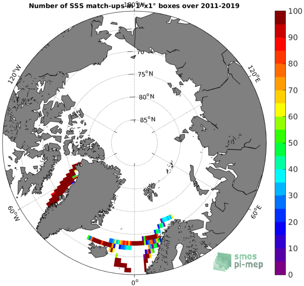
Figure 4: Number of SSS match-ups between TSG (LEGOS-DM) SSS and the SMOS SSS L3 v2 - 9-Days (BEC) SSS product for the Arctic Ocean Pi-MEP region over 1^\circ \times 1^\circ boxes and for the full satellite product period.
