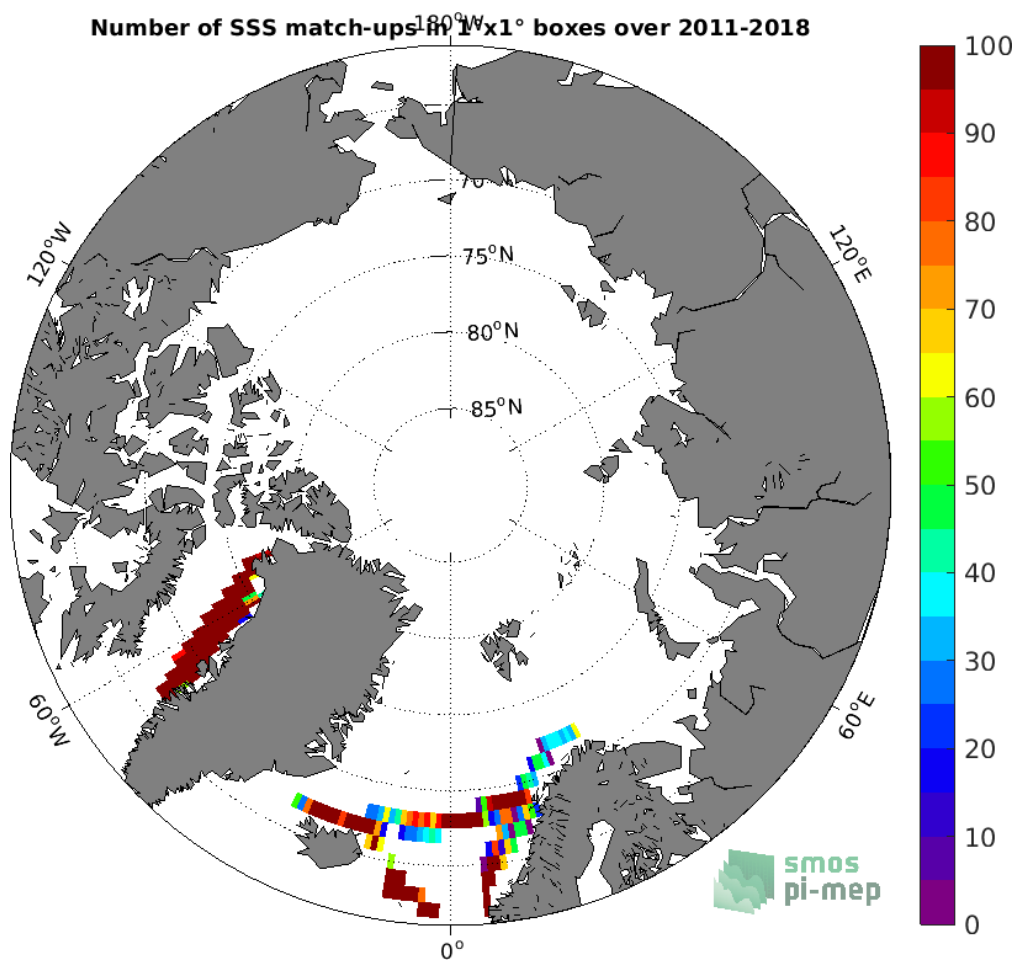
Figure 4: Number of SSS match-ups between TSG (LEGOS-DM) SSS and the SMOS SSS L3 v2 - 9-Days (BEC) SSS product for the Arctic Ocean Pi-MEP region over 1°x1° boxes and for the full satellite product period.
