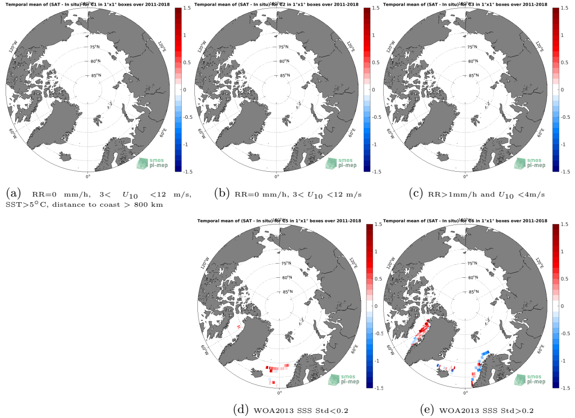
Figure 12: Temporal mean gridded over spatial boxes of size 1^{\circ}\times 1^{\circ} of \Delta\text{SSS} (SMOS SSS L3 v2 - 9-Days (BEC) - TSG (LEGOS-DM)) for 5 different subdatasets corresponding to:RR=0 mm/h, 3 < U_{10} < 12 m/s, SST >5^{\circ}\text{C} , distance to coast > 800 km (a), RR=0 mm/h, 3 < U_{10} < 12 m/s (b), RR >1 mm/h and U_{10} < 4 m/s (c), WOA2013 SSS Std <0.2 (d), WOA2013 SSS Std >0.2 (e).
