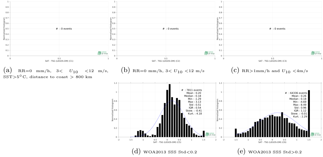
Figure 13: Normalized histogram of \Delta\text{SSS} (SMOS SSS L3 v2 - 9-Days (BEC) - TSG (LEGOS-DM)) for 5 different subdatasets corresponding to: RR=0 mm/h, 3 < U_{10} < 12 m/s, SST > 5^\circ\text{C} , distance to coast > 800 km (a), RR=0 mm/h, 3 < U_{10} < 12 m/s (b), RR > 1 mm/h and U_{10} < 4 m/s (c), WOA2013 SSS Std < 0.2 (d), WOA2013 SSS Std > 0.2 (e).
