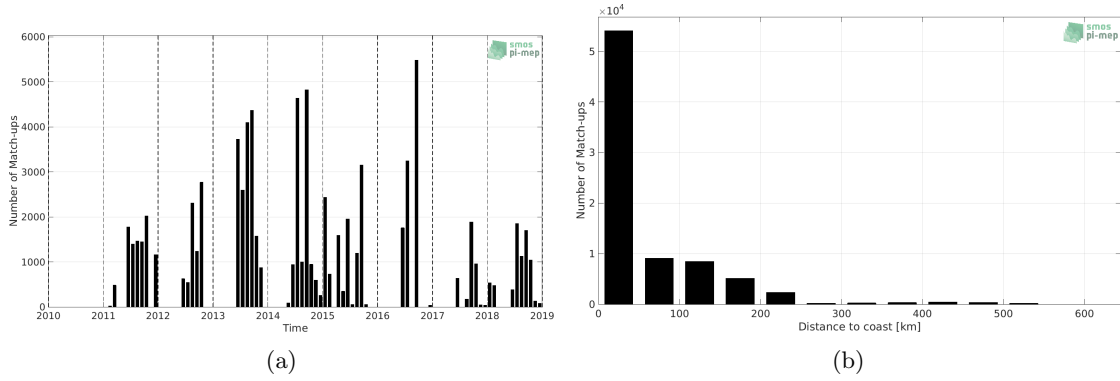
Figure 1: Number of match-ups between TSG (LEGOS-DM) and SMOS SSS L3 v2 - 9-Days (BEC) SSS as a function of time (a) and as function of the distance to coast (b) over the Arctic Ocean Pi-MEP region and for the full satellite product period.
