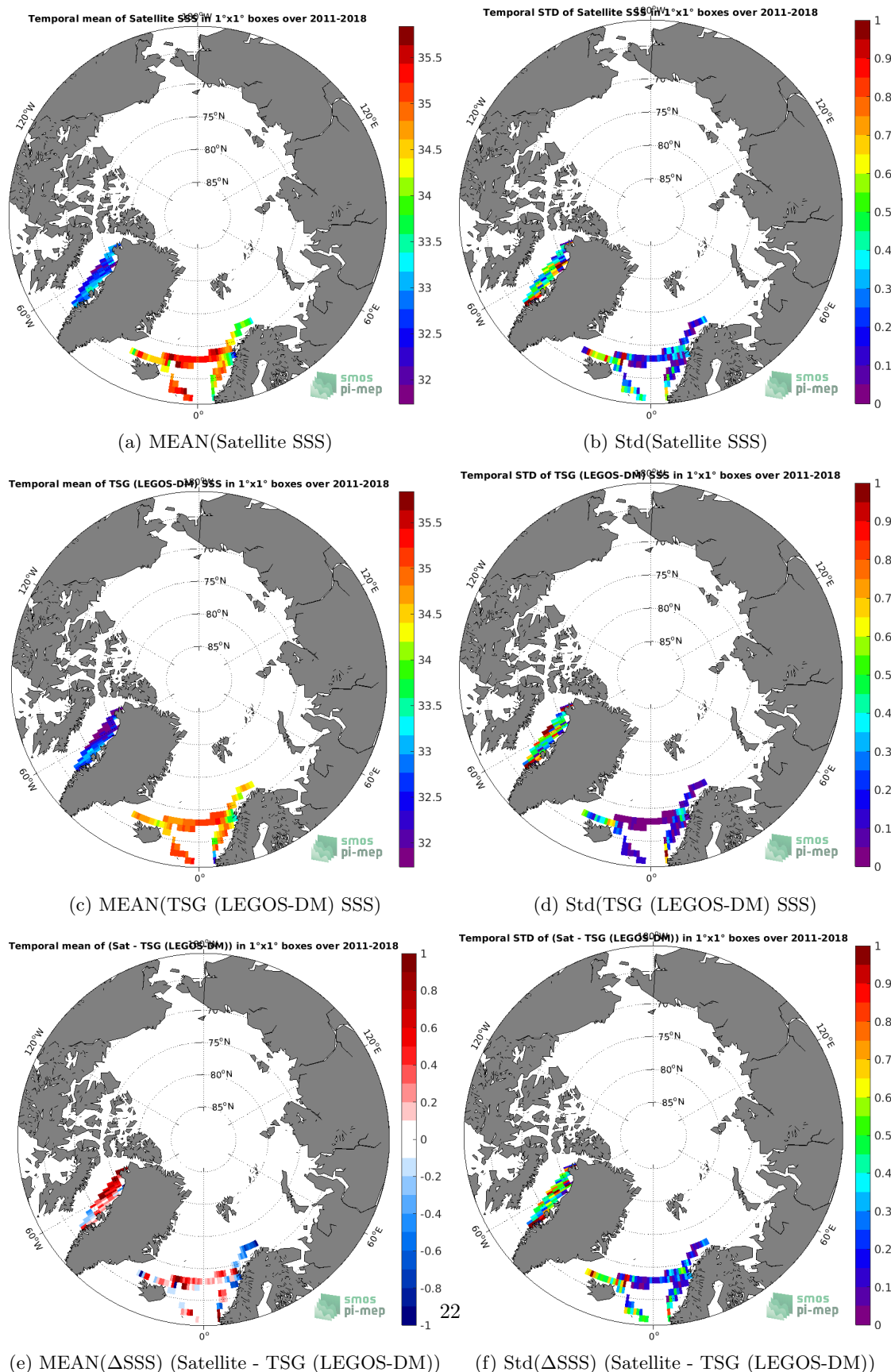
Figure 6: Temporal mean (left) and Std (right) of SSS from SMOS SSS L3 v2 - 9-Days (BEC) (top), TSG (LEGOS-DM) (middle), and of \Delta SSS (Satellite - TSG (LEGOS-DM)). Only match-up pairs are used to generate these maps.
