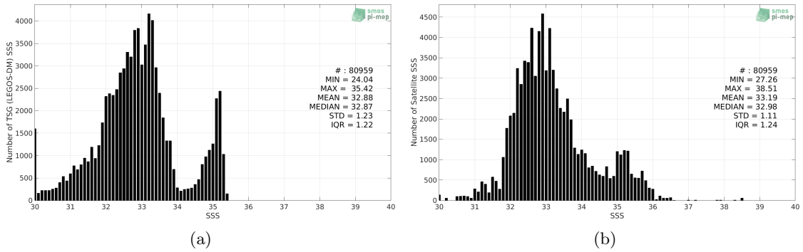
Figure 2: Histograms of SSS from TSG (LEGOS-DM) (a) and SMOS SSS L3 v2 - 9-Days (BEC) (b) considering all match-up pairs per bins of 0.1 over the Arctic Ocean Pi-MEP region and for the full satellite product period.
