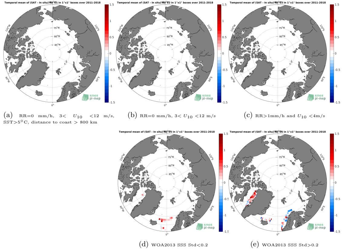
Figure 12: Temporal mean gridded over spatial boxes of size 1^{\circ}\times 1^{\circ} of \Delta\text{SSS} (SMOS L3 v2 - 9-Days (BEC) - TSG (LEGOS-DM)) for 5 different subdatasets corresponding to:RR=0 mm/h, 3 < U_{10} < 12 m/s, SST >5^{\circ}\text{C} , distance to coast > 800 km (a), RR=0 mm/h, 3 < U_{10} < 12 m/s (b), RR >1 mm/h and U_{10} < 4 m/s (c), WOA2013 SSS Std <0.2 (d), WOA2013 SSS Std >0.2 (e).
