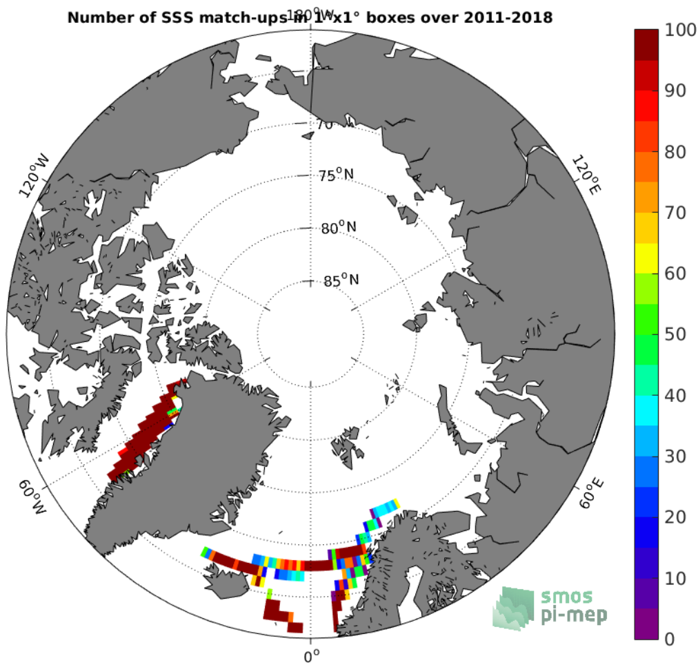
Figure 4: Number of SSS match-ups between TSG (LEGOS-DM) SSS and the SMOS L3 v2 - 9-Days (BEC) SSS product for the Arctic Ocean Pi-MEP region over 1°x1° boxes and for the full satellite product period.
