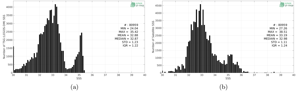
Figure 2: Histograms of SSS from TSG (LEGOS-DM) (a) and SMOS L3 v2 - 9-Days (BEC) (b) considering all match-up pairs per bins of 0.1 over the Arctic Ocean Pi-MEP region and for the full satellite product period.
