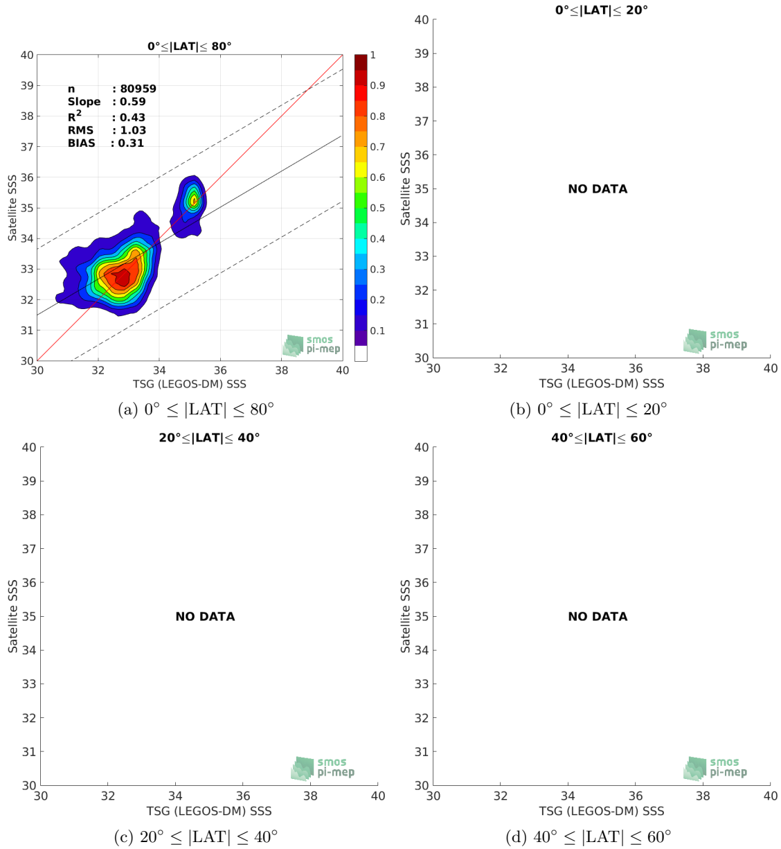
Figure 9: Contour maps of the concentration of SMOS L3 v2 - 9-Days (BEC) SSS (y-axis) versus TSG (LEGOS-DM) SSS (x-axis) at match-up pairs for different latitude bands. For each plot, the red line shows x=y . The black thin and dashed lines indicate a linear fit through the data cloud and the \pm 95\% confidence levels, respectively. The number match-up pairs n , the slope and R^2 coefficient of the linear fit, the root mean square (RMS) and the mean bias between satellite and in situ data are indicated for each latitude band in each plots.
