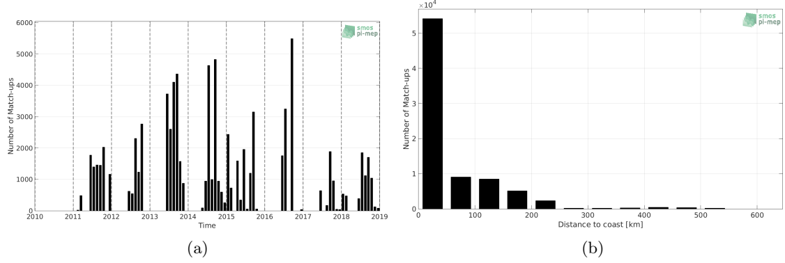
Figure 1: Number of match-ups between TSG (LEGOS-DM) and SMOS L3 v2 - 9-Days (BEC) SSS as a function of time (a) and as function of the distance to coast (b) over the Arctic Ocean Pi-MEP region and for the full satellite product period.
