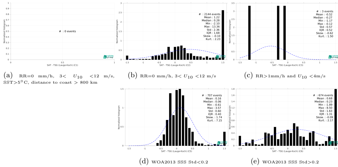
Figure 15: Normalized histogram of \Delta SSS (SMOS SSS L3 v2 - 9-Days (BEC) - TSG (Lauge-Koch)) for 5 different subdatasets corresponding to: RR=0 mm/h, 3 < U_{10} < 12 m/s, SST > 5°C, distance to coast > 800 km (a), RR=0 mm/h, 3 < U_{10} < 12 m/s (b), RR > 1mm/h and U_{10} < 4 m/s (c), WOA2013 SSS Std < 0.2 (d), WOA2013 SSS Std > 0.2 (e).
