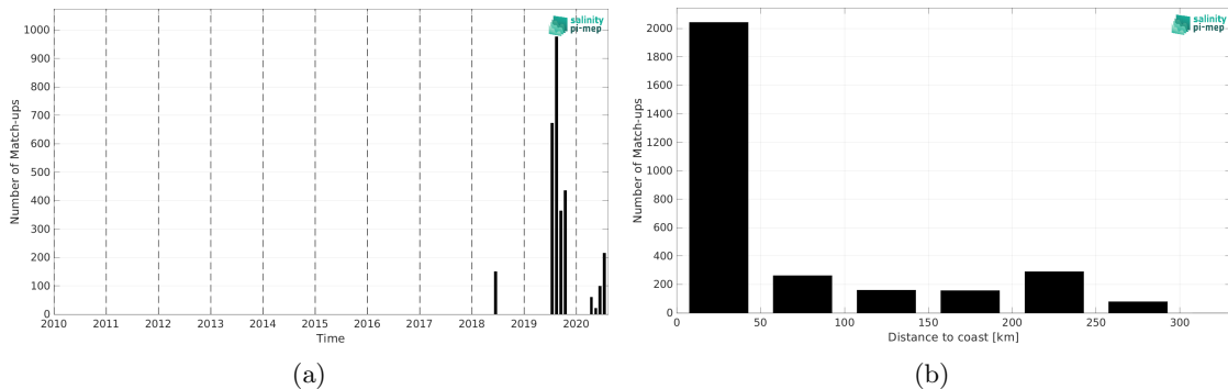
Figure 2: Number of match-ups between TSG (Lauge-Koch) and SMOS SSS L3 v2 - 9-Days (BEC) SSS as a function of time (a) and as function of the distance to coast (b) over the Arctic Ocean Pi-MEP region and for the full satellite product period.
