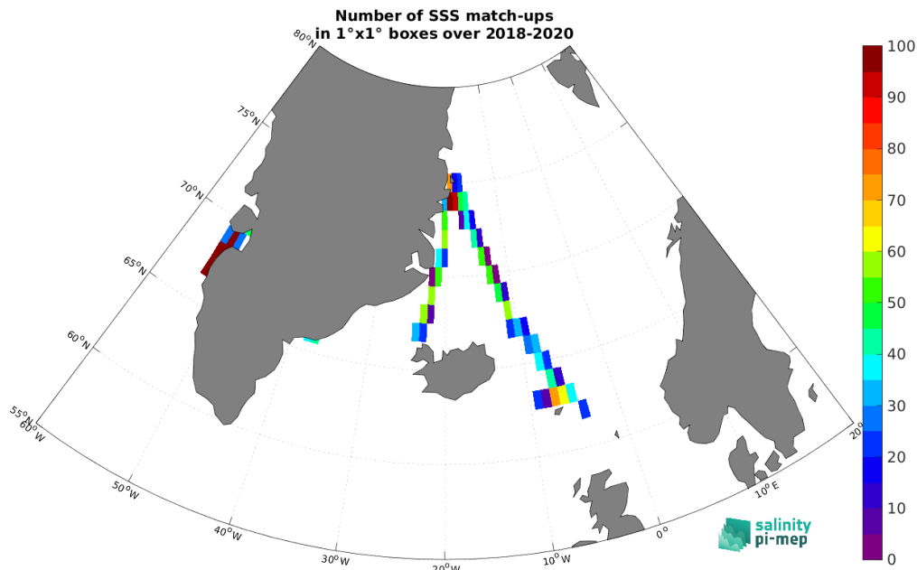
Figure 5: Number of SSS match-ups between TSG (Lauge-Koch) SSS and the SMOS SSS L3 v2 - 9-Days (BEC) SSS product for the Arctic Ocean Pi-MEP region over 1^\circ \times 1^\circ boxes and for the full satellite product period.
