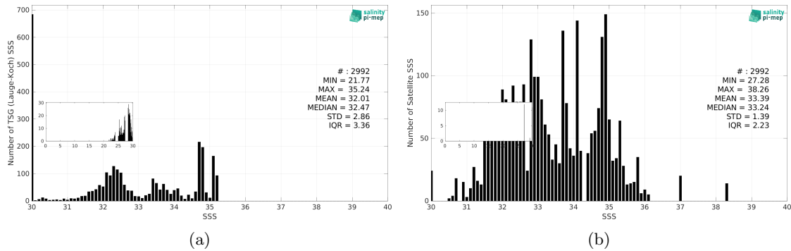
Figure 3: Histograms of SSS from TSG (Lauge-Koch) (a) and SMOS SSS L3 v2 - 9-Days (BEC) (b) considering all match-up pairs per bins of 0.1 over the Arctic Ocean Pi-MEP region and for the full satellite product period.
