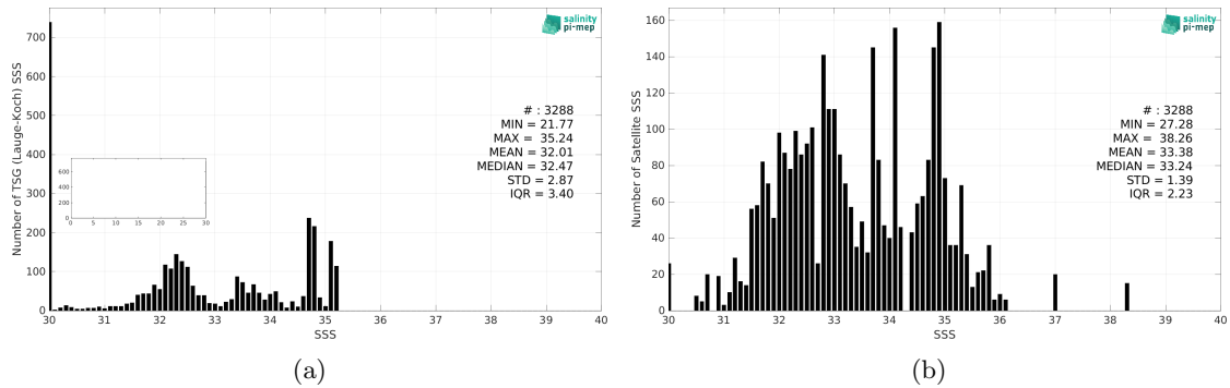
Figure 2: Histograms of SSS from TSG (Lauge-Koch) (a) and SMOS SSS L3 v2 - 9-Days (BEC) (b) considering all match-up pairs per bins of 0.1 over the Arctic Ocean Pi-MEP region and for the full satellite product period.
