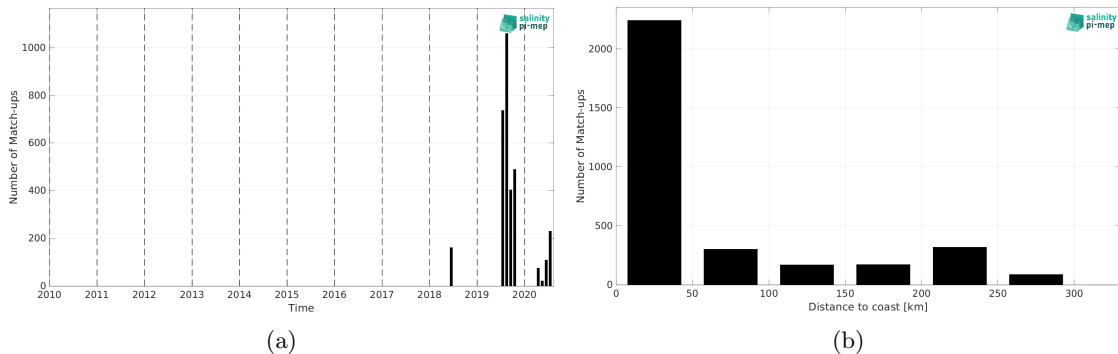
Figure 1: Number of match-ups between TSG (Lauge-Koch) and SMOS SSS L3 v2 - 9-Days (BEC) SSS as a function of time (a) and as function of the distance to coast (b) over the Arctic Ocean Pi-MEP region and for the full satellite product period.
