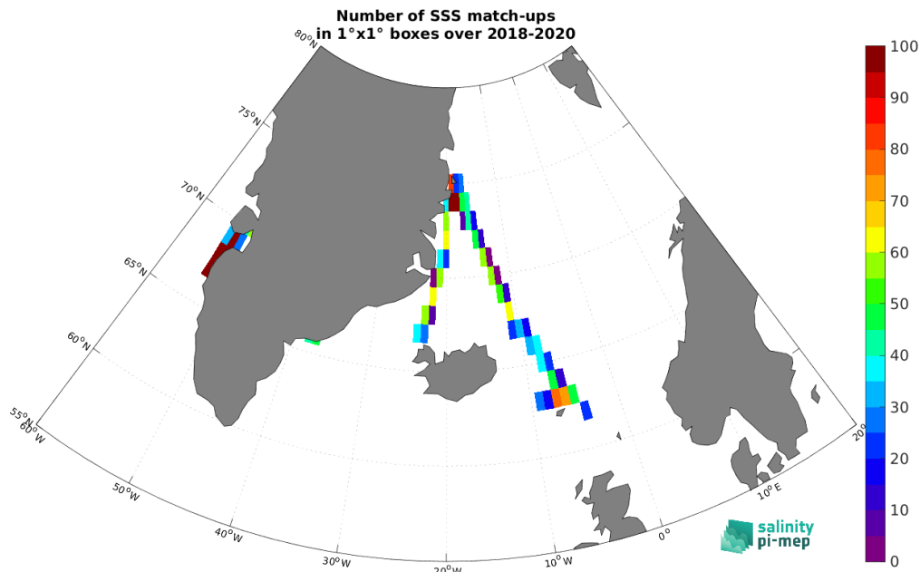
Figure 4: Number of SSS match-ups between TSG (Lauge-Koch) SSS and the SMOS SSS L3 v2 - 9-Days (BEC) SSS product for the Arctic Ocean Pi-MEP region over 1^\circ \times 1^\circ boxes and for the full satellite product period.
