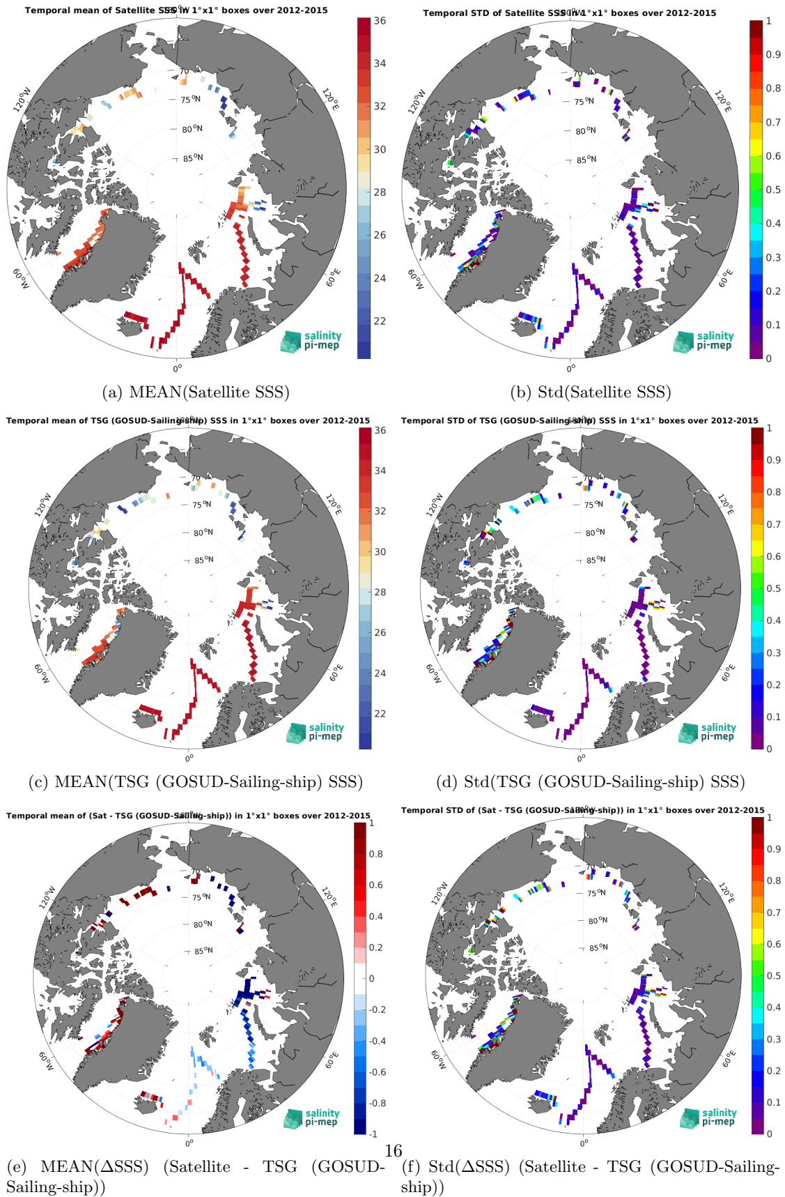
Figure 7: Temporal mean (left) and Std (right) of SSS from SMOS SSS L3 v2 - 9-Days (BEC) (top), TSG (GOSUD-Sailing-ship) (middle), and of \Delta SSS (Satellite - TSG (GOSUD-Sailing-ship)). Only match-up pairs are used to generate these maps.
