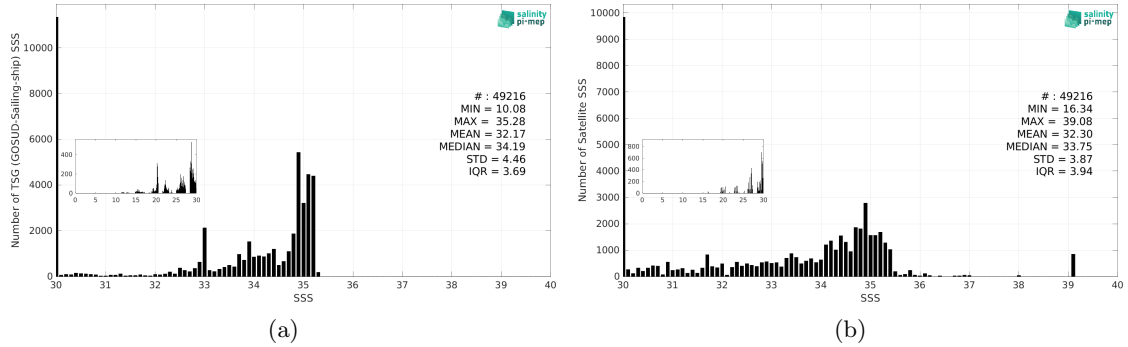
Figure 3: Histograms of SSS from TSG (GOSUD-Sailing-ship) (a) and SMOS SSS L3 v2 - 9-Days (BEC) (b) considering all match-up pairs per bins of 0.1 over the Arctic Ocean Pi-MEP region and for the full satellite product period.
