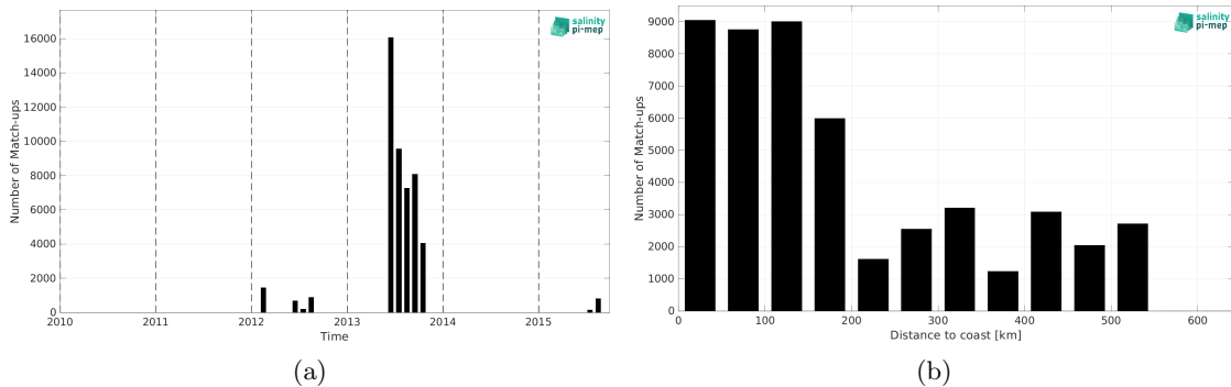
Figure 2: Number of match-ups between TSG (GOSUD-Sailing-ship) and SMOS SSS L3 v2 - 9-Days (BEC) SSS as a function of time (a) and as function of the distance to coast (b) over the Arctic Ocean Pi-MEP region and for the full satellite product period.
