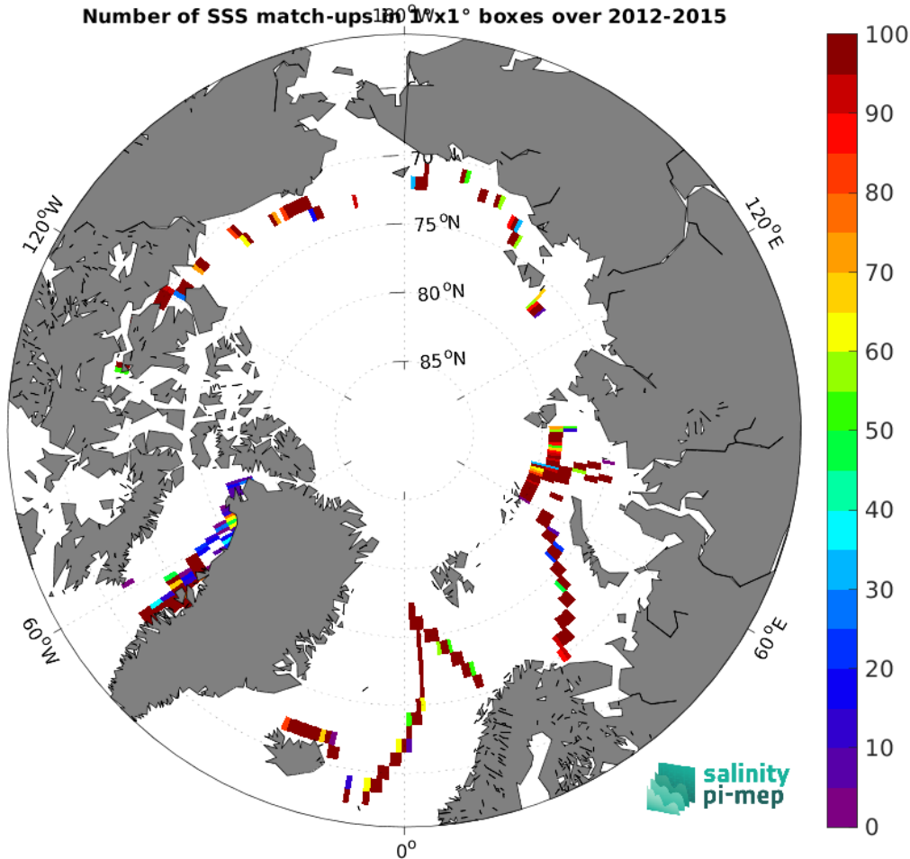
Figure 5: Number of SSS match-ups between TSG (GOSUD-Sailing-ship) SSS and the SMOS SSS L3 v2 - 9-Days (BEC) SSS product for the Arctic Ocean Pi-MEP region over 1^\circ \times 1^\circ boxes and for the full satellite product period.
