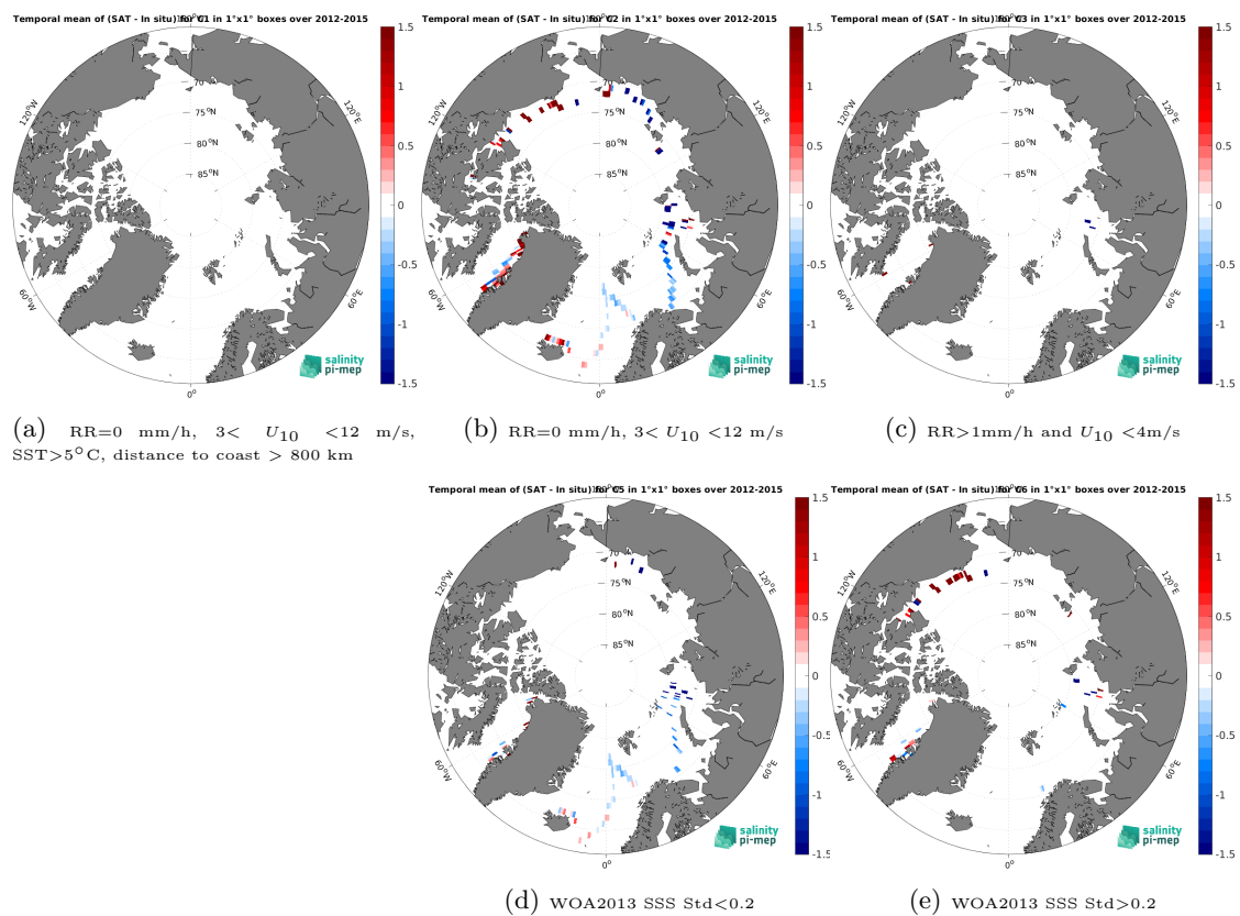
Figure 14: Temporal mean gridded over spatial boxes of size 1^\circ \times 1^\circ of \Delta\text{SSS} (SMOS SSS L3 v2 - 9-Days (BEC) - TSG (GOSUD-Sailing-ship)) for 5 different subdatasets corresponding to:RR=0 mm/h, 3 < U_{10} < 12 m/s, SST > 5^\circ\text{C} , distance to coast > 800 km (a), RR=0 mm/h, 3 < U_{10} < 12 m/s (b), RR > 1 mm/h and U_{10} < 4 m/s (c), WOA2013 SSS Std < 0.2 (d), WOA2013 SSS Std > 0.2 (e).
