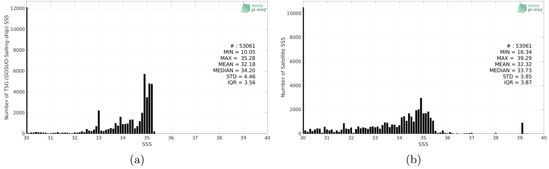
Figure 2: Histograms of SSS from TSG (GOSUD-Sailing-ship) (a) and SMOS SSS L3 v2 - 9-Days (BEC) (b) considering all match-up pairs per bins of 0.1 over the Arctic Ocean Pi-MEP region and for the full satellite product period.
