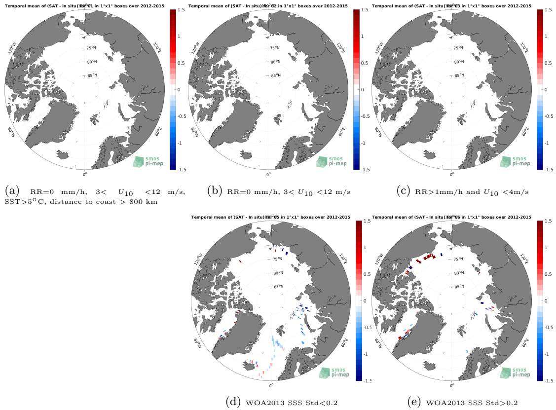
Figure 12: Temporal mean gridded over spatial boxes of size 1^\circ \times 1^\circ of \Delta SSS (SMOS SSS L3 v2 - 9-Days (BEC) - TSG (GOSUD-Sailing-ship)) for 5 different subdatasets corresponding to: RR=0 mm/h, 3 < U_{10} < 12 m/s, SST > 5°C, distance to coast > 800 km (a), RR=0 mm/h, 3 < U_{10} < 12 m/s (b), RR > 1mm/h and U_{10} < 4 m/s (c), WOA2013 SSS Std < 0.2 (d), WOA2013 SSS Std > 0.2 (e).
