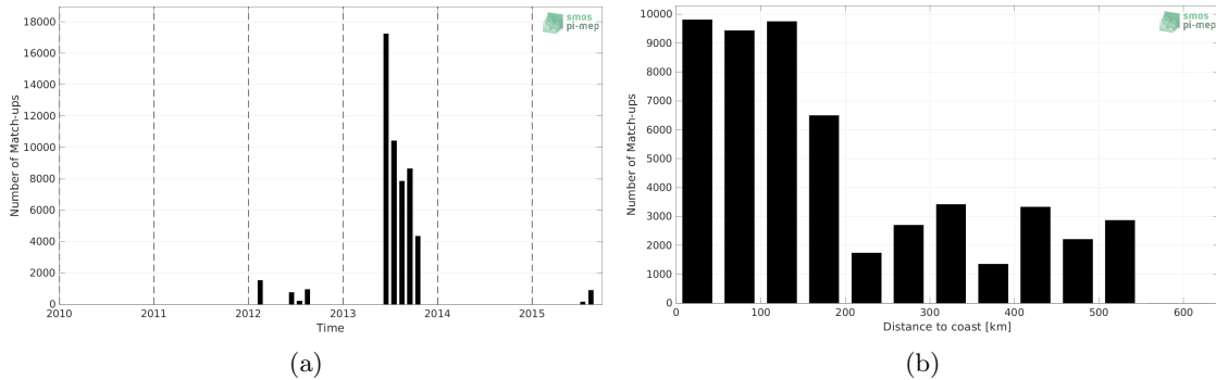
Figure 1: Number of match-ups between TSG (GOSUD-Sailing-ship) and SMOS SSS L3 v2 - 9-Days (BEC) SSS as a function of time (a) and as function of the distance to coast (b) over the Arctic Ocean Pi-MEP region and for the full satellite product period.
