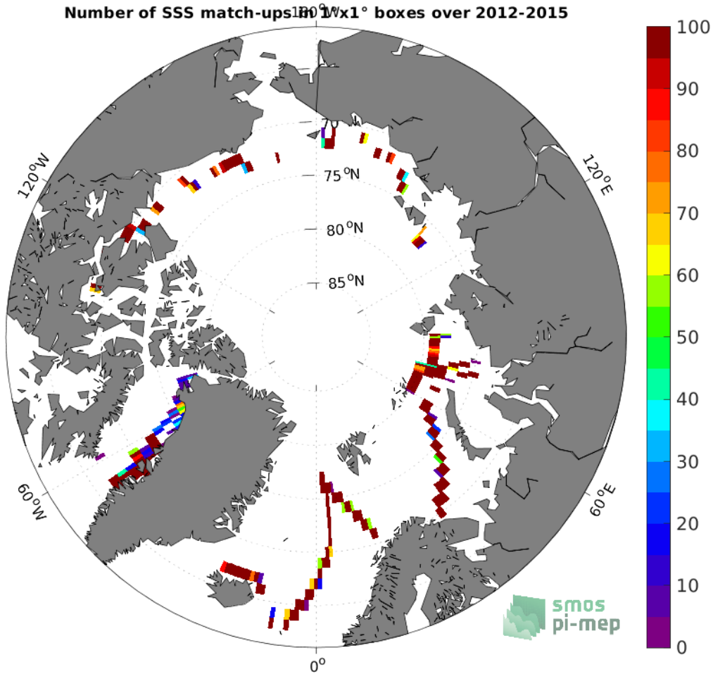
Figure 4: Number of SSS match-ups between TSG (GOSUD-Sailing-ship) SSS and the SMOS SSS L3 v2 - 9-Days (BEC) SSS product for the Arctic Ocean Pi-MEP region over 1^\circ \times 1^\circ boxes and for the full satellite product period.
