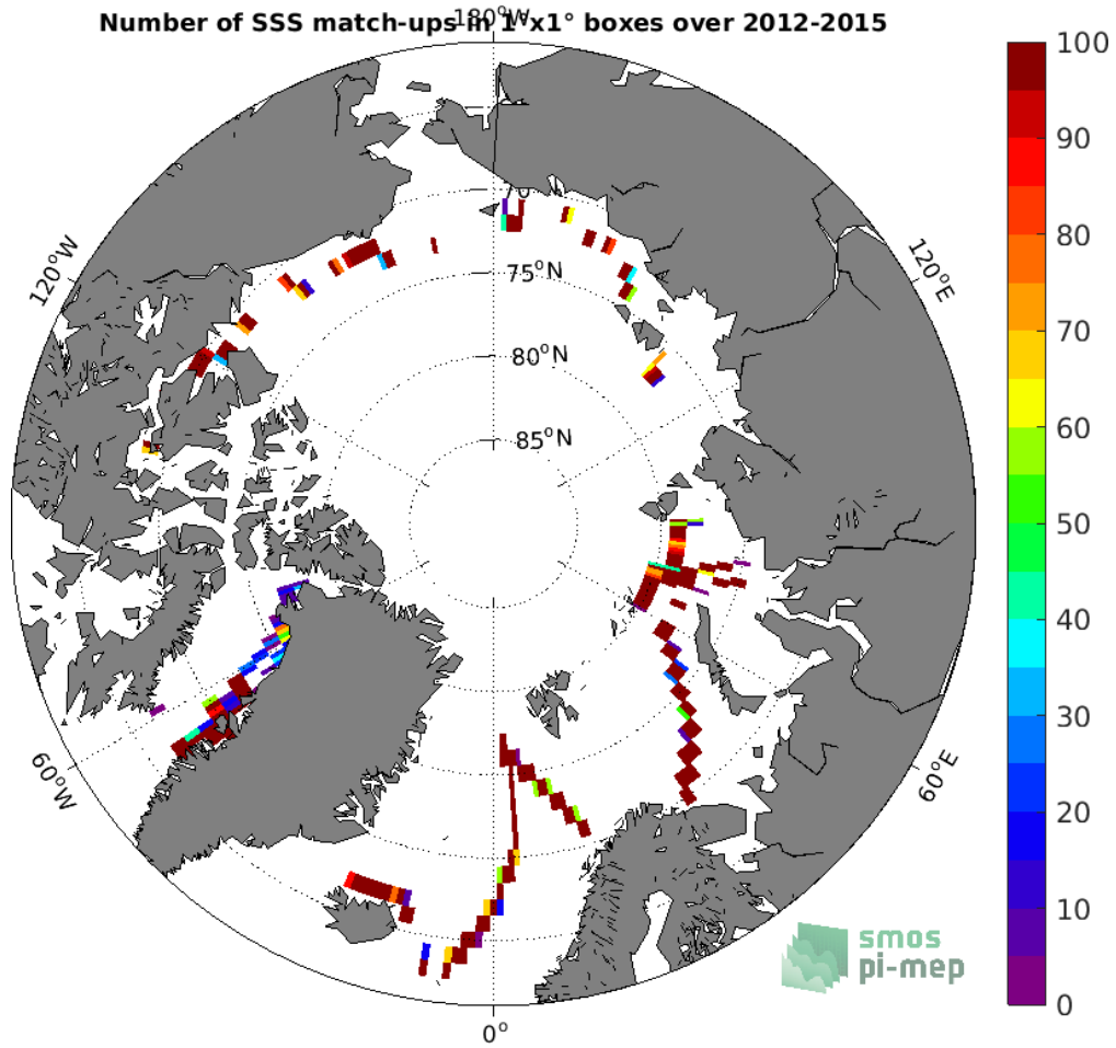
Figure 4: Number of SSS match-ups between TSG (GOSUD-Sailing-ship) SSS and the SMOS SSS L3 v2 - 9-Days (BEC) SSS product for the Arctic Ocean Pi-MEP region over 1°x1° boxes and for the full satellite product period.
