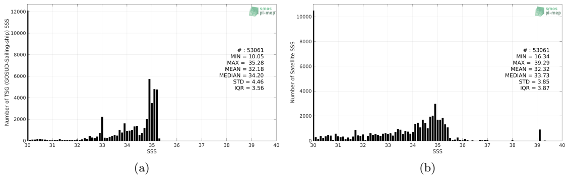
Figure 2: Histograms of SSS from TSG (GOSUD-Sailing-ship) (a) and SMOS SSS L3 v2 - 9-Days (BEC) (b) considering all match-up pairs per bins of 0.1 over the Arctic Ocean Pi-MEP region and for the full satellite product period.
