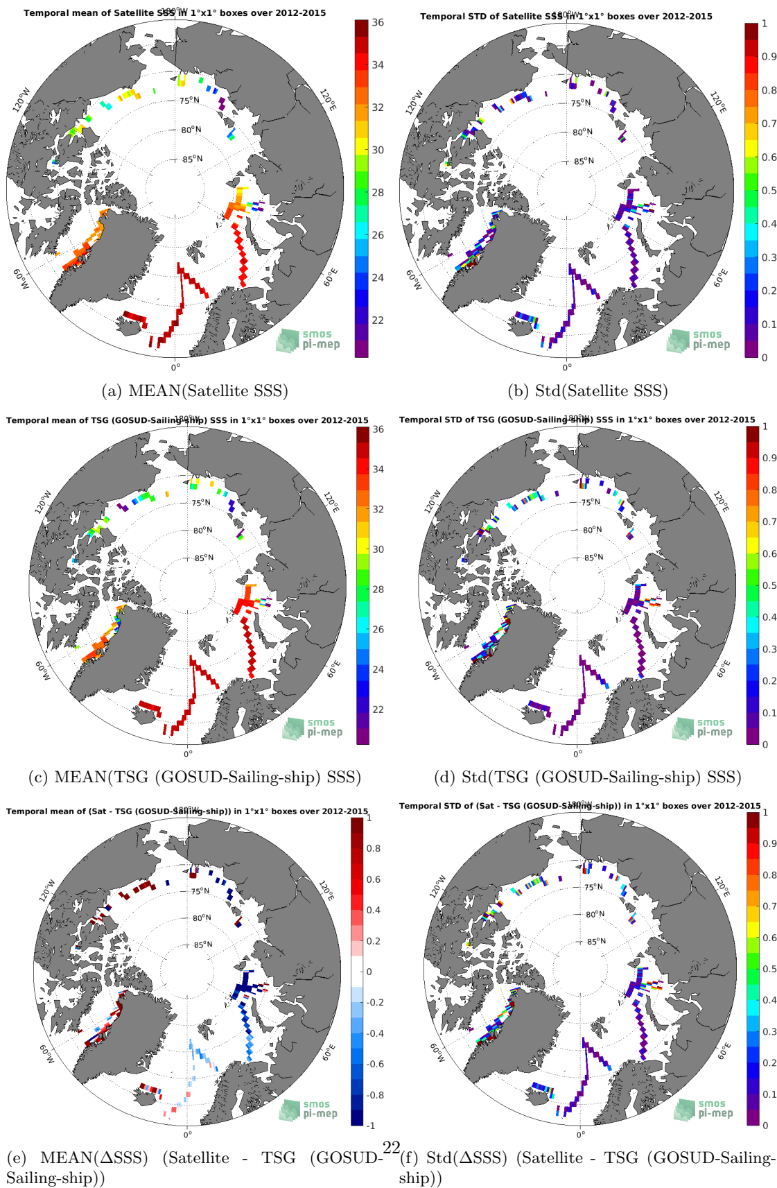
Figure 6: Temporal mean (left) and Std (right) of SSS from SMOS SSS L3 v2 - 9-Days (BEC) (top), TSG (GOSUD-Sailing-ship) (middle), and of \Delta SSS (Satellite - TSG (GOSUD-Sailing-ship)). Only match-up pairs are used to generate these maps.
