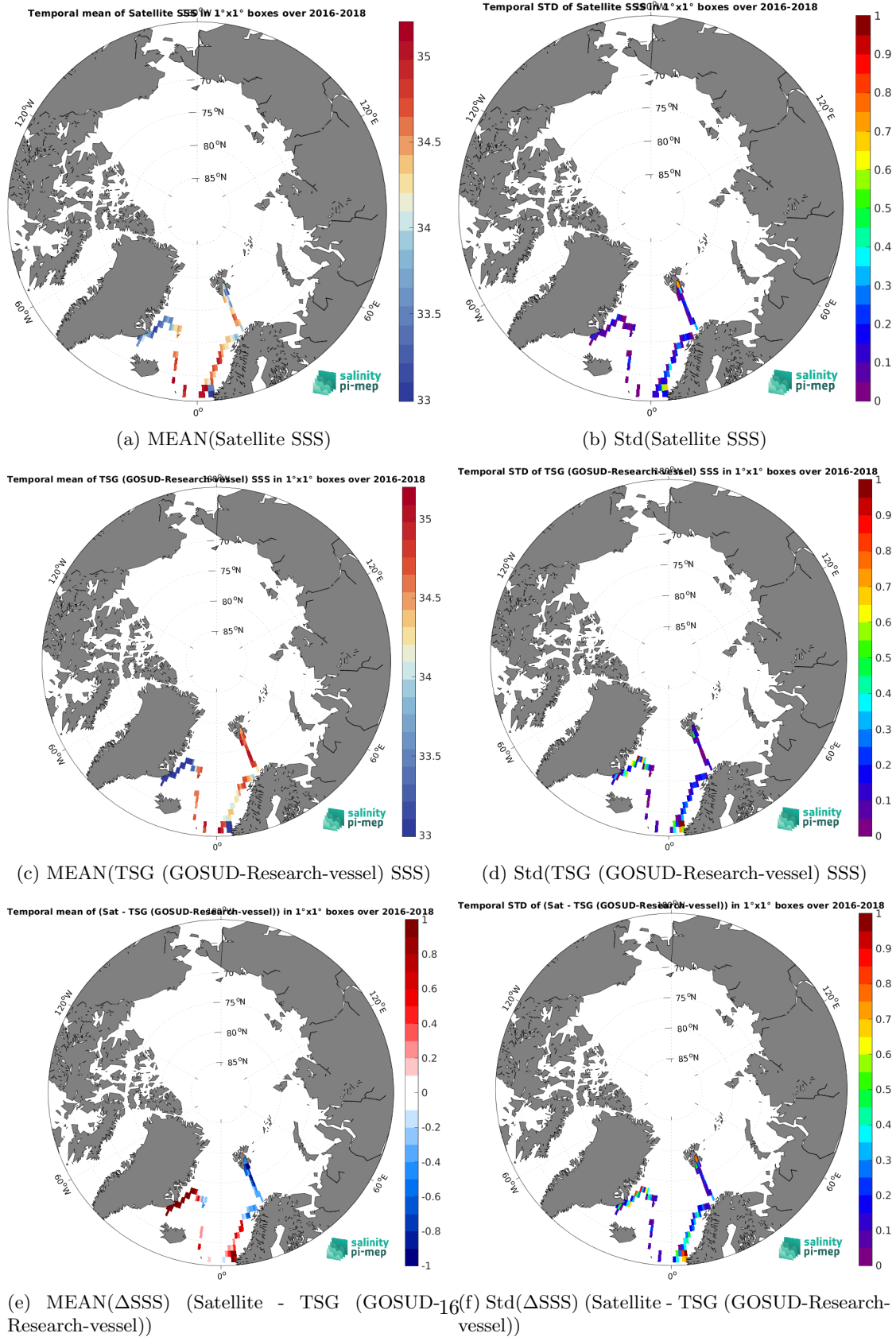
Figure 7: Temporal mean (left) and Std (right) of SSS from SMOS SSS L3 v2 - 9-Days (BEC) (top), TSG (GOSUD-Research-vessel) (middle), and of \Delta SSS (Satellite - TSG (GOSUD-Research-vessel)). Only match-up pairs are used to generate these maps.
