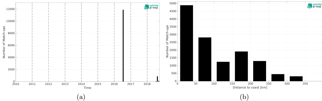
Figure 2: Number of match-ups between TSG (GOSUD-Research-vessel) and SMOS SSS L3 v2 - 9-Days (BEC) SSS as a function of time (a) and as function of the distance to coast (b) over the Arctic Ocean Pi-MEP region and for the full satellite product period.
