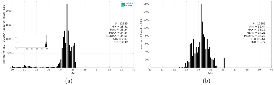
Figure 3: Histograms of SSS from TSG (GOSUD-Research-vessel) (a) and SMOS SSS L3 v2 - 9-Days (BEC) (b) considering all match-up pairs per bins of 0.1 over the Arctic Ocean Pi-MEP region and for the full satellite product period.
