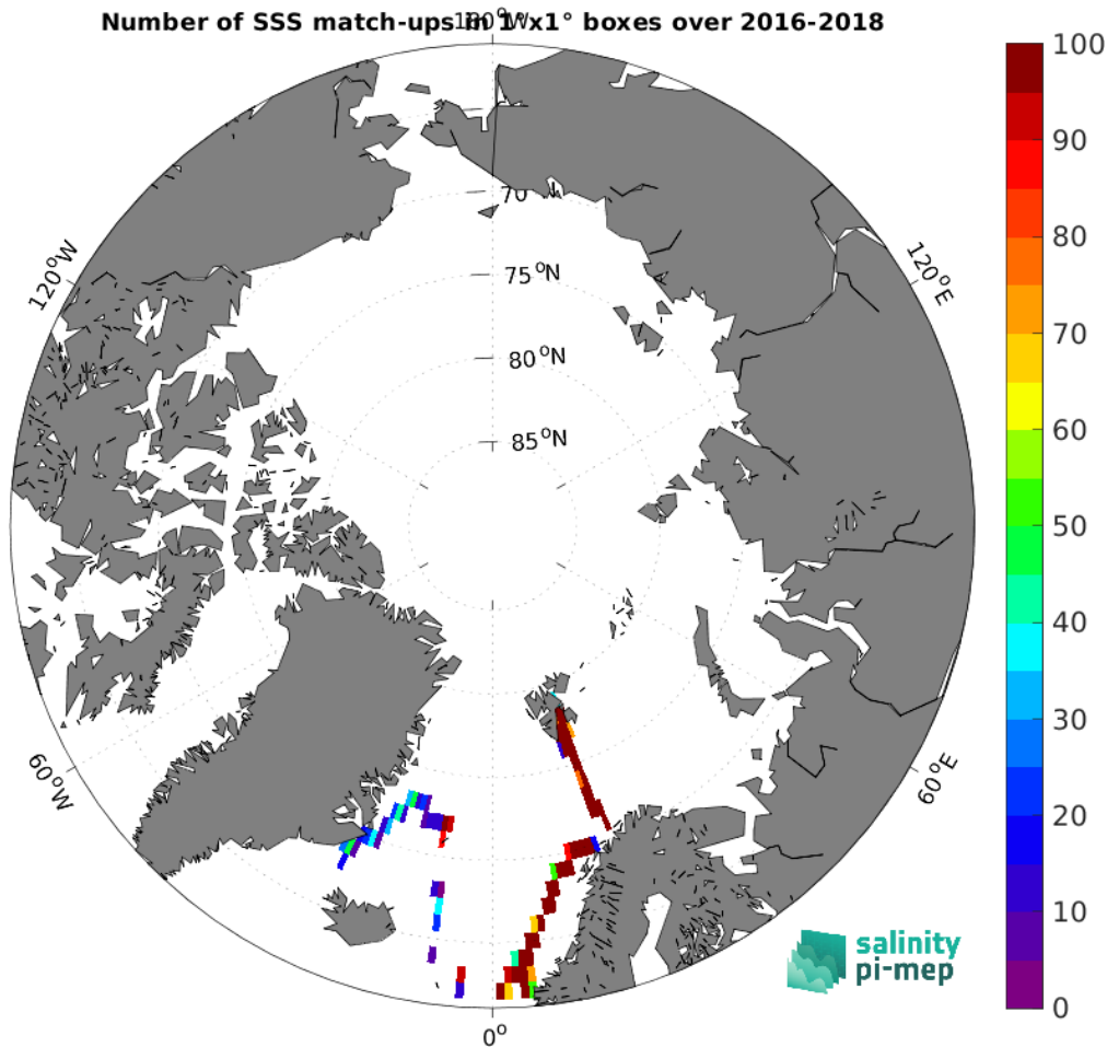
Figure 5: Number of SSS match-ups between TSG (GOSUD-Research-vessel) SSS and the SMOS SSS L3 v2 - 9-Days (BEC) SSS product for the Arctic Ocean Pi-MEP region over 1^\circ \times 1^\circ boxes and for the full satellite product period.
