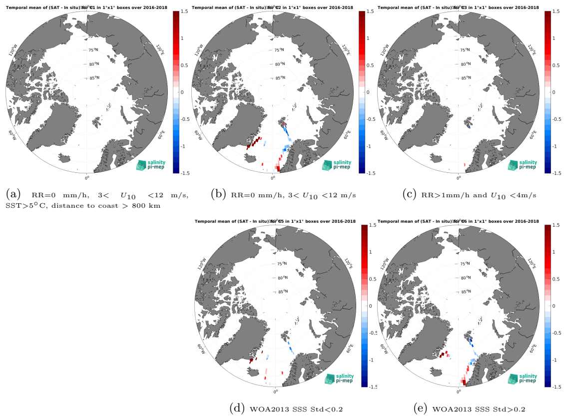
Figure 14: Temporal mean gridded over spatial boxes of size 1^\circ \times 1^\circ of \Delta SSS (SMOS SSS L3 v2 - 9-Days (BEC) - TSG (GOSUD-Research-vessel)) for 5 different subdatasets corresponding to: RR=0 mm/h, 3 < U_{10} < 12 m/s, SST > 5^\circ\text{C} , distance to coast > 800 km (a), RR=0 mm/h, 3 < U_{10} < 12 m/s (b), RR > 1 mm/h and U_{10} < 4 m/s (c), WOA2013 SSS Std < 0.2 (d), WOA2013 SSS Std > 0.2 (e).
