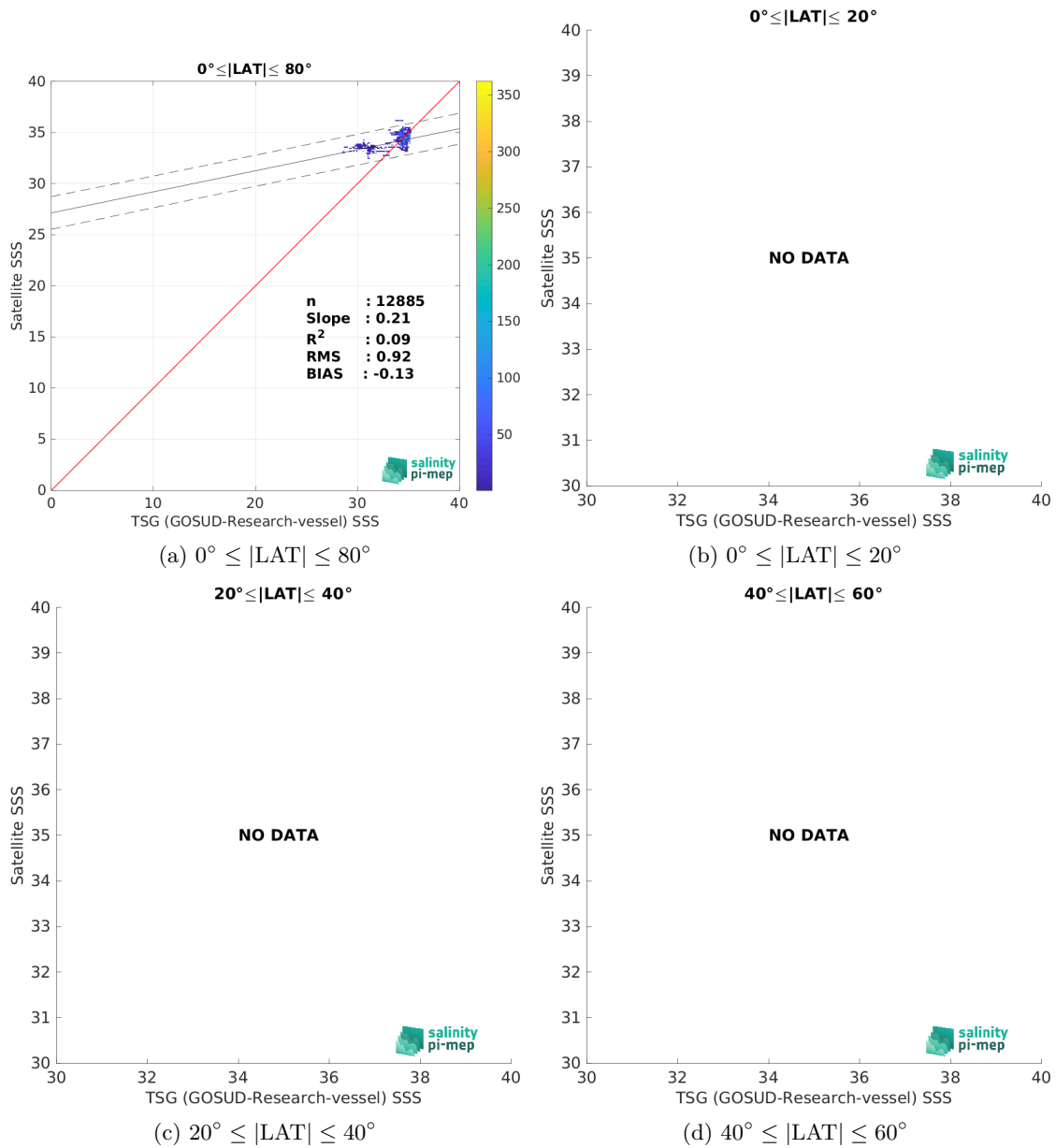
Figure 10: Contour maps of the concentration of SMOS SSS L3 v2 - 9-Days (BEC) SSS (y-axis) versus TSG (GOSUD-Research-vessel) SSS (x-axis) at match-up pairs for different latitude bands. For each plot, the red line shows x=y . The black thin and dashed lines indicate a linear fit through the data cloud and the \pm 95\% confidence levels, respectively. The number match-up pairs n , the slope and R^2 coefficient of the linear fit, the root mean square (RMS) and the mean bias between satellite and in situ data are indicated for each latitude band in each plots.
