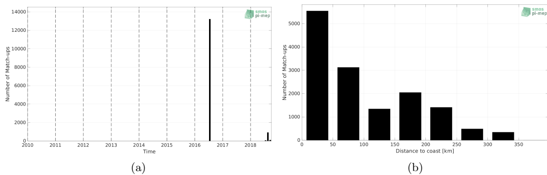
Figure 1: Number of match-ups between TSG (GOSUD-Research-vessel) and SMOS SSS L3 v2 - 9-Days (BEC) SSS as a function of time (a) and as function of the distance to coast (b) over the Arctic Ocean Pi-MEP region and for the full satellite product period.
