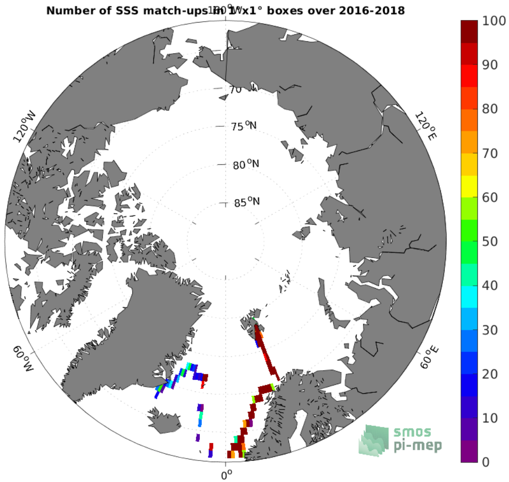
Figure 4: Number of SSS match-ups between TSG (GOSUD-Research-vessel) SSS and the SMOS SSS L3 v2 - 9-Days (BEC) SSS product for the Arctic Ocean Pi-MEP region over 1^\circ \times 1^\circ boxes and for the full satellite product period.
