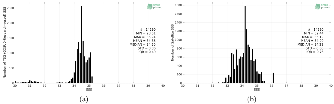
Figure 2: Histograms of SSS from TSG (GOSUD-Research-vessel) (a) and SMOS SSS L3 v2 - 9-Days (BEC) (b) considering all match-up pairs per bins of 0.1 over the Arctic Ocean Pi-MEP region and for the full satellite product period.
