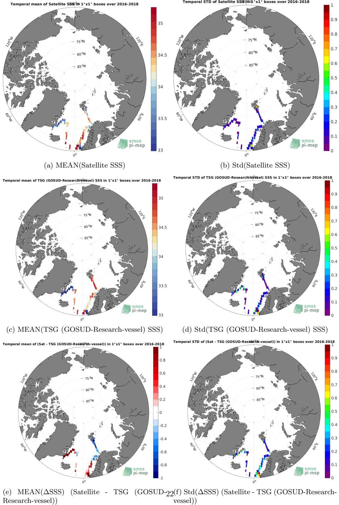
Figure 6: Temporal mean (left) and Std (right) of SSS from SMOS SSS L3 v2 - 9-Days (BEC) (top), TSG (GOSUD-Research-vessel) (middle), and of \Delta SSS (Satellite - TSG (GOSUD-Research-vessel)). Only match-up pairs are used to generate these maps.
