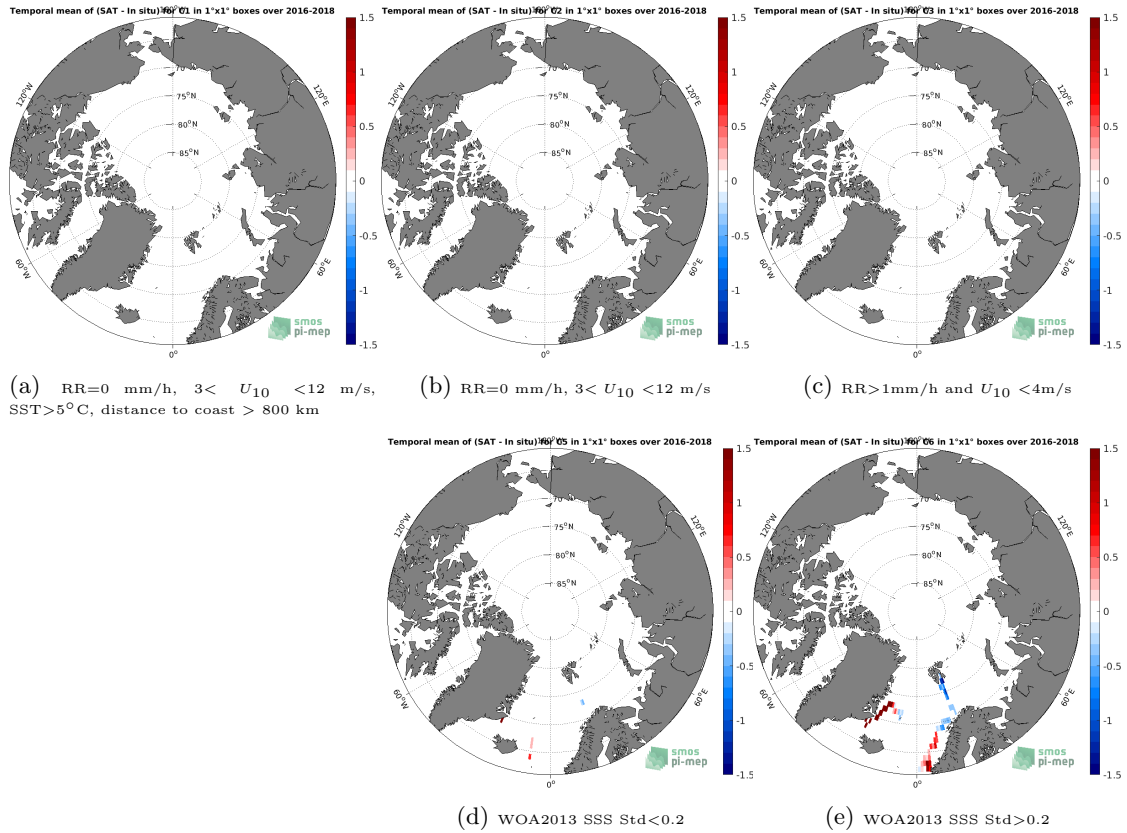
Figure 12: Temporal mean gridded over spatial boxes of size 1°x1° of \Delta SSS (SMOS SSS L3 v2 - 9-Days (BEC) - TSG (GOSUD-Research-vessel)) for 5 different subdatasets corresponding to:RR=0 mm/h, 3 < U_{10} < 12 m/s, SST>5°C, distance to coast > 800 km (a), RR=0 mm/h, 3 < U_{10} < 12 m/s (b), RR>1mm/h and U_{10} < 4 m/s (c), WOA2013 SSS Std<0.2 (d), WOA2013 SSS Std>0.2 (e).
