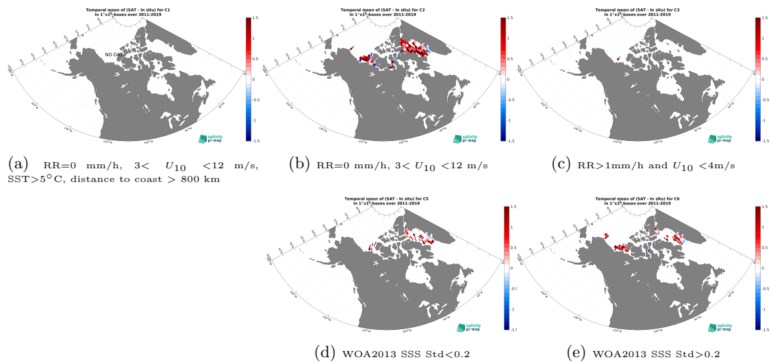
Figure 14: Temporal mean gridded over spatial boxes of size 1^\circ \times 1^\circ of \Delta SSS (SMOS SSS L3 v2 - 9-Days (BEC) - TSG (Amundsen)) for 5 different subdatasets corresponding to: RR=0 mm/h, 3 < U_{10} < 12 m/s, SST > 5°C, distance to coast > 800 km (a), RR=0 mm/h, 3 < U_{10} < 12 m/s (b), RR > 1mm/h and U_{10} < 4 m/s (c), WOA2013 SSS Std < 0.2 (d), WOA2013 SSS Std > 0.2 (e).
