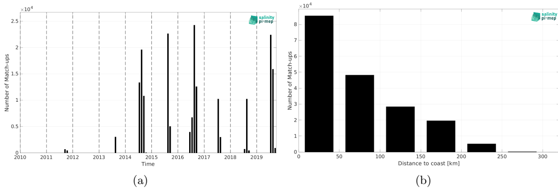
Figure 1: Number of match-ups between TSG (Amundsen) and SMOS SSS L3 v2 - 9-Days (BEC) SSS as a function of time (a) and as function of the distance to coast (b) over the Arctic Ocean Pi-MEP region and for the full satellite product period.
