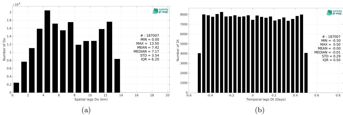
Figure 5: Histograms of the spatial (a) and temporal (b) lags between the location/time of the TSG (Amundsen) measurement and the date of the corresponding SMOS SSS L3 v2 - 9-Days (BEC) SSS pixel.
