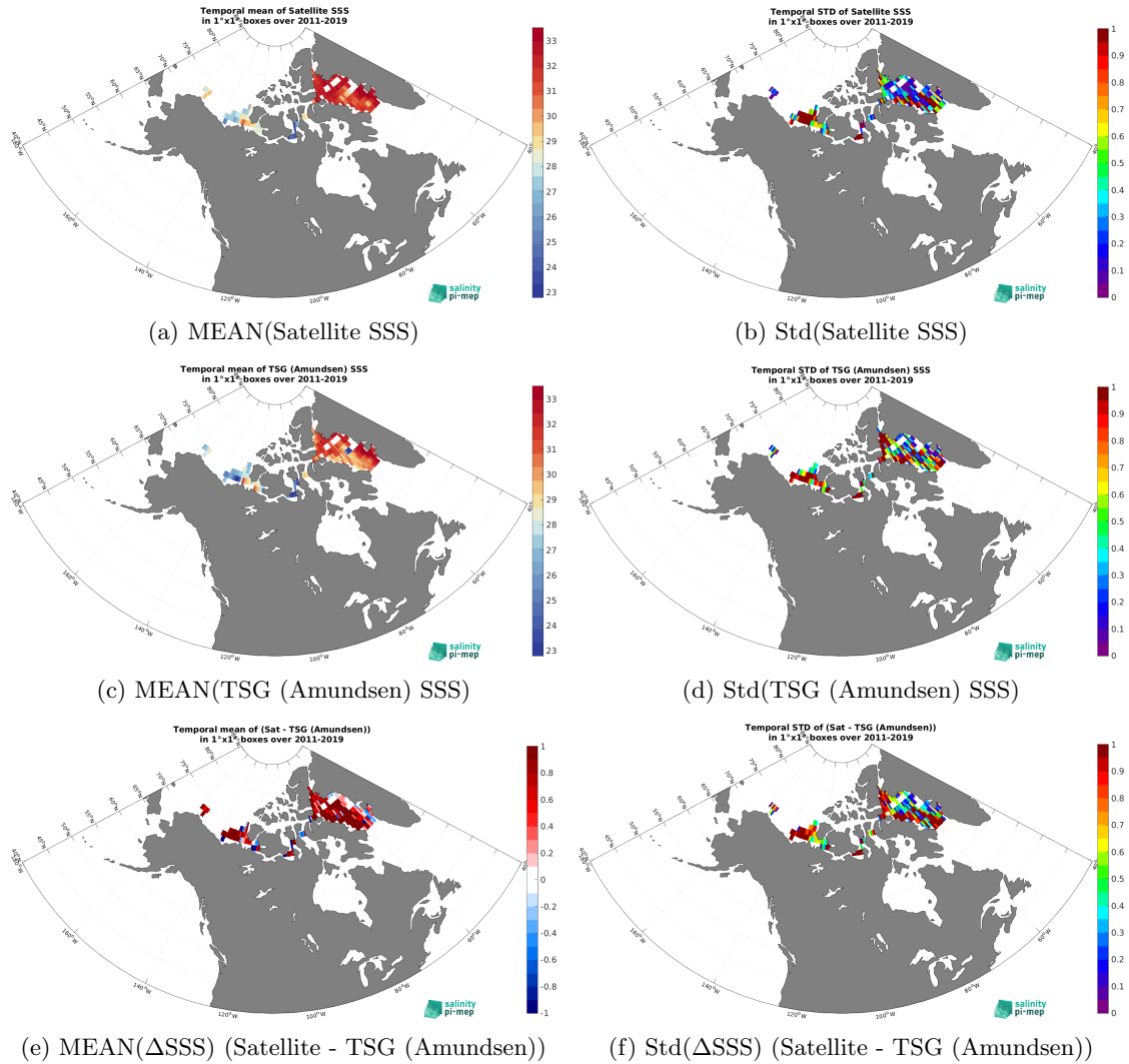
Figure 6: Temporal mean (left) and Std (right) of SSS from SMOS SSS L3 v2 - 9-Days (BEC) (top), TSG (Amundsen) (middle), and of \Delta SSS (Satellite - TSG (Amundsen)). Only match-up pairs are used to generate these maps.
