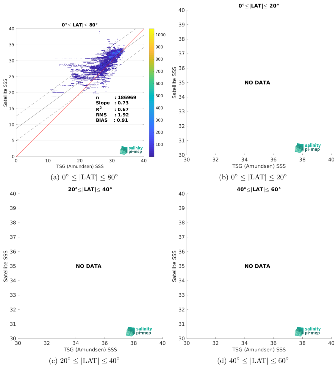
Figure 9: Contour maps of the concentration of SMOS SSS L3 v2 - 9-Days (BEC) SSS (y-axis) versus TSG (Amundsen) SSS (x-axis) at match-up pairs for different latitude bands. For each plot, the red line shows x=y . The black thin and dashed lines indicate a linear fit through the data cloud and the \pm 95\% confidence levels, respectively. The number match-up pairs n , the slope and R^2 coefficient of the linear fit, the root mean square (RMS) and the mean bias between satellite and in situ data are indicated for each latitude band in each plots.
