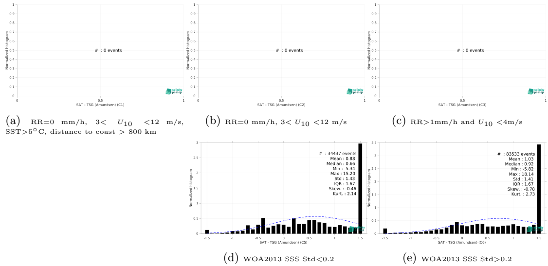
Figure 13: Normalized histogram of \Delta SSS (SMOS SSS L3 v2 - 9-Days (BEC) - TSG (Amundsen)) for 5 different subdatasets corresponding to: RR=0 mm/h, 3 < U_{10} < 12 m/s, SST>5°C, distance to coast > 800 km (a), RR=0 mm/h, 3 < U_{10} < 12 m/s (b), RR>1mm/h and U_{10} < 4 m/s (c), WOA2013 SSS Std<0.2 (d), WOA2013 SSS Std>0.2 (e).
