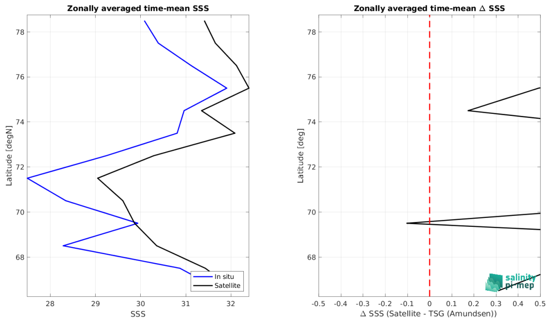
Figure 8: Left panel: Zonal mean SSS from SMOS SSS L3 v2 - 9-Days (BEC) satellite product (black) and from TSG (Amundsen) (blue). Right panel: Zonal mean of \Delta SSS (Satellite - TSG (Amundsen)) for all the collected Pi-MEP match-up pairs estimated over the full satellite product period.
