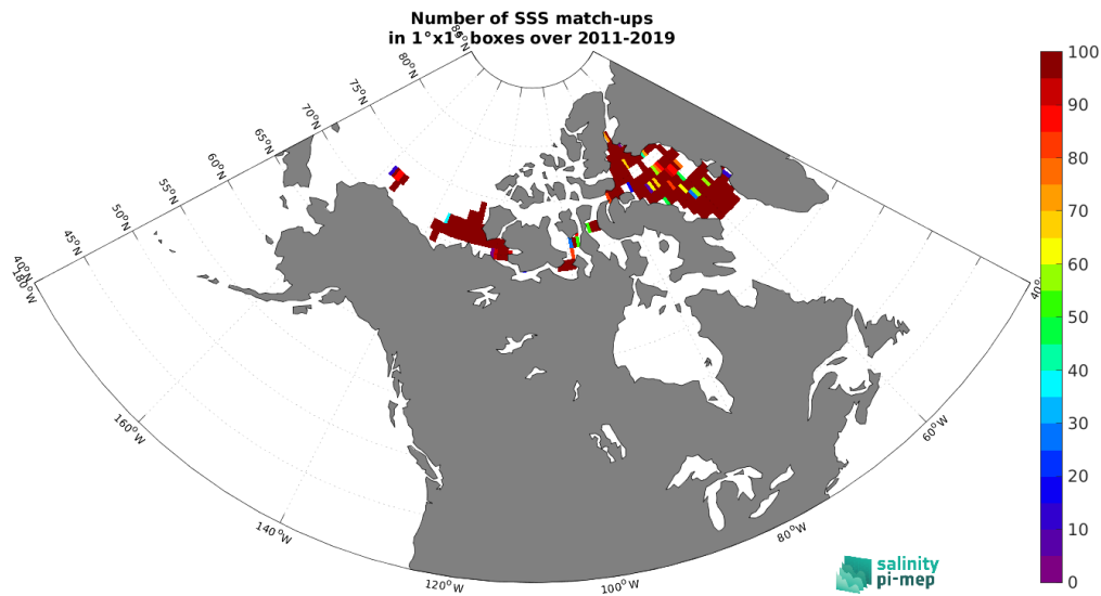
Figure 4: Number of SSS match-ups between TSG (Amundsen) SSS and the SMOS SSS L3 v2 - 9-Days (BEC) SSS product for the Arctic Ocean Pi-MEP region over 1^\circ \times 1^\circ boxes and for the full satellite product period.
