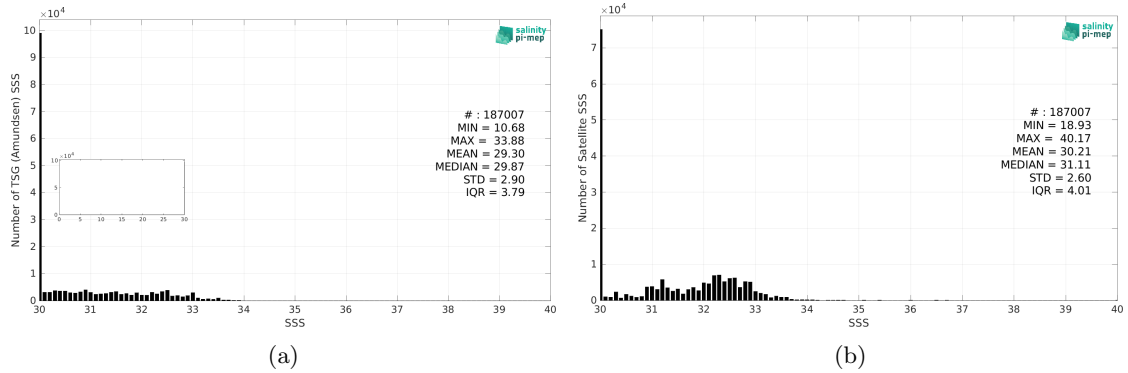
Figure 2: Histograms of SSS from TSG (Amundsen) (a) and SMOS SSS L3 v2 - 9-Days (BEC) (b) considering all match-up pairs per bins of 0.1 over the Arctic Ocean Pi-MEP region and for the full satellite product period.
