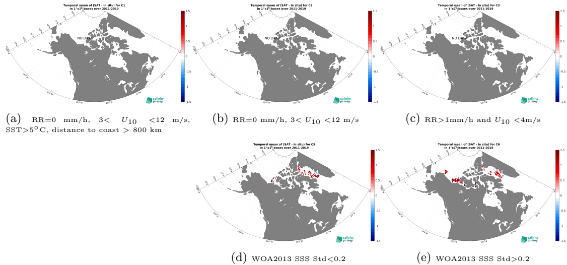
Figure 12: Temporal mean gridded over spatial boxes of size 1^{\circ}\times 1^{\circ} of \Delta\text{SSS} (SMOS SSS L3 v2 - 9-Days (BEC) - TSG (Amundsen)) for 5 different subdatasets corresponding to:RR=0 mm/h, 3 < U_{10} < 12 m/s, SST > 5^{\circ}\text{C} , distance to coast > 800 km (a), RR=0 mm/h, 3 < U_{10} < 12 m/s (b), RR > 1 mm/h and U_{10} < 4 m/s (c), WOA2013 SSS Std < 0.2 (d), WOA2013 SSS Std > 0.2 (e).
