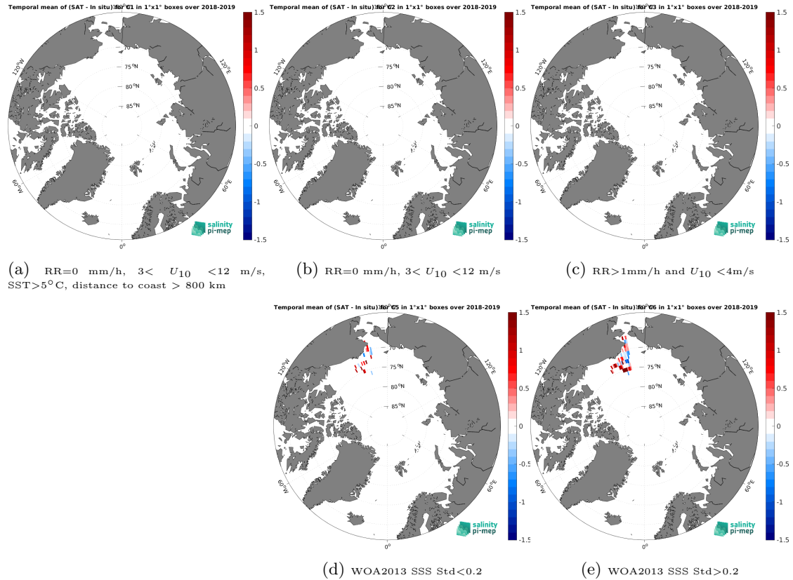
Figure 12: Temporal mean gridded over spatial boxes of size 1^{\circ}\times 1^{\circ} of \Delta\text{SSS} (SMOS SSS L3 v2 - 9-Days (BEC) - Sailability) for 5 different subdatasets corresponding to:RR=0 mm/h, 3 < U_{10} < 12 m/s, SST > 5^{\circ}\text{C} , distance to coast > 800 km (a), RR=0 mm/h, 3 < U_{10} < 12 m/s (b), RR > 1 mm/h and U_{10} < 4 m/s (c), WOA2013 SSS Std < 0.2 (d), WOA2013 SSS Std > 0.2 (e).
