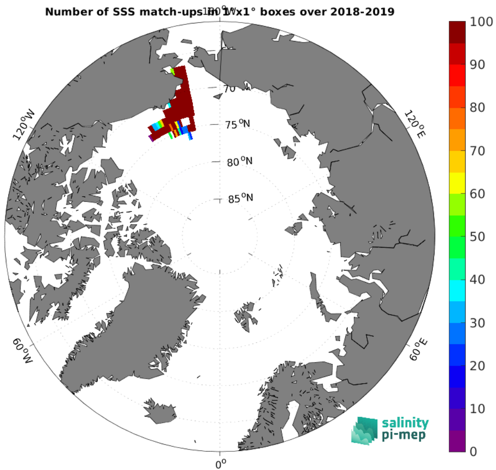
Figure 4: Number of SSS match-ups between Saildrone SSS and the SMOS SSS L3 v2 - 9-Days (BEC) SSS product for the Arctic Ocean Pi-MEP region over 1^\circ \times 1^\circ boxes and for the full satellite product period.
