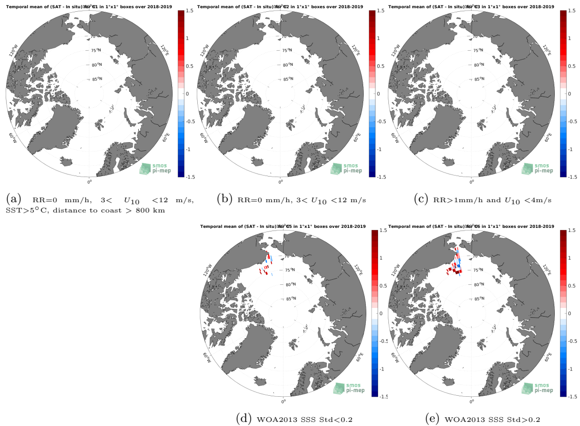
Figure 12: Temporal mean gridded over spatial boxes of size 1^{\circ}\times 1^{\circ} of \Delta\text{SSS} (SMOS SSS L3 v2 - 9-Days (BEC) - Sailydrone) for 5 different subdatasets corresponding to:RR=0 mm/h, 3 < U_{10} < 12 m/s, SST >5^{\circ}\text{C} , distance to coast > 800 km (a), RR=0 mm/h, 3 < U_{10} < 12 m/s (b), RR >1 mm/h and U_{10} < 4 m/s (c), WOA2013 SSS Std <0.2 (d), WOA2013 SSS Std >0.2 (e).
