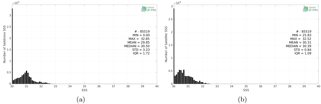
Figure 2: Histograms of SSS from Sairdrone (a) and SMOS SSS L3 v2 - 9-Days (BEC) (b) considering all match-up pairs per bins of 0.1 over the Arctic Ocean Pi-MEP region and for the full satellite product period.
