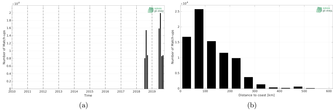
Figure 1: Number of match-ups between Saildrone and SMOS SSS L3 v2 - 9-Days (BEC) SSS as a function of time (a) and as function of the distance to coast (b) over the Arctic Ocean Pi-MEP region and for the full satellite product period.
