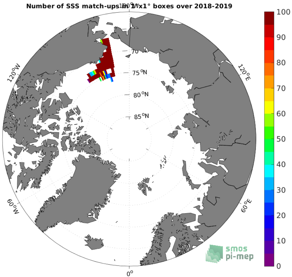
Figure 4: Number of SSS match-ups between Saildrone SSS and the SMOS SSS L3 v2 - 9-Days (BEC) SSS product for the Arctic Ocean Pi-MEP region over 1^{\circ} \times 1^{\circ} boxes and for the full satellite product period.
