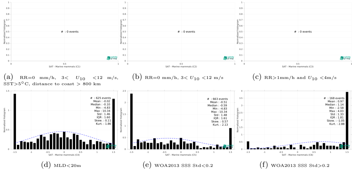
Figure 13: Normalized histogram of \Delta\text{SSS} (SMOS SSS L3 v2 - 9-Days (BEC) - Marine mammals) for 6 different subdatasets corresponding to: RR=0 mm/h, 3 < U_{10} < 12 m/s, SST > 5^\circ\text{C} , distance to coast > 800 km (a), RR=0 mm/h, 3 < U_{10} < 12 m/s (b), RR > 1\text{mm/h} and U_{10} < 4\text{m/s} (c), MLD < 20\text{m} (d), WOA2013 SSS Std < 0.2 (e), WOA2013 SSS Std > 0.2 (f).
