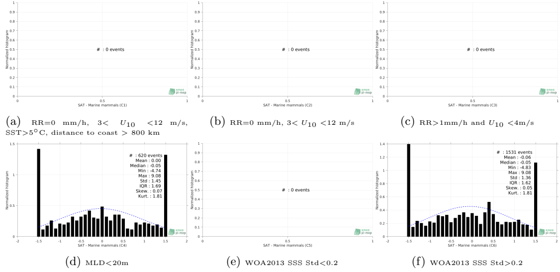
Figure 13: Normalized histogram of \Delta\text{SSS} (SMOS SSS L3 v2 - 9-Days (BEC) - Marine mammals) for 6 different subdatasets corresponding to: RR=0 mm/h, 3 < U_{10} < 12 m/s, SST > 5^{\circ}\text{C} , distance to coast > 800 km (a), RR=0 mm/h, 3 < U_{10} < 12 m/s (b), RR > 1\text{mm/h} and U_{10} < 4\text{m/s} (c), MLD < 20\text{m} (d), WOA2013 SSS Std < 0.2 (e), WOA2013 SSS Std > 0.2 (f).
