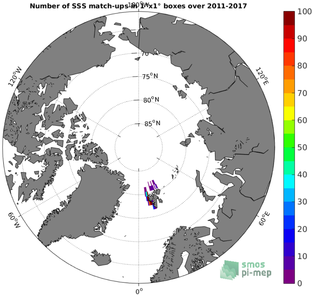
Figure 4: Number of SSS match-ups between Marine mammals SSS and the SMOS SSS L3 v2 - 9-Days (BEC) SSS product for the Arctic Ocean Pi-MEP region over 1^\circ \times 1^\circ boxes and for the full satellite product period.
