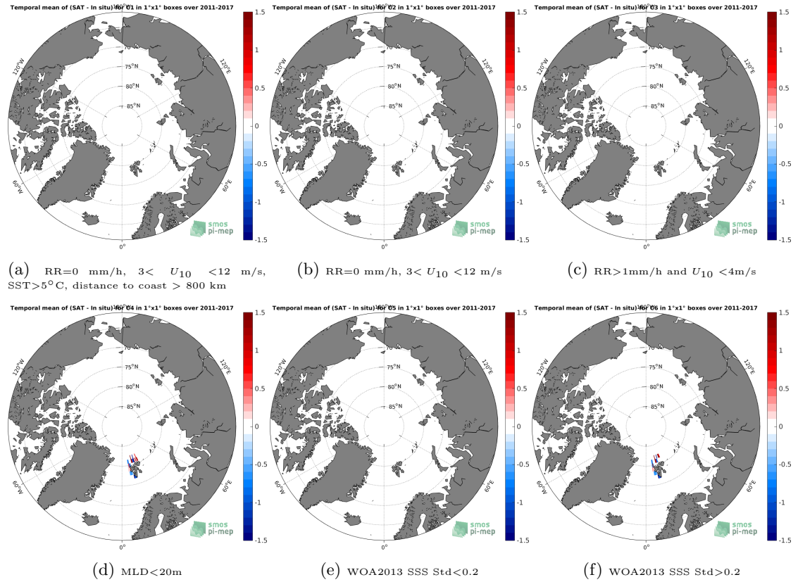
Figure 12: Temporal mean gridded over spatial boxes of size 1^{\circ} \times 1^{\circ} of \Delta\text{SSS} (SMOS SSS L3 v2 - 9-Days (BEC) - Marine mammals) for 6 different subdatasets corresponding to:RR=0 mm/h, 3 < U_{10} < 12 m/s, SST >5^{\circ}\text{C} , distance to coast > 800 km (a), RR=0 mm/h, 3 < U_{10} < 12 m/s (b), RR >1 mm/h and U_{10} < 4 m/s (c),MLD <20 m (d),WOA2013 SSS Std <0.2 (e),WOA2013 SSS Std >0.2 (f).
