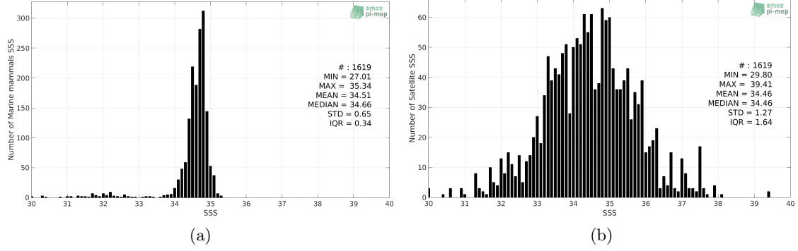
Figure 2: Histograms of SSS from Marine mammals (a) and SMOS SSS L3 v2 - 9-Days (BEC) (b) considering all match-up pairs per bins of 0.1 over the Arctic Ocean Pi-MEP region and for the full satellite product period.
