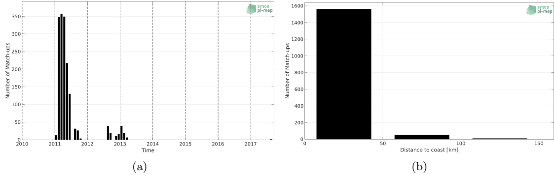
Figure 1: Number of match-ups between Marine mammals and SMOS SSS L3 v2 - 9-Days (BEC) SSS as a function of time (a) and as function of the distance to coast (b) over the Arctic Ocean Pi-MEP region and for the full satellite product period.
