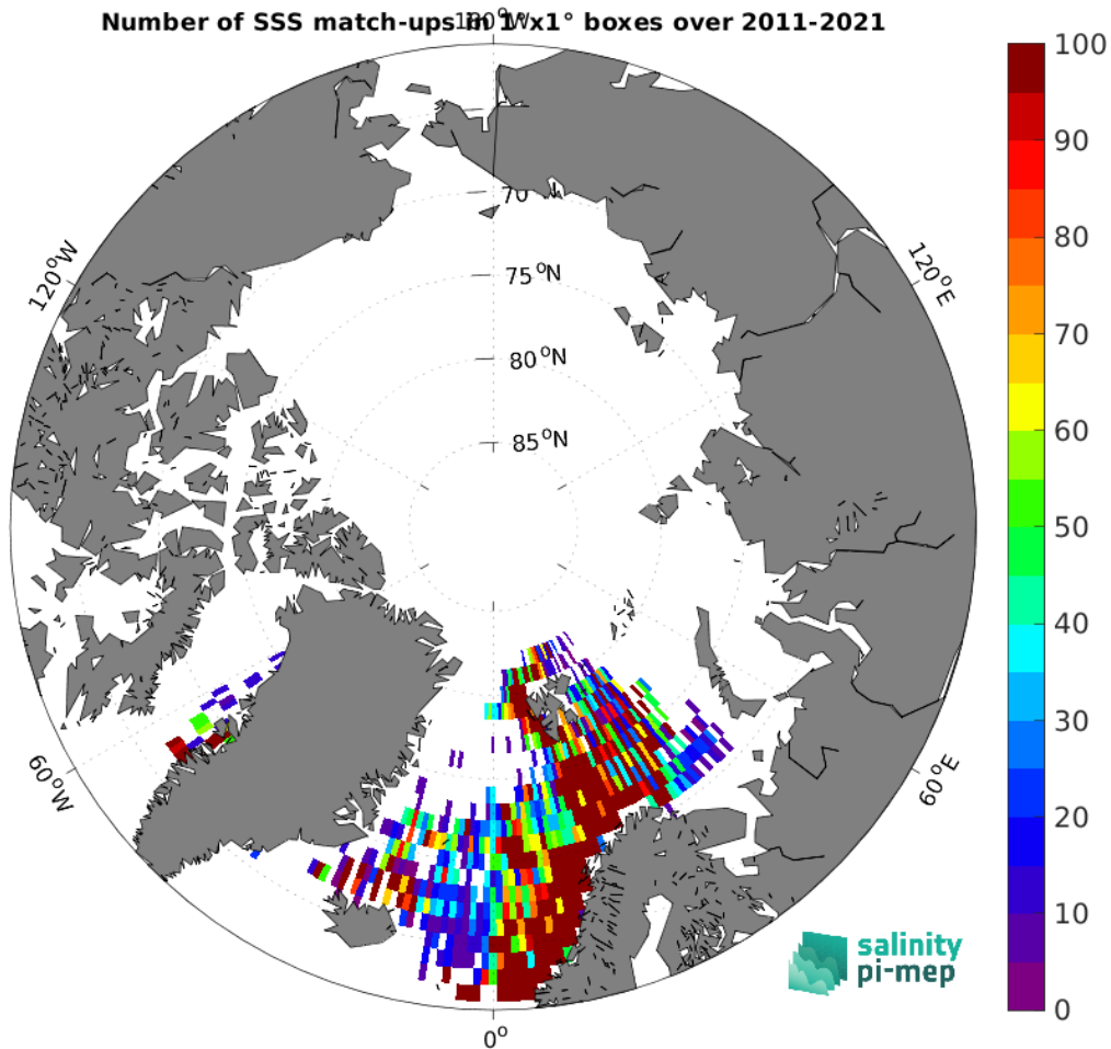
Figure 4: Number of SSS match-ups between ICES SSS and the SMOS SSS L3 v2 - 9-Days (BEC) SSS product for the Arctic Ocean Pi-MEP region over 1^\circ \times 1^\circ boxes and for the full satellite product period.
