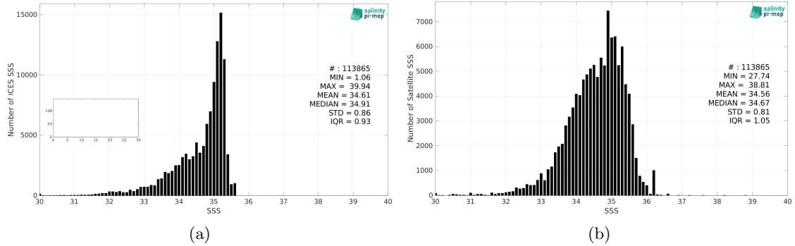
Figure 2: Histograms of SSS from ICES (a) and SMOS SSS L3 v2 - 9-Days (BEC) (b) considering all match-up pairs per bins of 0.1 over the Arctic Ocean Pi-MEP region and for the full satellite product period.
