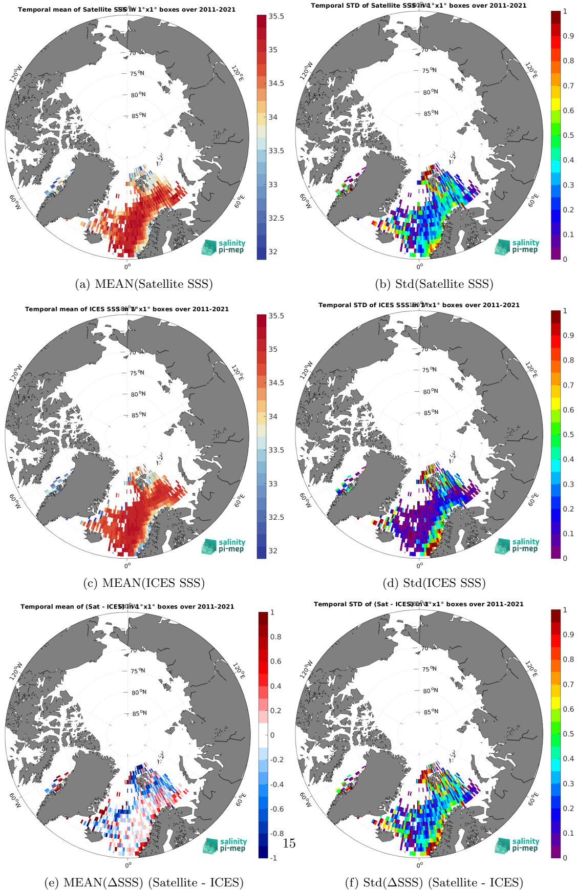
Figure 6: Temporal mean (left) and Std (right) of SSS from SMOS SSS L3 v2 - 9-Days (BEC) (top), ICES (middle), and of \Delta SSS (Satellite - ICES). Only match-up pairs are used to generate these maps.
