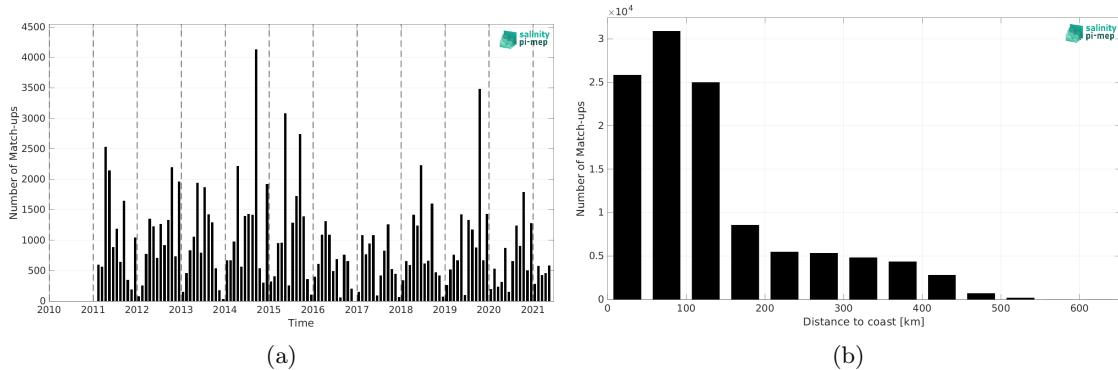
Figure 1: Number of match-ups between ICES and SMOS SSS L3 v2 - 9-Days (BEC) SSS as a function of time (a) and as function of the distance to coast (b) over the Arctic Ocean Pi-MEP region and for the full satellite product period.
