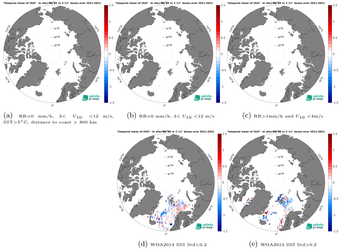
Figure 12: Temporal mean gridded over spatial boxes of size 1^{\circ}\times 1^{\circ} of \Delta\text{SSS} (SMOS SSS L3 v2 - 9-Days (BEC) - ICES) for 5 different subdatasets corresponding to:RR=0 mm/h, 3 < U_{10} < 12 m/s, SST >5^{\circ}\text{C} , distance to coast > 800 km (a), RR=0 mm/h, 3 < U_{10} < 12 m/s (b), RR >1 mm/h and U_{10} < 4 m/s (c), WOA2013 SSS Std <0.2 (d), WOA2013 SSS Std >0.2 (e).
