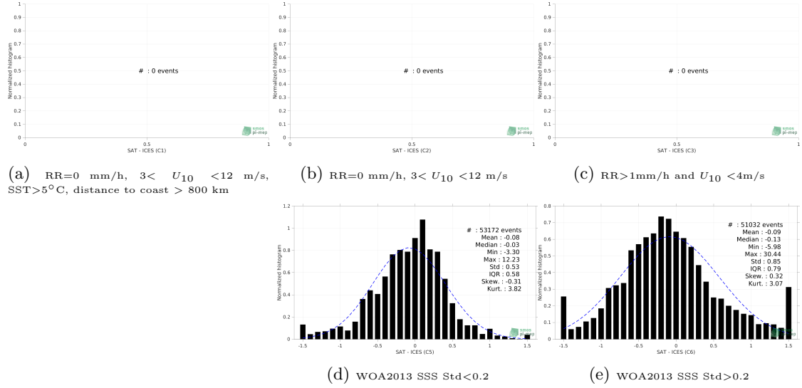
Figure 13: Normalized histogram of \Delta SSS (SMOS SSS L3 v2 - 9-Days (BEC) - ICES) for 5 different subdatasets corresponding to: RR=0 mm/h, 3 < U_{10} < 12 m/s, SST > 5°C, distance to coast > 800 km (a), RR=0 mm/h, 3 < U_{10} < 12 m/s (b), RR > 1mm/h and U_{10} < 4 m/s (c), WOA2013 SSS Std < 0.2 (d), WOA2013 SSS Std > 0.2 (e).
