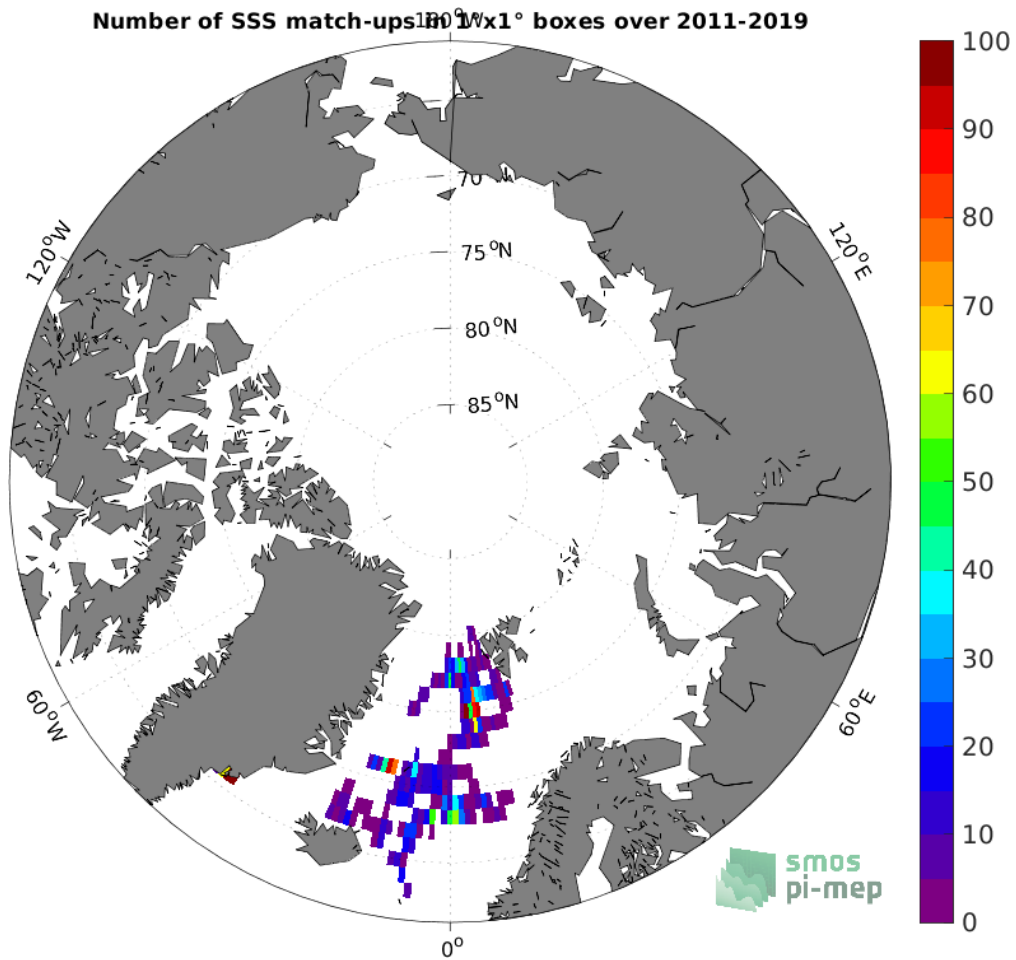
Figure 3: Number of SSS match-ups between Surface drifters SSS and the SMOS SSS L3 v2 - 9-Days (BEC) SSS product for the Arctic Ocean Pi-MEP region over 1^{\circ} \times 1^{\circ} boxes and for the full satellite product period.
