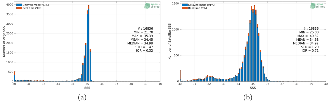
Figure 2: Histograms of SSS from Argo (a) and SMOS SSS L3 v2 - 9-Days (BEC) (b) considering all match-up pairs per bins of 0.1 over the Arctic Ocean Pi-MEP region and for the full satellite product period.
