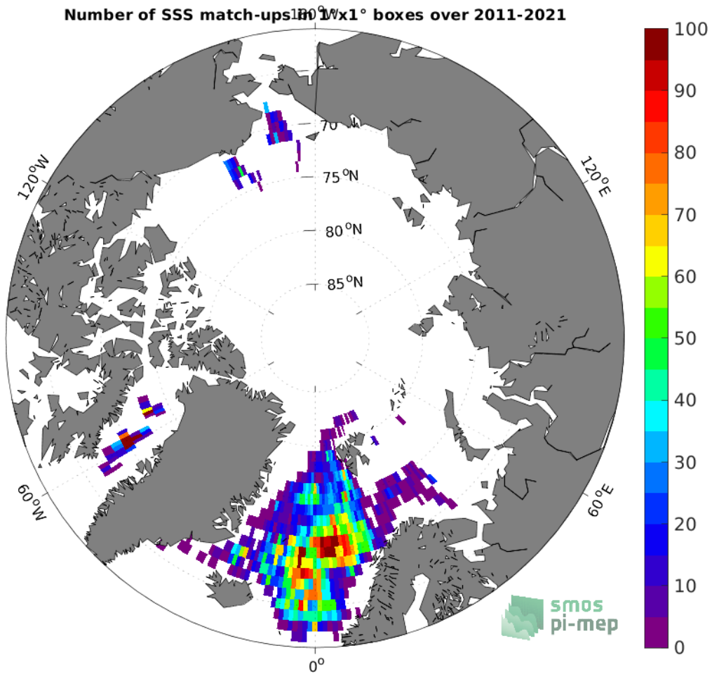
Figure 4: Number of SSS match-ups between Argo SSS and the SMOS SSS L3 v2 - 9-Days (BEC) SSS product for the Arctic Ocean Pi-MEP region over 1^{\circ} \times 1^{\circ} boxes and for the full satellite product period.
