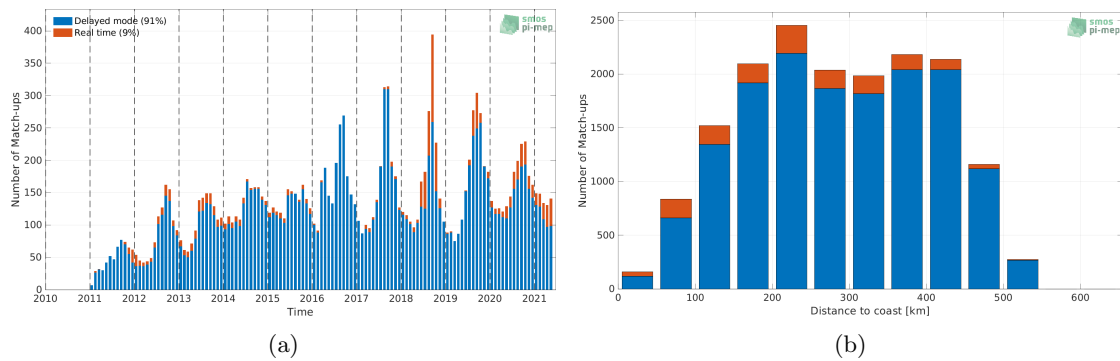
Figure 1: Number of match-ups between Argo and SMOS SSS L3 v2 - 9-Days (BEC) SSS as a function of time (a) and as function of the distance to coast (b) over the Arctic Ocean Pi-MEP region and for the full satellite product period.
