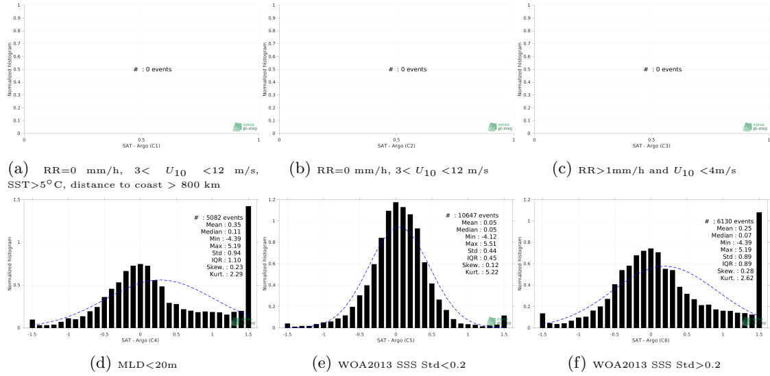
Figure 13: Normalized histogram of \Delta\text{SSS} (SMOS SSS L3 v2 - 9-Days (BEC) - Argo) for 6 different subdatasets corresponding to: RR=0 mm/h, 3 < U_{10} < 12 m/s, SST > 5^{\circ}\text{C} , distance to coast > 800 km (a), RR=0 mm/h, 3 < U_{10} < 12 m/s (b), RR > 1\text{mm/h} and U_{10} < 4\text{m/s} (c), MLD < 20\text{m} (d), WOA2013 SSS Std < 0.2 (e), WOA2013 SSS Std > 0.2 (f).
