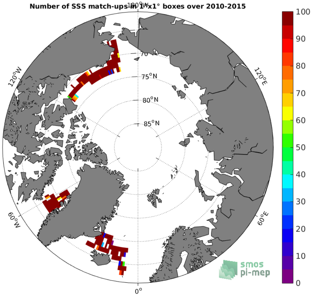
Figure 4: Number of SSS match-ups between TSG-SAMOS SSS and the SMOS-L3-BEC-OA-V1-9DAYS-0.25DEG SSS product for the Arctic Ocean Pi-MEP region over 1^\circ \times 1^\circ boxes and for the full satellite product period.
