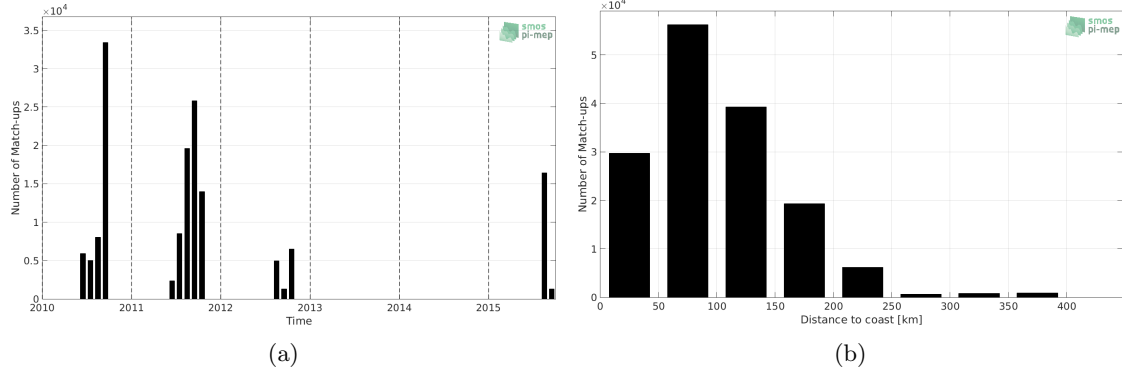
Figure 1: Number of match-ups between TSG-SAMOS and SMOS-L3-BEC-OA-V1-9DAYS-0.25DEG SSS as a function of time (a) and as function of the distance to coast (b) over the Arctic Ocean Pi-MEP region and for the full satellite product period.
