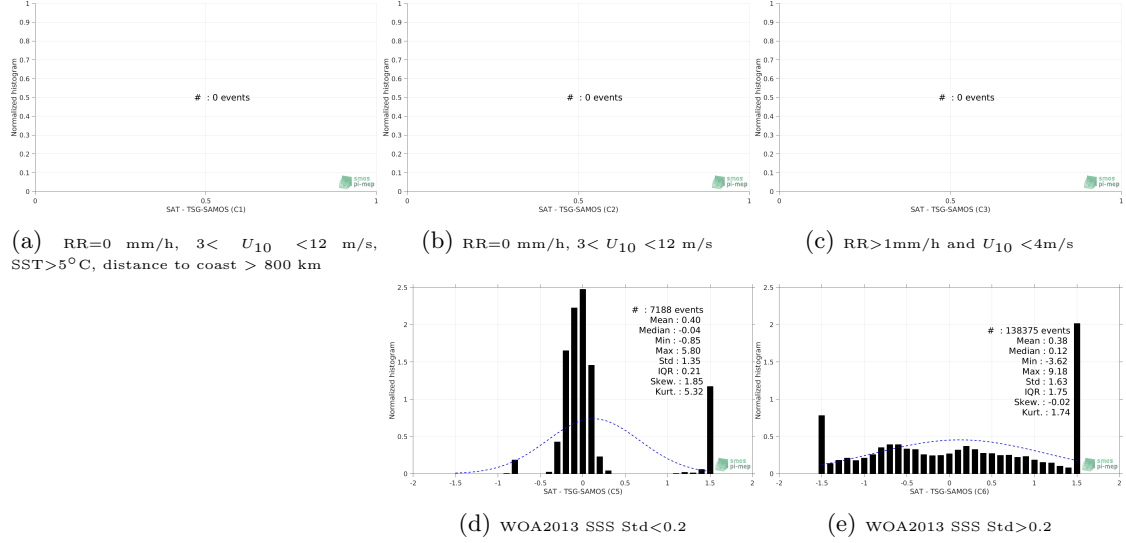
Figure 13: Normalized histogram of \Delta\text{SSS} (SMOS-L3-BEC-OA-V1-9DAYS-0.25DEG - TSG-SAMOS) for 5 different subdatasets corresponding to: RR=0 mm/h, 3 < U_{10} < 12 m/s, SST > 5^{\circ}\text{C} , distance to coast > 800 km (a), RR=0 mm/h, 3 < U_{10} < 12 m/s (b), RR > 1\text{mm/h} and U_{10} < 4\text{m/s} (c), WOA2013 SSS Std < 0.2 (d), WOA2013 SSS Std > 0.2 (e).
