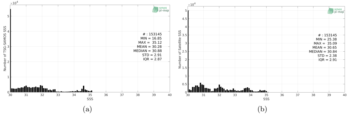
Figure 2: Histograms of SSS from TSG-SAMOS (a) and SMOS-L3-BEC-OA-V1-9DAYS-0.25DEG (b) considering all match-up pairs per bins of 0.1 over the Arctic Ocean Pi-MEP region and for the full satellite product period.
