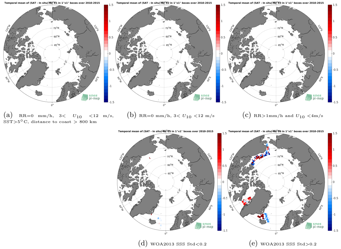
Figure 12: Temporal mean gridded over spatial boxes of size 1^\circ \times 1^\circ of \Delta SSS (SMOS-L3-BEC-OA-V1-9DAYS-0.25DEG - TSG-SAMOS) for 5 different subdatasets corresponding to:RR=0 mm/h, 3 < U_{10} < 12 m/s, SST >5^\circ\text{C} , distance to coast > 800 km (a), RR=0 mm/h, 3 < U_{10} < 12 m/s (b), RR >1 mm/h and U_{10} < 4 m/s (c), WOA2013 SSS Std <0.2 (d), WOA2013 SSS Std >0.2 (e).
