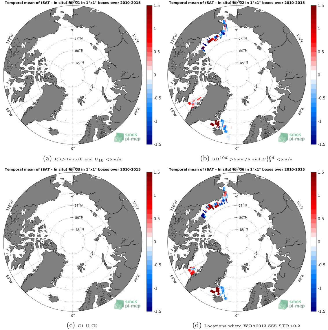
Figure 12: Temporal mean gridded over spatial boxes of size 1^\circ \times 1^\circ of \Delta SSS (SMOS-L3-BEC-OA-V1-9DAYS-0.25DEG - TSG-SAMOS) for 4 different subdatasets corresponding to: RR > 1\text{mm/h} and U_{10} < 5\text{m/s} (a), RR^{10d} > 5\text{mm/h} and U_{10}^{10d} < 5\text{m/s} (b), C1 U C2 (c), Locations where WOA2013 SSS STD > 0.2 (d).
