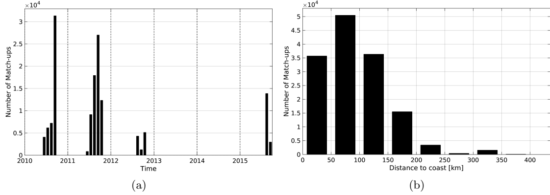
Figure 1: Number of match-ups between TSG-SAMOS and SMOS-L3-BEC-OA-V1-9DAYS-0.25DEG SSS as a function of time (a) and as function of the distance to coast (b) over the Arctic Ocean Pi-MEP region and for the full satellite product period.
