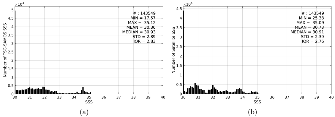
Figure 2: Histograms of SSS from TSG-SAMOS (a) and SMOS-L3-BEC-OA-V1-9DAYS-0.25DEG (b) considering all match-up pairs per bins of 0.1 over the Arctic Ocean Pi-MEP region and for the full satellite product period.
