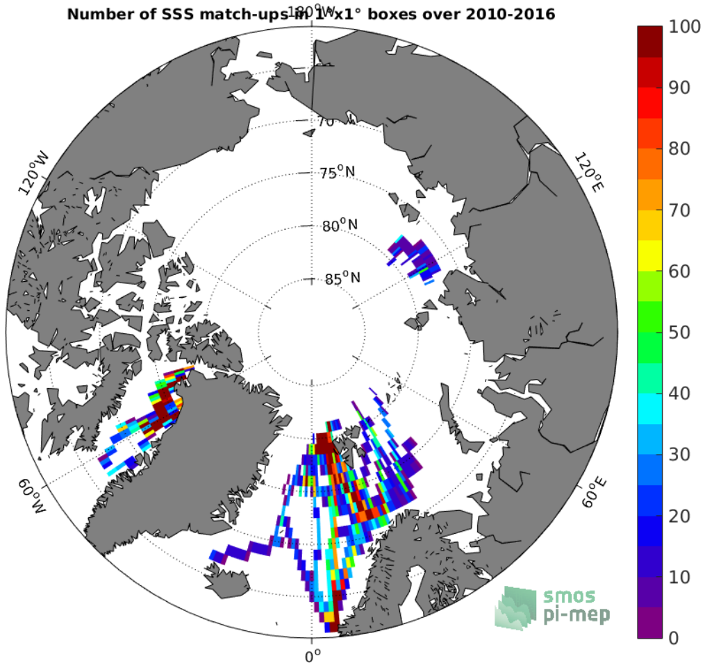
Figure 4: Number of SSS match-ups between TSG-POLARSTERN SSS and the SMOS-L3-BEC-OA-V1-9DAYS-0.25DEG SSS product for the Arctic Ocean Pi-MEP region over 1°x1° boxes and for the full satellite product period.
