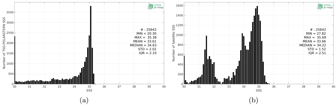
Figure 2: Histograms of SSS from TSG-POLARSTERN (a) and SMOS-L3-BEC-OA-V1-9DAYS-0.25DEG (b) considering all match-up pairs per bins of 0.1 over the Arctic Ocean Pi-MEP region and for the full satellite product period.
