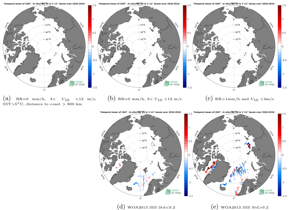
Figure 12: Temporal mean gridded over spatial boxes of size 1^\circ \times 1^\circ of \Delta SSS (SMOS-L3-BEC-OA-V1-9DAYS-0.25DEG - TSG-POLARSTERN) for 5 different subdatasets corresponding to:RR=0 mm/h, 3 < U_{10} < 12 m/s, SST >5^\circ\text{C} , distance to coast > 800 km (a), RR=0 mm/h, 3 < U_{10} < 12 m/s (b), RR >1 mm/h and U_{10} < 4 m/s (c), WOA2013 SSS Std <0.2 (d), WOA2013 SSS Std >0.2 (e).
