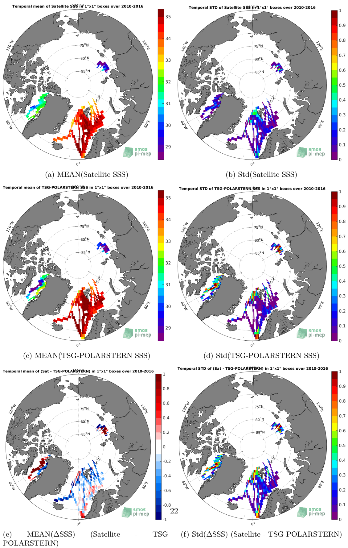
Figure 6: Temporal mean (left) and Std (right) of SSS from SMOS-L3-BEC-OA-V1-9DAYS-0.25DEG (top), TSG-POLARSTERN (middle), and of \Delta SSS (Satellite - TSG-POLARSTERN). Only match-up pairs are used to generate these maps.
