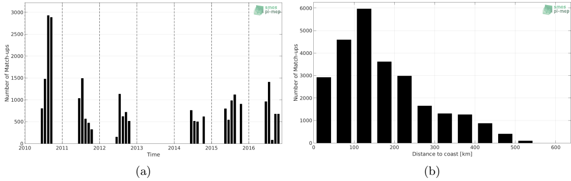
Figure 1: Number of match-ups between TSG-POLARSTERN and SMOS-L3-BEC-OA-V1-9DAYS-0.25DEG SSS as a function of time (a) and as function of the distance to coast (b) over the Arctic Ocean Pi-MEP region and for the full satellite product period.
