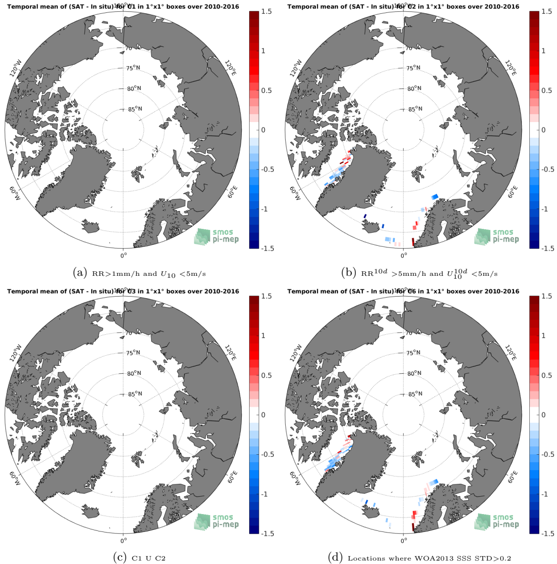
Figure 12: Temporal mean gridded over spatial boxes of size 1^\circ \times 1^\circ of \Delta SSS (SMOS-L3-BEC-OA-V1-9DAYS-0.25DEG - TSG-LEGOS-DM) for 4 different subdatasets corresponding to: RR > 1\text{mm/h} and U_{10} < 5\text{m/s} (a), RR ^{10d} > 5\text{mm/h} and U_{10}^{10d} < 5\text{m/s} (b), C1 U C2 (c), Locations where WOA2013 SSS STD > 0.2 (d).
