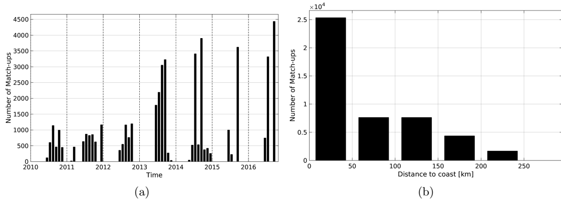
Figure 1: Number of match-ups between TSG-LEGOS-DM and SMOS-L3-BEC-OA-V1-9DAYS-0.25DEG SSS as a function of time (a) and as function of the distance to coast (b) over the Arctic Ocean Pi-MEP region and for the full satellite product period.
