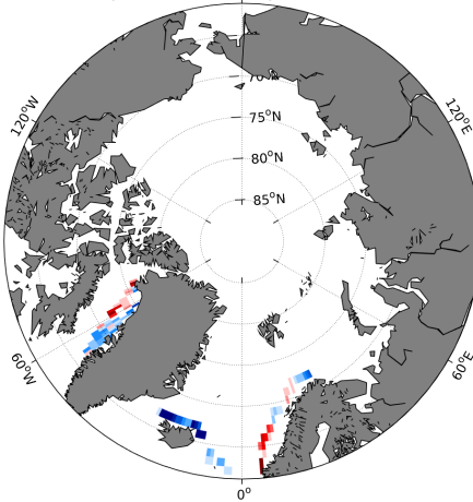
(e) MEAN( \Delta SSS) (Satellite - TSG-LEGOS-DM)
