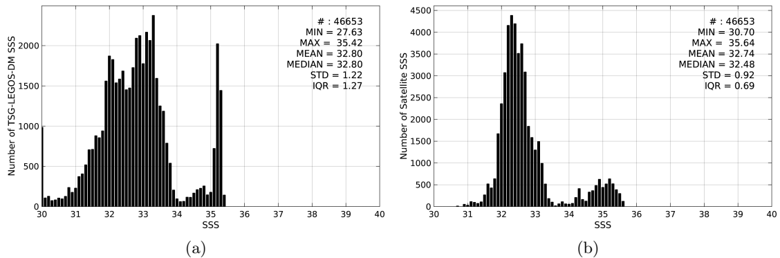
Figure 2: Histograms of SSS from TSG-LEGOS-DM (a) and SMOS-L3-BEC-OA-V1-9DAYS-0.25DEG (b) considering all match-up pairs per bins of 0.1 over the Arctic Ocean Pi-MEP region and for the full satellite product period.
