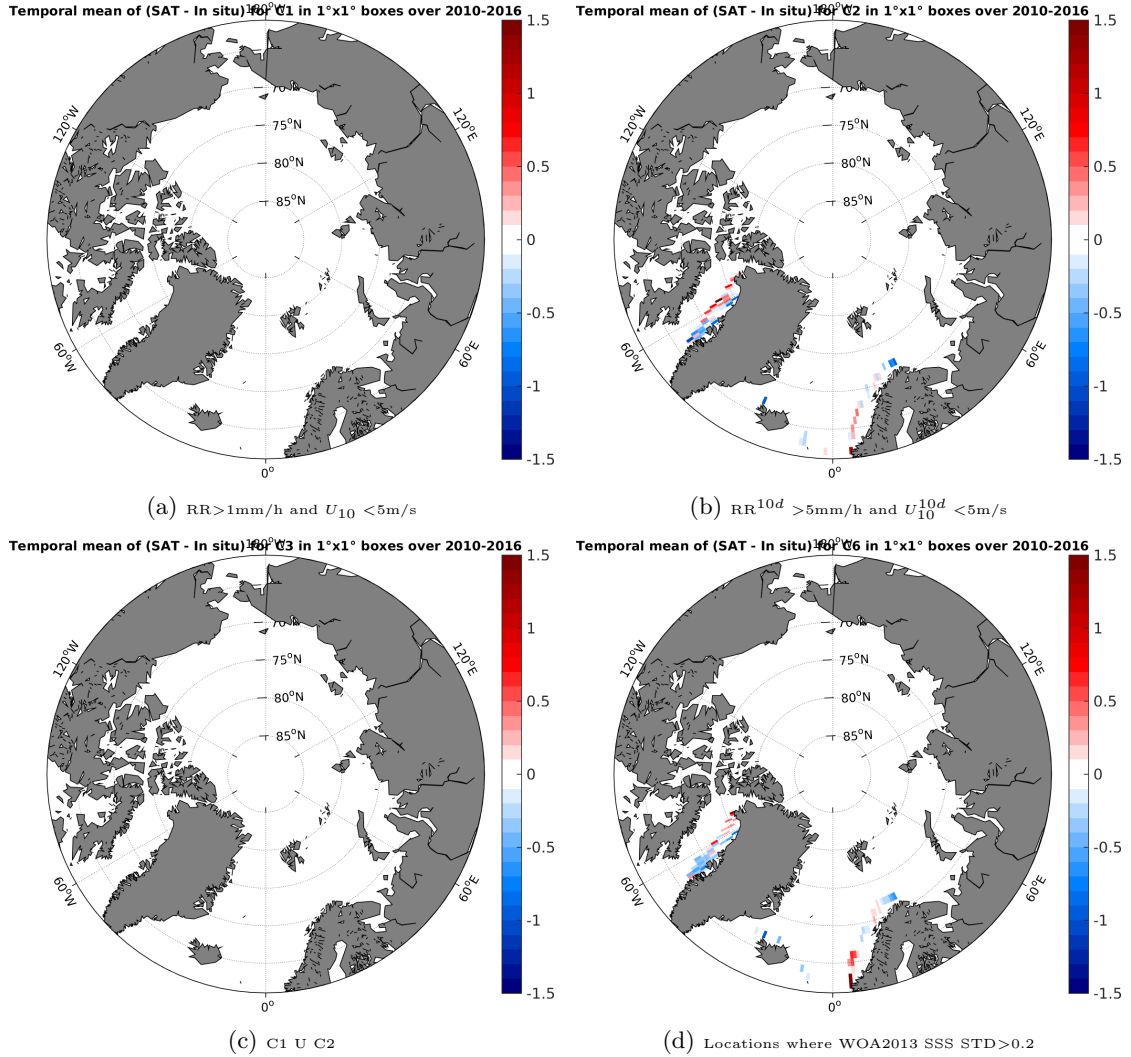
Figure 12: Temporal mean gridded over spatial boxes of size 1°x1° of \Delta SSS (SMOS-L3-BEC-OA-V1-9DAYS-0.25DEG - TSG-LEGOS-DM) for 4 different subdatasets corresponding to: RR > 1mm/h and U_{10} < 5\text{m/s} (a), RR^{10d} > 5\text{mm/h} and U_{10}^{10d} < 5\text{m/s} (b), C1 U C2 (c), Locations where WOA2013 SSS STD > 0.2 (d).
