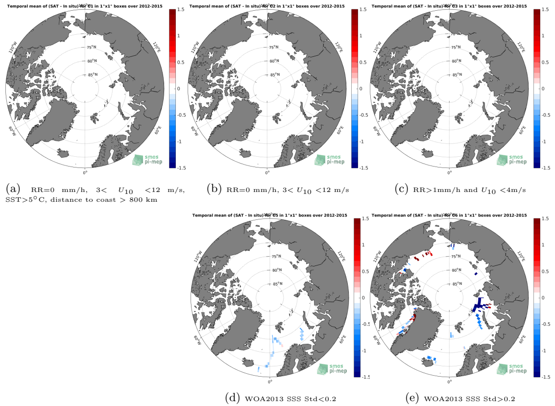
Figure 12: Temporal mean gridded over spatial boxes of size 1^\circ \times 1^\circ of \Delta SSS (SMOS-L3-BEC-OA-V1-9DAYS-0.25DEG - TSG-GOSUD-Sailing-ship) for 5 different subdatasets corresponding to:RR=0 mm/h, 3 < U_{10} < 12 m/s, SST >5^\circ C, distance to coast > 800 km (a), RR=0 mm/h, 3 < U_{10} < 12 m/s (b), RR >1 mm/h and U_{10} < 4 m/s (c), WOA2013 SSS Std <0.2 (d), WOA2013 SSS Std >0.2 (e).
