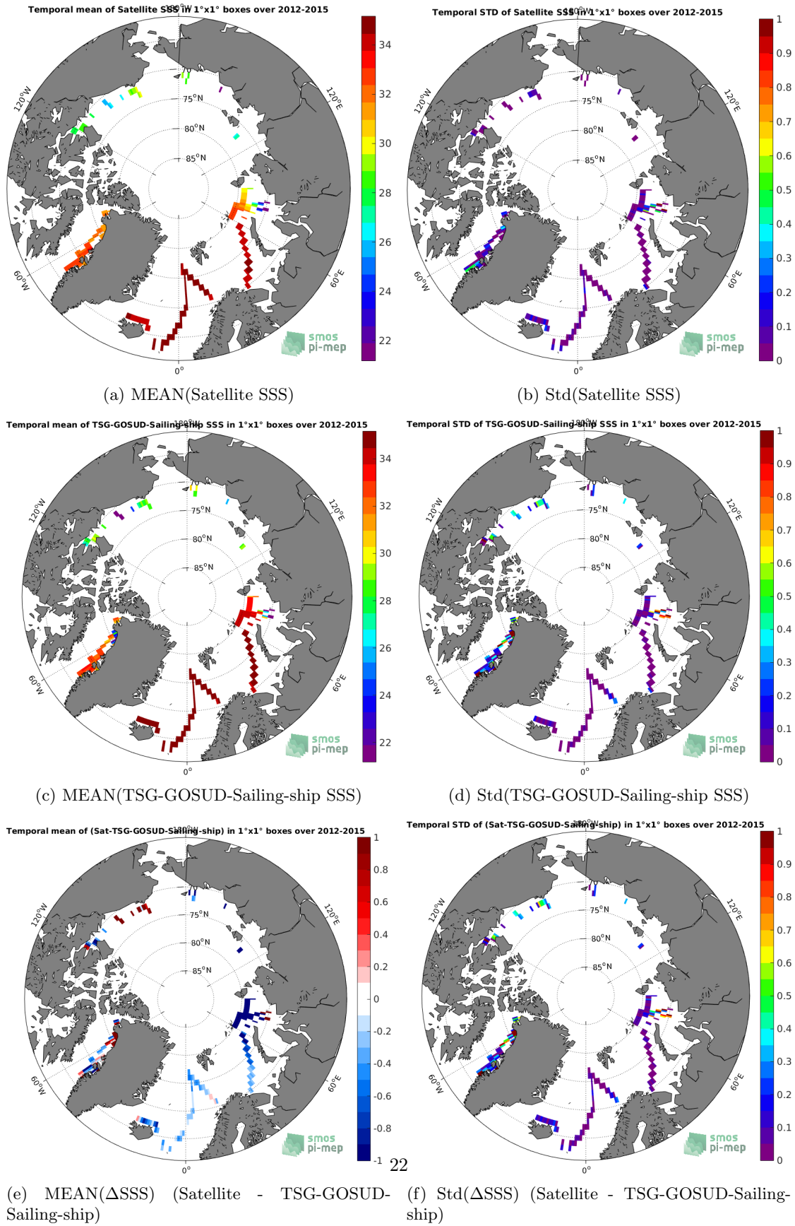
Figure 6: Temporal mean (left) and Std (right) of SSS from SMOS-L3-BEC-OA-V1-9DAYS-0.25DEG (top), TSG-GOSUD-Sailing-ship (middle), and of \Delta SSS (Satellite - TSG-GOSUD-Sailing-ship). Only match-up pairs are used to generate these maps.
