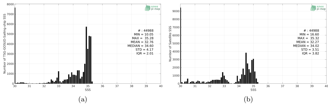
Figure 2: Histograms of SSS from TSG-GOSUD-Sailing-ship (a) and SMOS-L3-BEC-OA-V1-9DAYS-0.25DEG (b) considering all match-up pairs per bins of 0.1 over the Arctic Ocean Pi-MEP region and for the full satellite product period.
