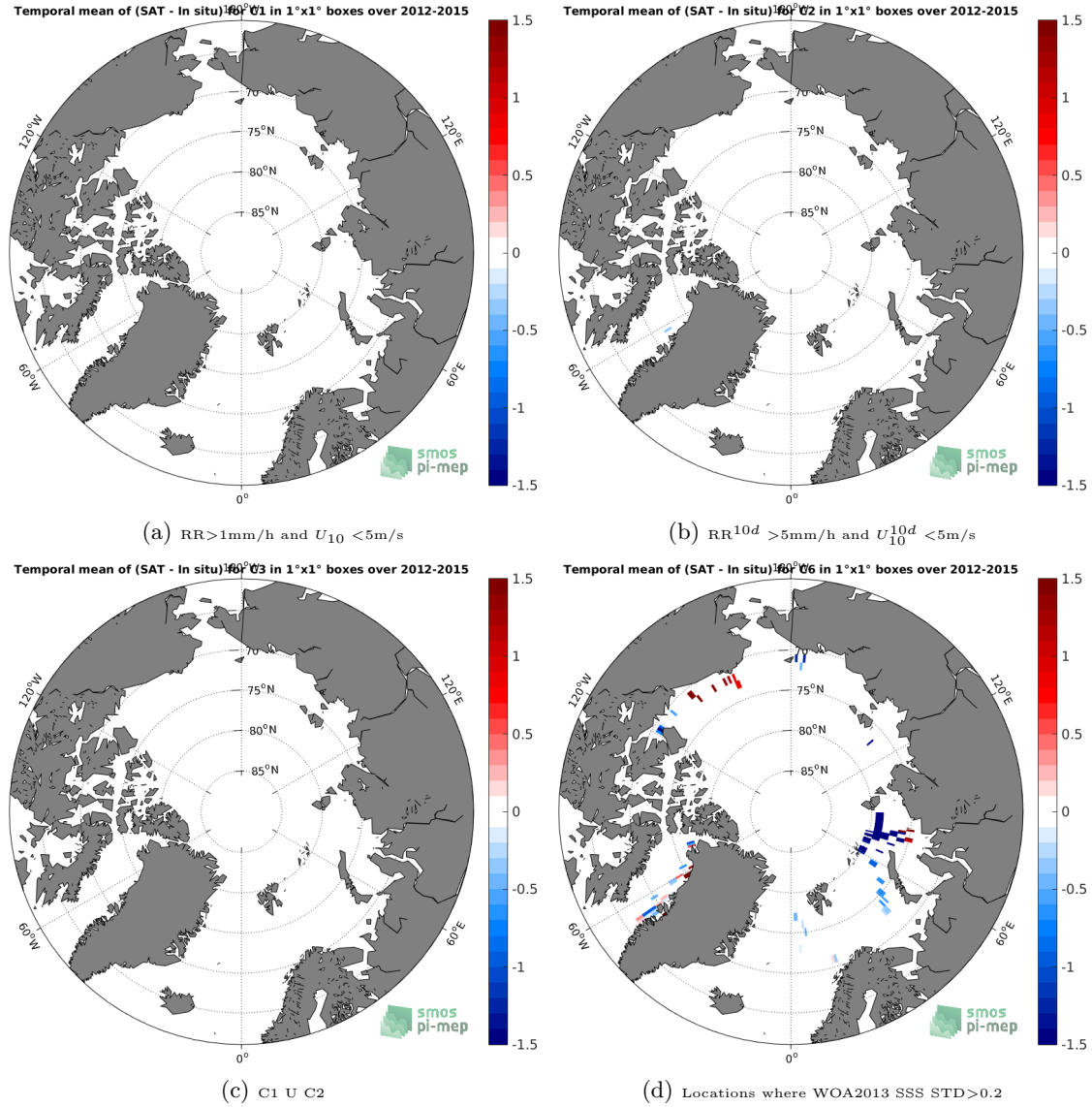
Figure 12: Temporal mean gridded over spatial boxes of size 1^\circ \times 1^\circ of \Delta SSS (SMOS-L3-BEC-OA-V1-9DAYS-0.25DEG - TSG-GOSUD-Sailing-ship) for 4 different subdatasets corresponding to: RR > 1\text{mm/h} and U_{10} < 5\text{m/s} (a), RR^{10d} > 5\text{mm/h} and U_{10}^{10d} < 5\text{m/s} (b), C1 U C2 (c), Locations where WOA2013 SSS STD > 0.2 (d).
