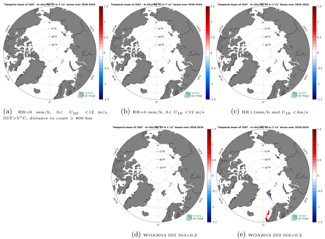
Figure 12: Temporal mean gridded over spatial boxes of size 1^\circ \times 1^\circ of \Delta\text{SSS} (SMOS-L3-BEC-OA-V1-9DAYS-0.25DEG - TSG-GOSUD-Research-vessel) for 5 different subdatasets corresponding to:RR=0 mm/h, 3 < U_{10} < 12 m/s, SST>5°C, distance to coast > 800 km (a), RR=0 mm/h, 3 < U_{10} < 12 m/s (b), RR>1mm/h and U_{10} < 4 m/s (c), WOA2013 SSS Std<0.2 (d), WOA2013 SSS Std>0.2 (e).
