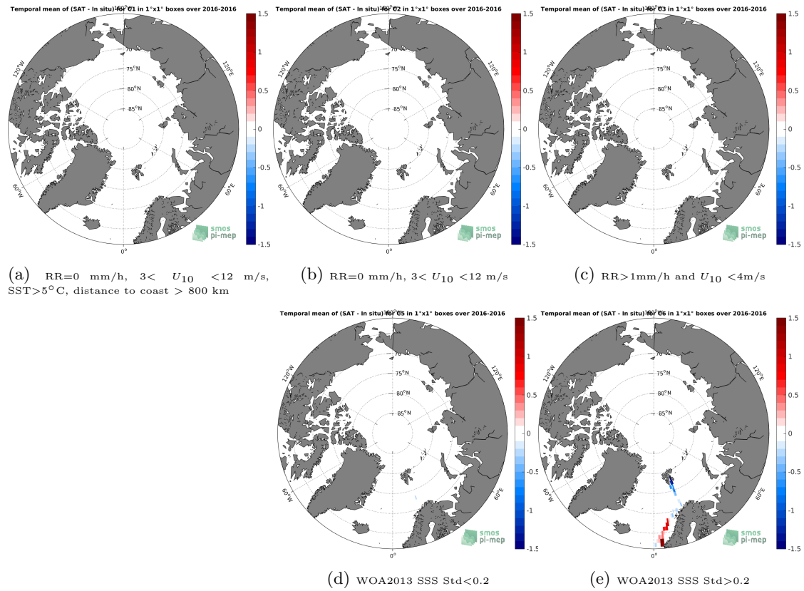
Figure 12: Temporal mean gridded over spatial boxes of size 1^\circ \times 1^\circ of \Delta SSS (SMOS-L3-BEC-OA-V1-9DAYS-0.25DEG - TSG-GOSUD-Research-vessel) for 5 different subdatasets corresponding to:RR=0 mm/h, 3 < U_{10} < 12 m/s, SST >5^\circ C, distance to coast > 800 km (a), RR=0 mm/h, 3 < U_{10} < 12 m/s (b), RR >1 mm/h and U_{10} < 4 m/s (c), WOA2013 SSS Std <0.2 (d), WOA2013 SSS Std >0.2 (e).
