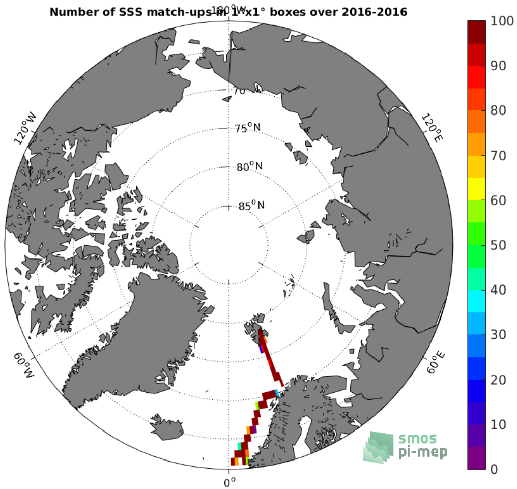
Figure 4: Number of SSS match-ups between TSG-GOSUD-Research-vessel SSS and the SMOS-L3-BEC-OA-V1-9DAYS-0.25DEG SSS product for the Arctic Ocean Pi-MEP region over 1°x1° boxes and for the full satellite product period.
