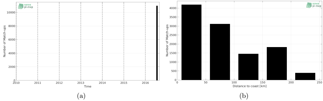
Figure 1: Number of match-ups between TSG-GOSUD-Research-vessel and SMOS-L3-BEC-OA-V1-9DAYS-0.25DEG SSS as a function of time (a) and as function of the distance to coast (b) over the Arctic Ocean Pi-MEP region and for the full satellite product period.
