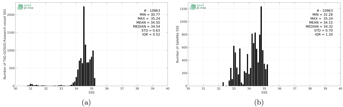
Figure 2: Histograms of SSS from TSG-GOSUD-Research-vessel (a) and SMOS-L3-BEC-OA-V1-9DAYS-0.25DEG (b) considering all match-up pairs per bins of 0.1 over the Arctic Ocean Pi-MEP region and for the full satellite product period.
