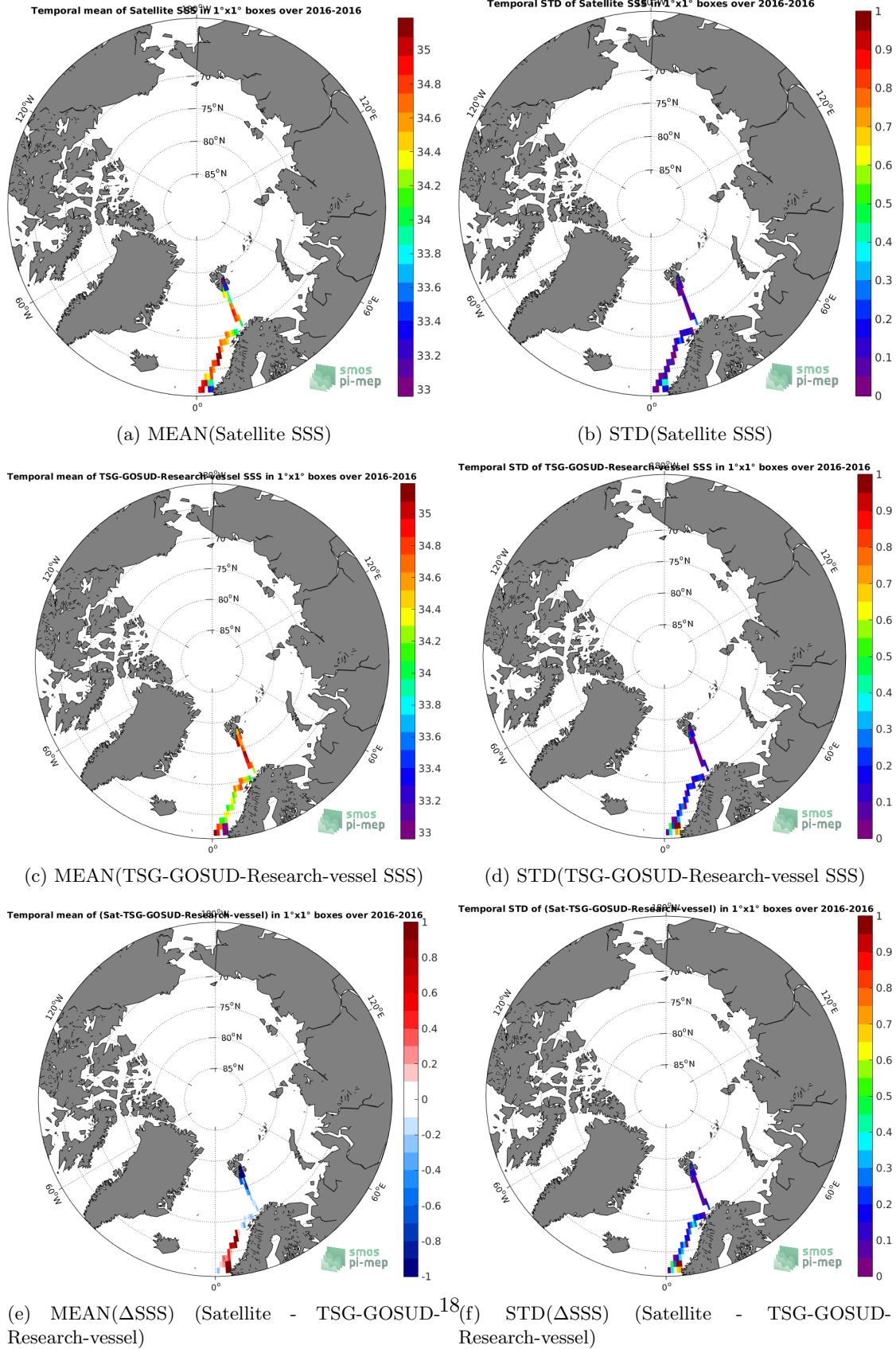
Figure 6: Temporal mean (left) and STD (right) of SSS from SMOS-L3-BEC-OA-V1-9DAYS-0.25DEG (top), TSG-GOSUD-Research-vessel (middle), and of \Delta SSS (Satellite - TSG-GOSUD-Research-vessel). Only match-up pairs are used to generate these maps.
