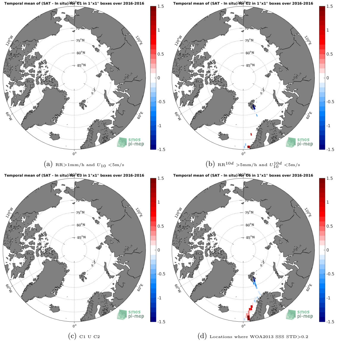
Figure 12: Temporal mean gridded over spatial boxes of size 1^\circ \times 1^\circ of \Delta SSS (SMOS-L3-BEC-OA-V1-9DAYS-0.25DEG - TSG-GOSUD-Research-vessel) for 4 different subdatasets corresponding to: RR > 1\text{mm/h} and U_{10} < 5\text{m/s} (a), RR^{10d} > 5\text{mm/h} and U_{10}^{10d} < 5\text{m/s} (b), C1 U C2 (c), Locations where WOA2013 SSS STD > 0.2 (d).
