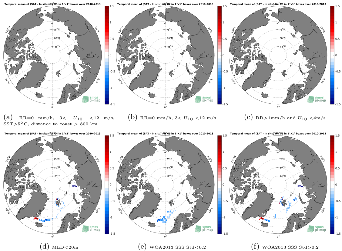
Figure 12: Temporal mean gridded over spatial boxes of size 1^\circ \times 1^\circ of \Delta SSS (SMOS-L3-BEC-OA-V1-9DAYS-0.25DEG - Sea mammals) for 6 different subdatasets corresponding to:RR=0 mm/h, 3 < U_{10} < 12 m/s, SST >5^\circ C, distance to coast > 800 km (a), RR=0 mm/h, 3 < U_{10} < 12 m/s (b), RR >1 mm/h and U_{10} < 4 m/s (c),MLD <20 m (d),WOA2013 SSS Std <0.2 (e),WOA2013 SSS Std >0.2 (f).
