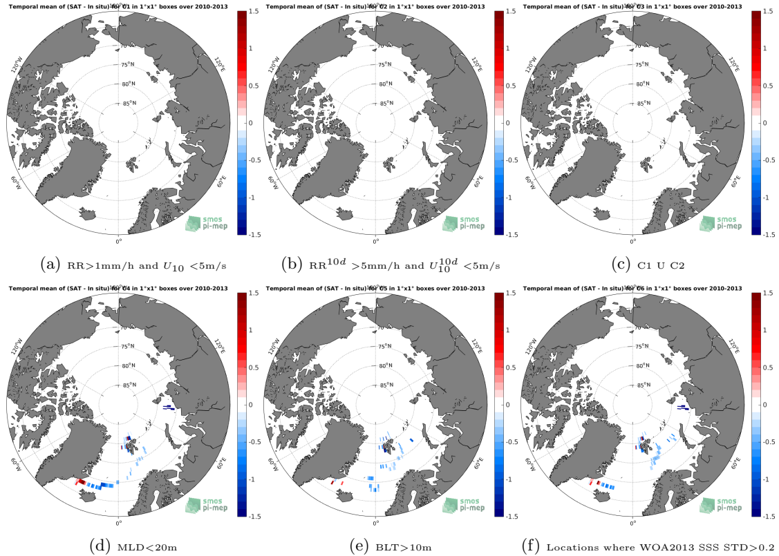
Figure 12: Temporal mean gridded over spatial boxes of size 1^\circ \times 1^\circ of \Delta SSS (SMOS-L3-BEC-OA-V1-9DAYS-0.25DEG - Sea mammals) for 6 different subdatasets corresponding to: RR > 1\text{mm/h} and U_{10} < 5\text{m/s} (a), RR^{10d} > 5\text{mm/h} and U_{10}^{10d} < 5\text{m/s} (b), C1 U C2 (c), MLD < 20\text{m} (d), BLT > 10\text{m} (e), Locations where WOA2013 SSS STD > 0.2 (f).
