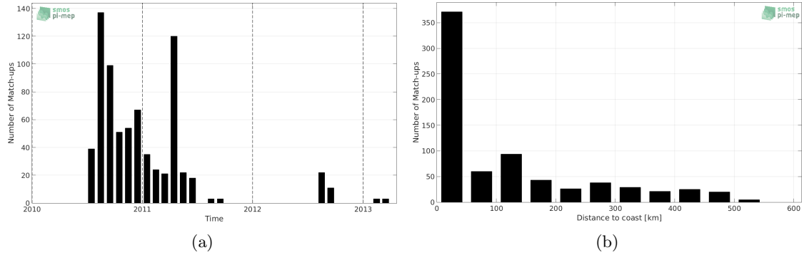
Figure 1: Number of match-ups between Sea mammals and SMOS-L3-BEC-OA-V1-9DAYS-0.25DEG SSS as a function of time (a) and as function of the distance to coast (b) over the Arctic Ocean Pi-MEP region and for the full satellite product period.
