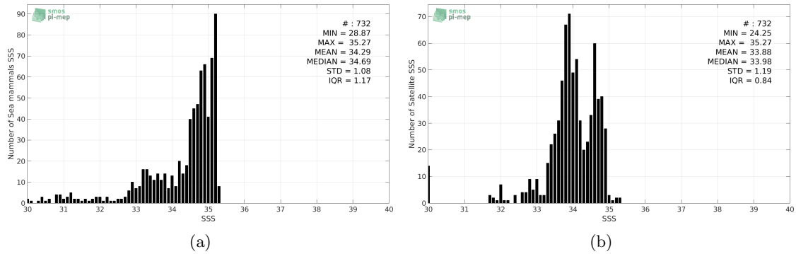
Figure 2: Histograms of SSS from Sea mammals (a) and SMOS-L3-BEC-OA-V1-9DAYS-0.25DEG (b) considering all match-up pairs per bins of 0.1 over the Arctic Ocean Pi-MEP region and for the full satellite product period.
