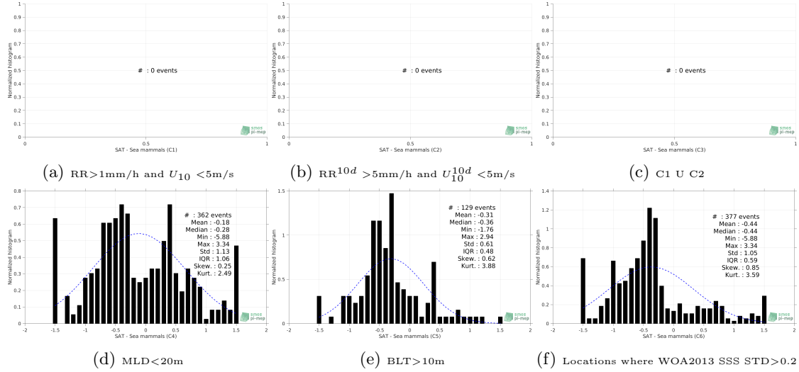
Figure 13: Normalized histogram of \Delta SSS (SMOS-L3-BEC-OA-V1-9DAYS-0.25DEG - Sea mammals) for 6 different subdatasets corresponding to: RR>1mm/h and U_{10} < 5\text{m/s} (a), RR^{10d} > 5\text{mm/h} and U_{10}^{10d} < 5\text{m/s} (b), C1 U C2 (c), MLD<20m (d), BLT>10m (e), Locations where WOA2013 SSS STD>0.2 (f).
