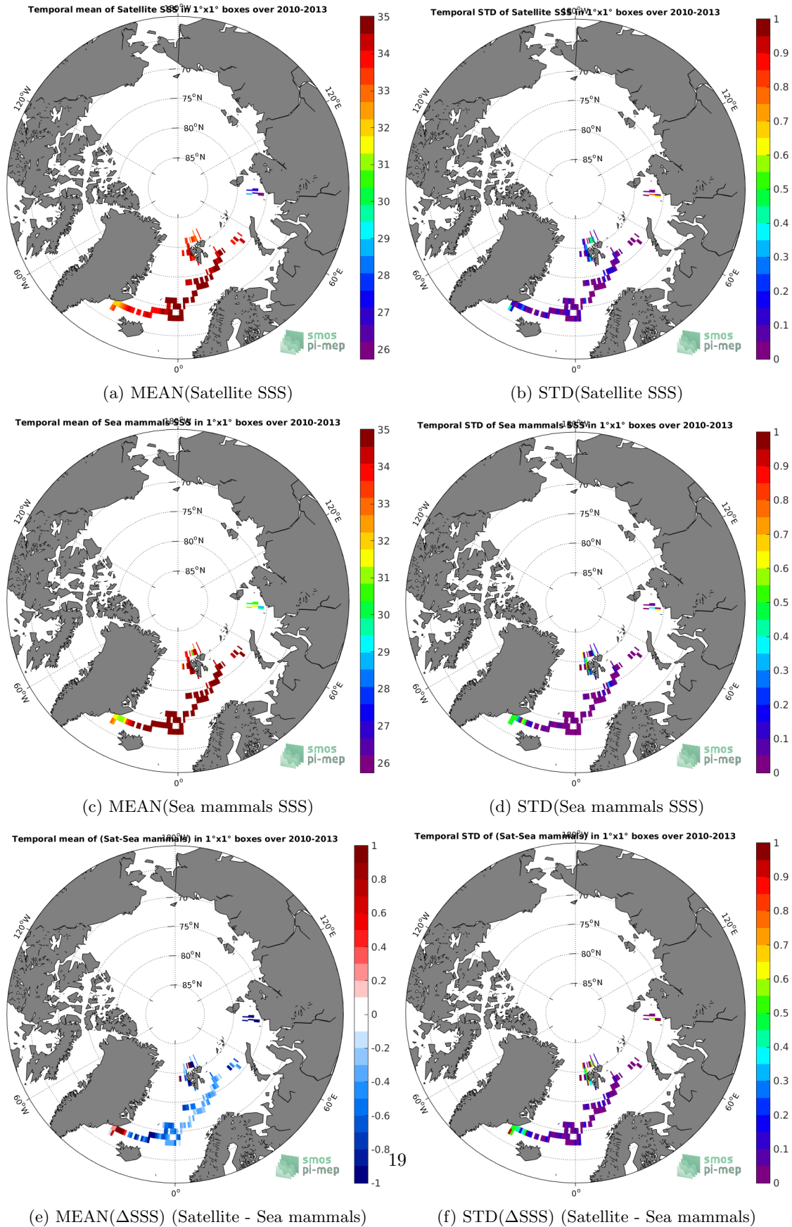
Figure 6: Temporal mean (left) and STD (right) of SSS from SMOS-L3-BEC-OA-V1-9DAYS-0.25DEG (top), Sea mammals (middle), and of \Delta SSS (Satellite - Sea mammals). Only match-up pairs are used to generate these maps.
