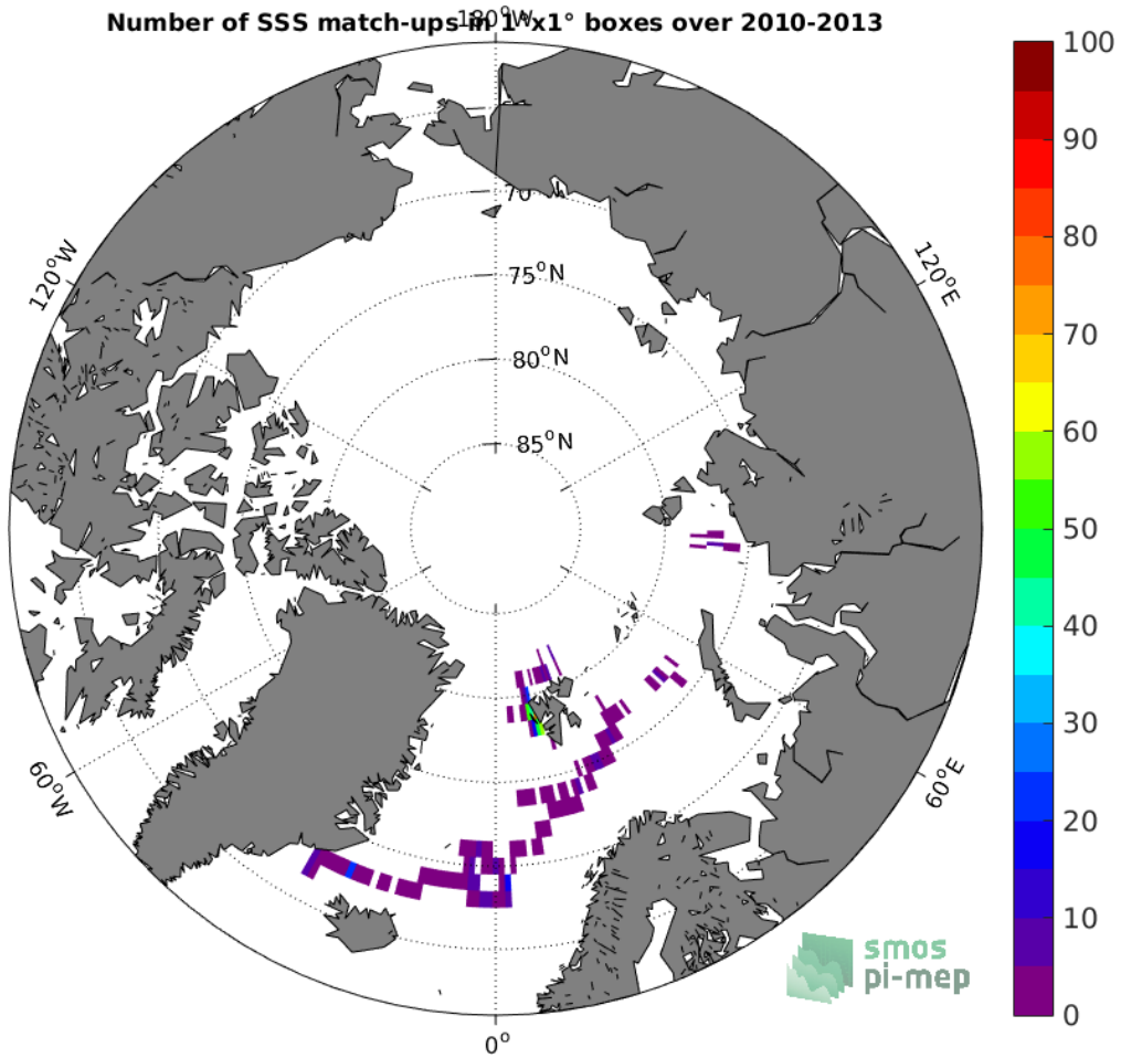
Figure 4: Number of SSS match-ups between Sea mammals SSS and the SMOS-L3-BEC-OA-V1-9DAYS-0.25DEG SSS product for the Arctic Ocean Pi-MEP region over 1°x1° boxes and for the full satellite product period.
