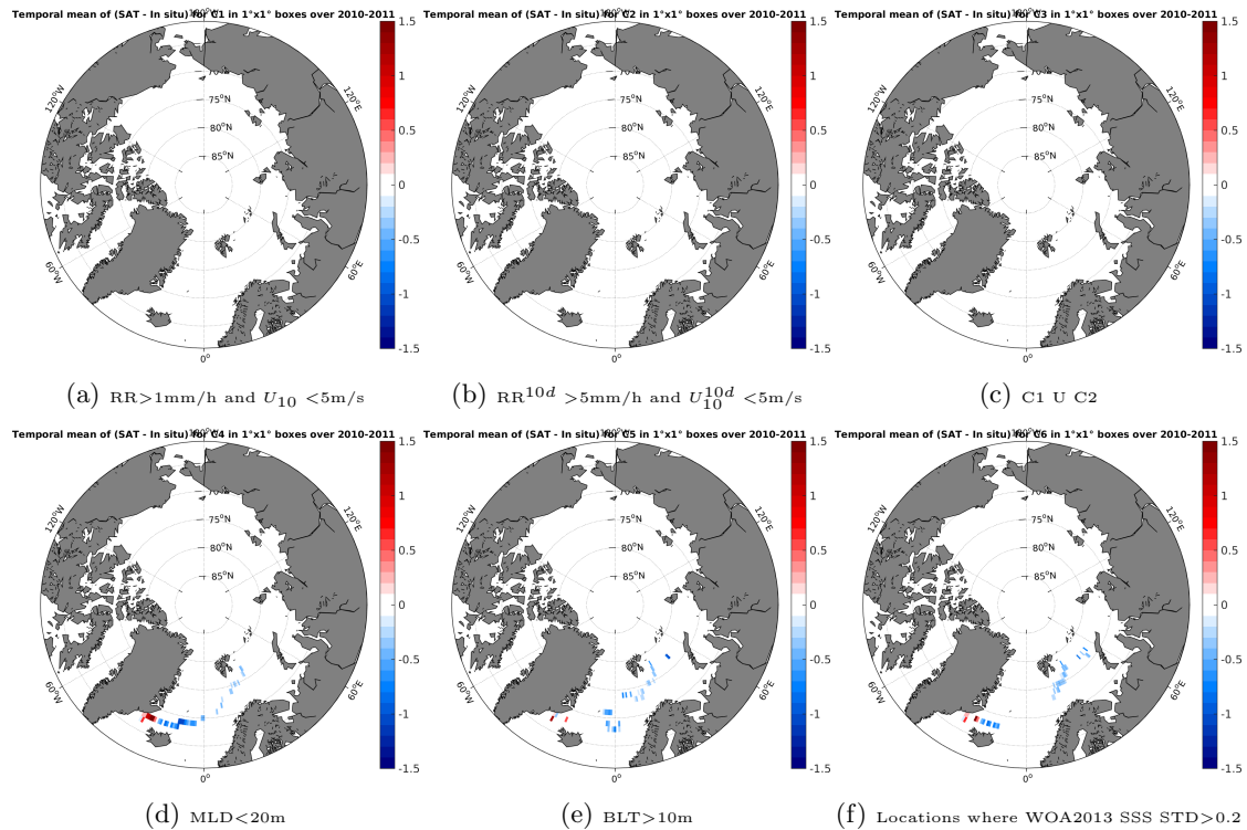
Figure 12: Temporal mean gridded over spatial boxes of size 1^\circ \times 1^\circ of \Delta SSS (SMOS-L3-BEC-OA-V1-9DAYS-0.25DEG - Sea mammals) for 6 different subdatasets corresponding to: RR > 1\text{mm/h} and U_{10} < 5\text{m/s} (a), RR^{10d} > 5\text{mm/h} and U_{10}^{10d} < 5\text{m/s} (b), C1 U C2 (c), MLD < 20\text{m} (d), BLT > 10\text{m} (e), Locations where WOA2013 SSS STD > 0.2 (f).
