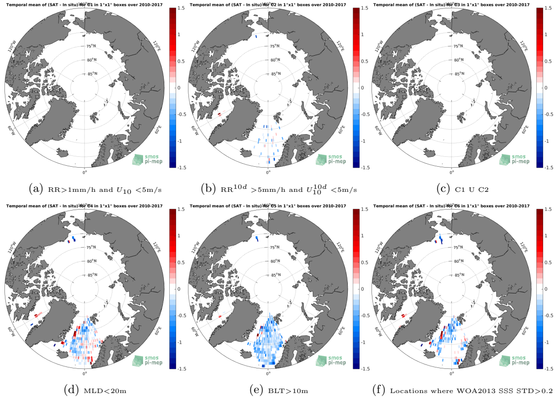
Figure 12: Temporal mean gridded over spatial boxes of size 1^\circ \times 1^\circ of \Delta SSS (SMOS-L3-BEC-OA-V1-9DAYS-0.25DEG - Argo) for 6 different subdatasets corresponding to: RR > 1\text{mm/h} and U_{10} < 5\text{m/s} (a), RR^{10d} > 5\text{mm/h} and U_{10}^{10d} < 5\text{m/s} (b), C1 U C2 (c), MLD < 20\text{m} (d), BLT > 10\text{m} (e), Locations where WOA2013 SSS STD > 0.2 (f).
