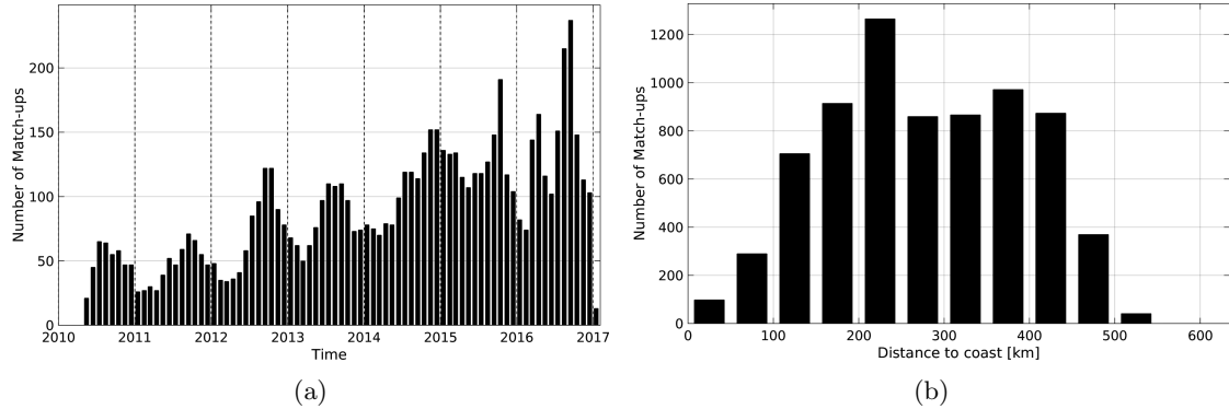
Figure 1: Number of match-ups between Argo and SMOS-L3-BEC-OA-V1-9DAYS-0.25DEG SSS as a function of time (a) and as function of the distance to coast (b) over the Arctic Ocean Pi-MEP region and for the full satellite product period.
