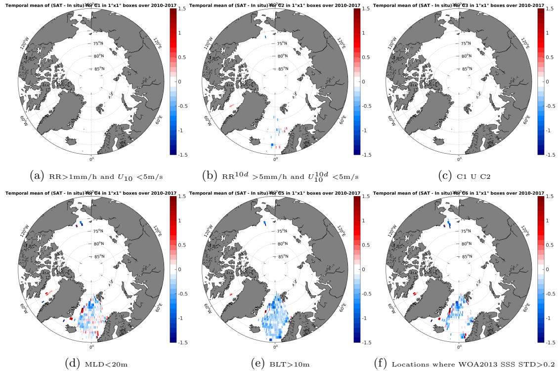
Figure 12: Temporal mean gridded over spatial boxes of size 1^\circ \times 1^\circ of \Delta SSS (SMOS-L3-BEC-OA-V1-9DAYS-0.25DEG - Argo) for 6 different subdatasets corresponding to:RR>1mm/h and U_{10} < 5 m/s (a), RR^{10d} > 5 mm/h and U_{10}^{10d} < 5 m/s (b), C1 U C2 (c),MLD<20m (d),BLT>10m (e),Locations where WOA2013 SSS STD>0.2 (f).
