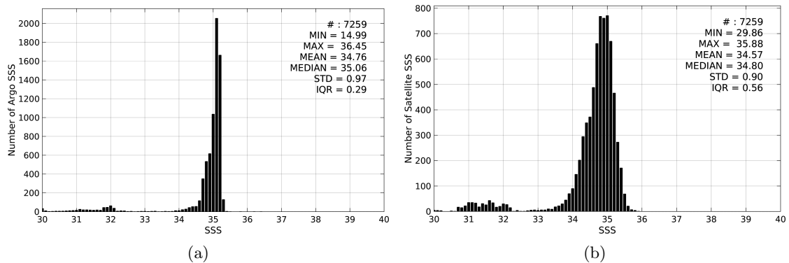
Figure 2: Histograms of SSS from Argo (a) and SMOS-L3-BEC-OA-V1-9DAYS-0.25DEG (b) considering all match-up pairs per bins of 0.1 over the Arctic Ocean Pi-MEP region and for the full satellite product period.
