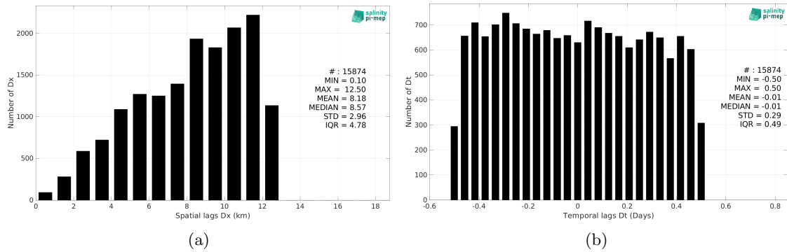
Figure 6: Histograms of the spatial (a) and temporal (b) lags between the location/time of the TSG (SAMOS) measurement and the date of the corresponding SMOS SSS L3 Arctic v4 - 9 Days (BEC) SSS pixel.
