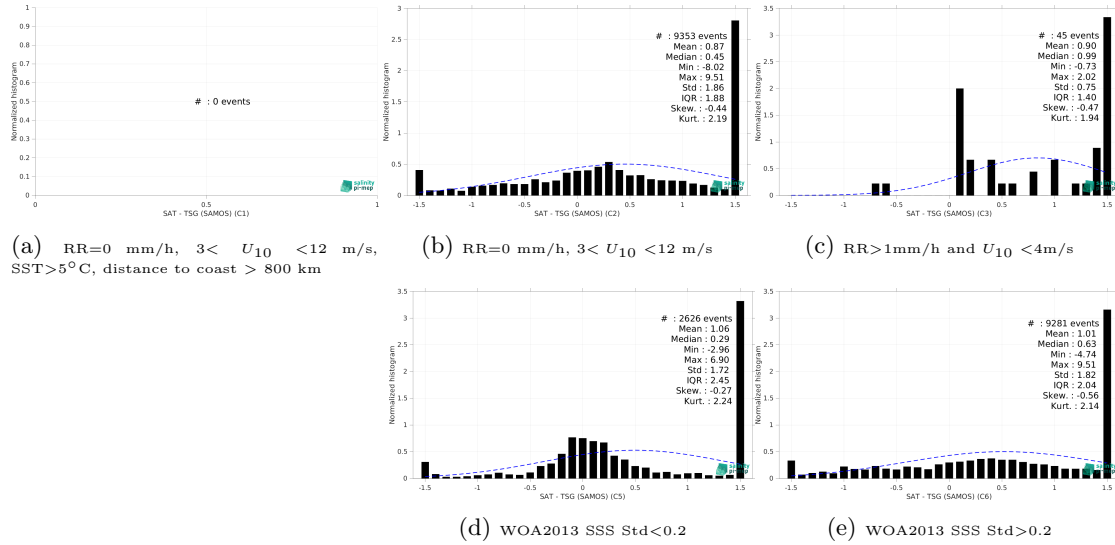
Figure 15: Normalized histogram of \Delta SSS (SMOS SSS L3 Arctic v4 - 9 Days (BEC) - TSG (SAMOS)) for 5 different subdatasets corresponding to: RR=0 mm/h, 3 < U_{10} < 12 m/s, SST > 5°C, distance to coast > 800 km (a), RR=0 mm/h, 3 < U_{10} < 12 m/s (b), RR > 1mm/h and U_{10} < 4 m/s (c), WOA2013 SSS Std < 0.2 (d), WOA2013 SSS Std > 0.2 (e).
