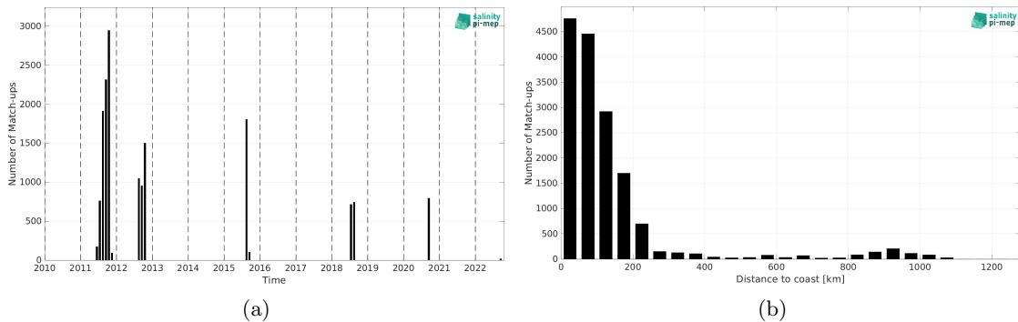
Figure 2: Number of match-ups between TSG (SAMOS) and SMOS SSS L3 Arctic v4 - 9 Days (BEC) SSS as a function of time (a) and as function of the distance to coast (b) over the Arctic Ocean Pi-MEP region and for the full satellite product period.
