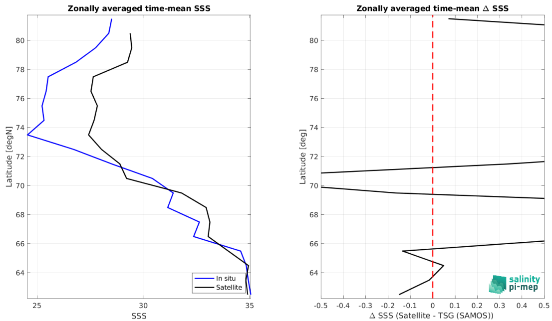
Figure 9: Left panel: Zonal mean SSS from SMOS SSS L3 Arctic v4 - 9 Days (BEC) satellite product (black) and from TSG (SAMOS) (blue). Right panel: Zonal mean of \Delta SSS (Satellite - TSG (SAMOS)) for all the collected Pi-MEP match-up pairs estimated over the full satellite product period.
