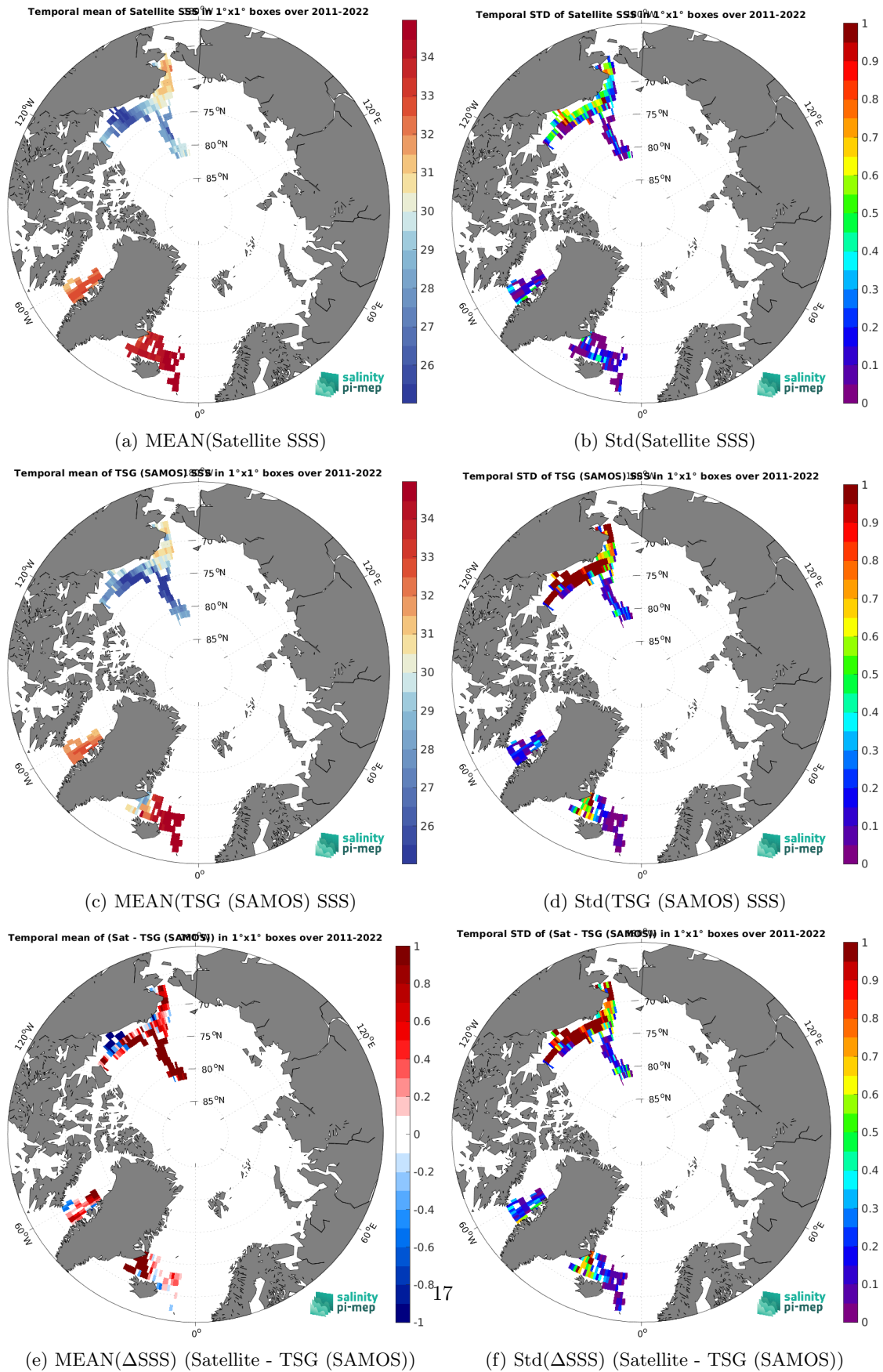
Figure 7: Temporal mean (left) and Std (right) of SSS from SMOS SSS L3 Arctic v4 - 9 Days (BEC) (top), TSG (SAMOS) (middle), and of \Delta SSS (Satellite - TSG (SAMOS)). Only match-up pairs are used to generate these maps.
