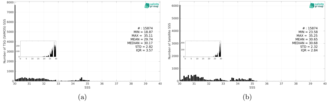
Figure 3: Histograms of SSS from TSG (SAMOS) (a) and SMOS SSS L3 Arctic v4 - 9 Days (BEC) (b) considering all match-up pairs per bins of 0.1 over the Arctic Ocean Pi-MEP region and for the full satellite product period.
