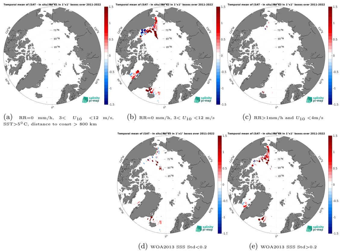
Figure 14: Temporal mean gridded over spatial boxes of size 1^\circ \times 1^\circ of \Delta\text{SSS} (SMOS SSS L3 Arctic v4 - 9 Days (BEC) - TSG (SAMOS)) for 5 different subdatasets corresponding to:RR=0 mm/h, 3 < U_{10} < 12 m/s, SST>5°C, distance to coast > 800 km (a), RR=0 mm/h, 3 < U_{10} < 12 m/s (b), RR>1mm/h and U_{10} < 4 m/s (c), WOA2013 SSS Std<0.2 (d), WOA2013 SSS Std>0.2 (e).
