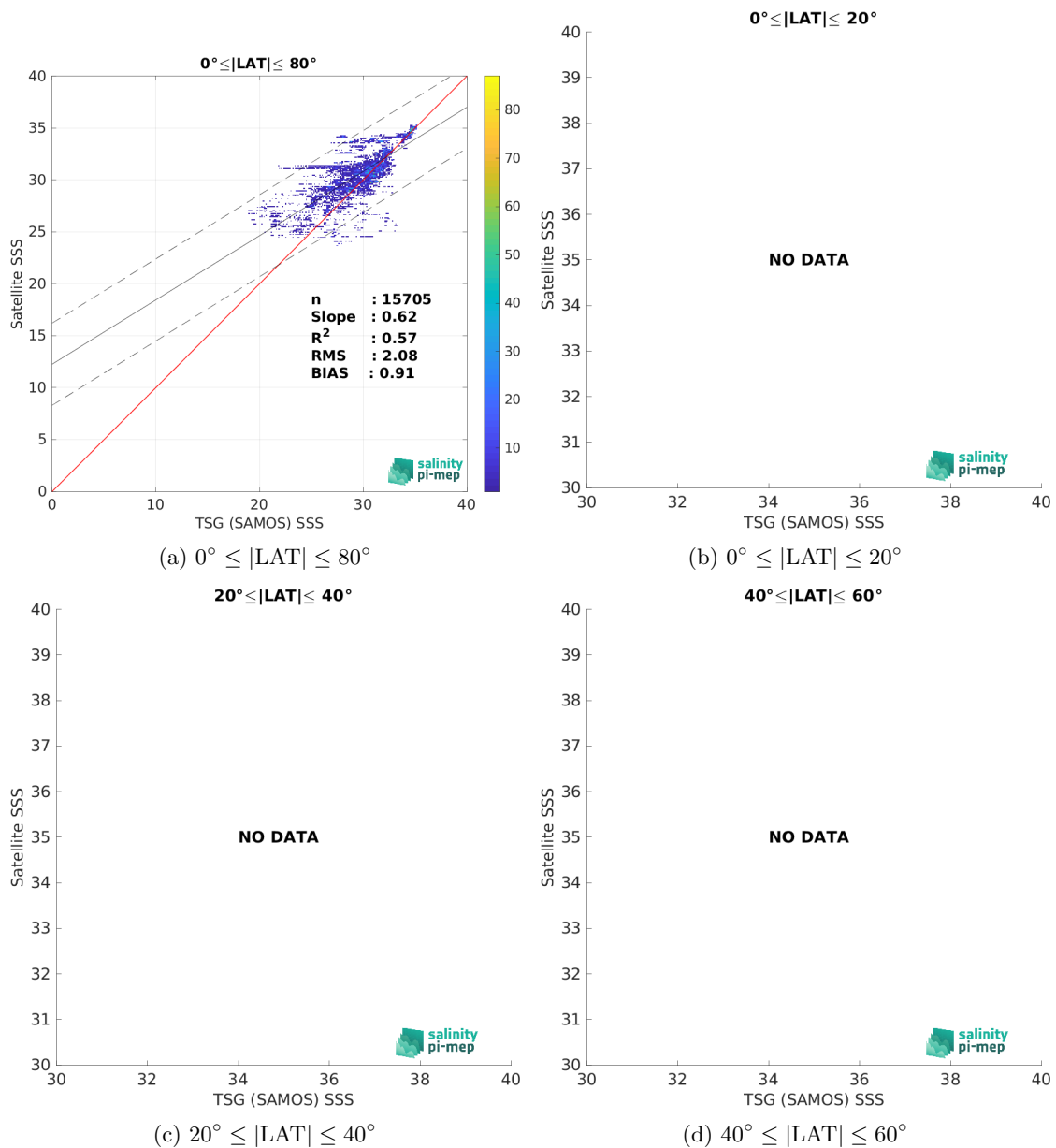
Figure 10: Contour maps of the concentration of SMOS SSS L3 Arctic v4 - 9 Days (BEC) SSS (y-axis) versus TSG (SAMOS) SSS (x-axis) at match-up pairs for different latitude bands. For each plot, the red line shows x=y . The black thin and dashed lines indicate a linear fit through the data cloud and the \pm 95\% confidence levels, respectively. The number match-up pairs n , the slope and R^2 coefficient of the linear fit, the root mean square (RMS) and the mean bias between satellite and in situ data are indicated for each latitude band in each plots.
