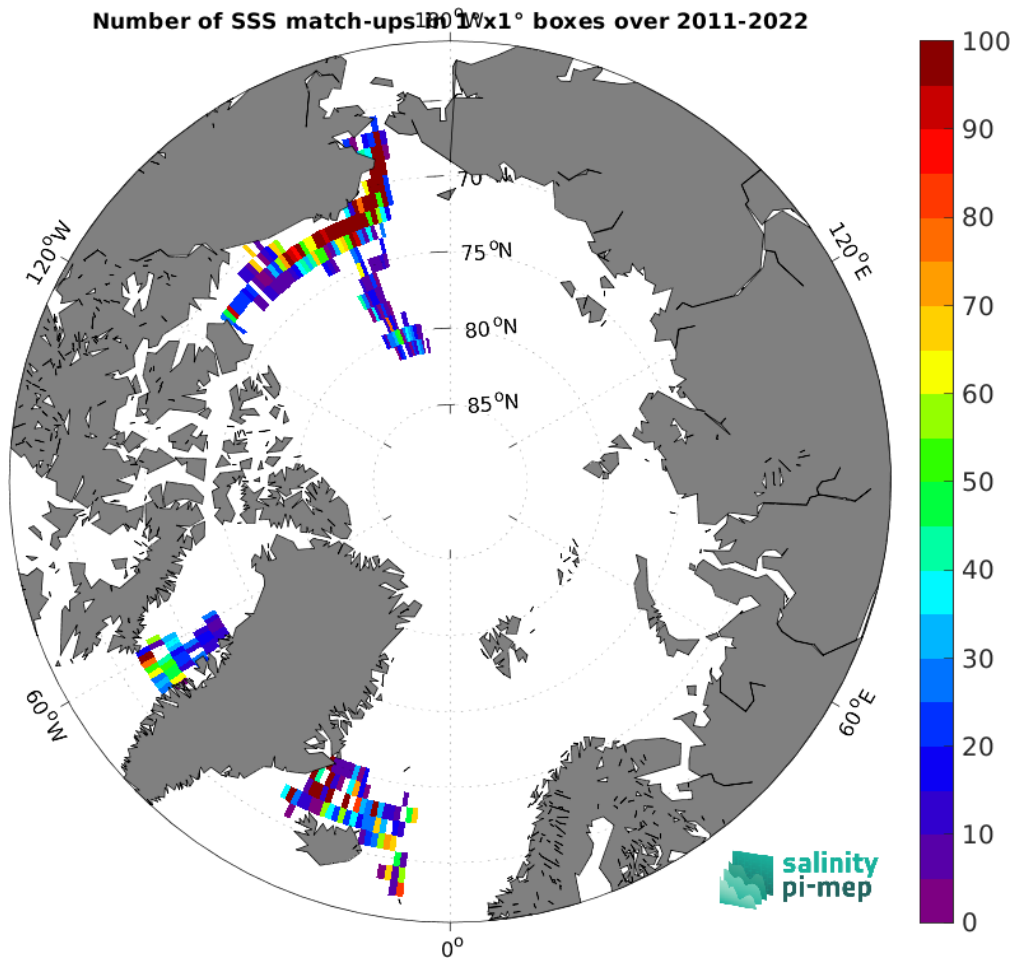
Figure 5: Number of SSS match-ups between TSG (SAMOS) SSS and the SMOS SSS L3 Arctic v4 - 9 Days (BEC) SSS product for the Arctic Ocean Pi-MEP region over 1^\circ \times 1^\circ boxes and for the full satellite product period.
