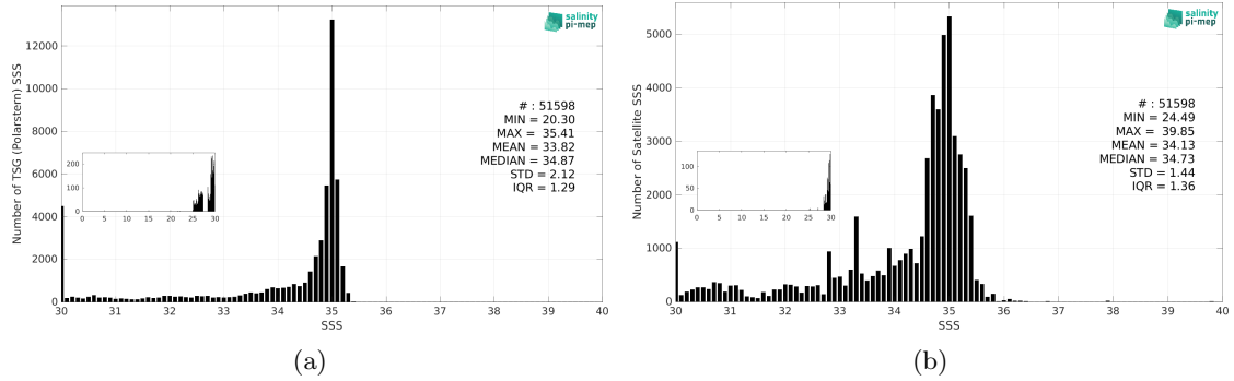
Figure 3: Histograms of SSS from TSG (Polarstern) (a) and SMOS SSS L3 Arctic v4 - 9 Days (BEC) (b) considering all match-up pairs per bins of 0.1 over the Arctic Ocean Pi-MEP region and for the full satellite product period.
