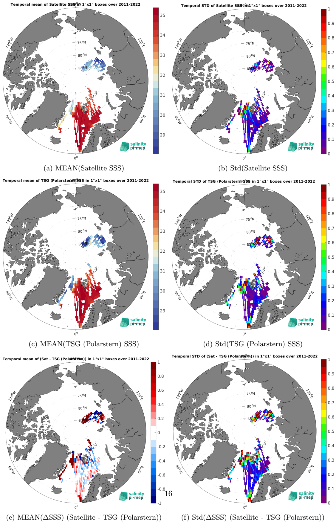
Figure 7: Temporal mean (left) and Std (right) of SSS from SMOS SSS L3 Arctic v4 - 9 Days (BEC) (top), TSG (Polarstern) (middle), and of \Delta SSS (Satellite - TSG (Polarstern)). Only match-up pairs are used to generate these maps.
