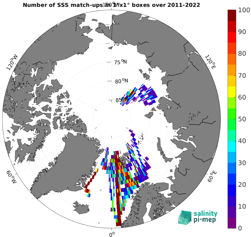
Figure 5: Number of SSS match-ups between TSG (Polarstern) SSS and the SMOS SSS L3 Arctic v4 - 9 Days (BEC) SSS product for the Arctic Ocean Pi-MEP region over 1^\circ \times 1^\circ boxes and for the full satellite product period.
