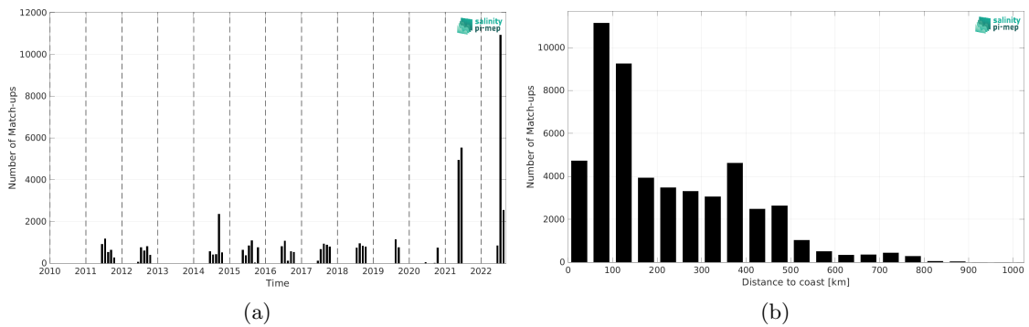
Figure 2: Number of match-ups between TSG (Polarstern) and SMOS SSS L3 Arctic v4 - 9 Days (BEC) SSS as a function of time (a) and as function of the distance to coast (b) over the Arctic Ocean Pi-MEP region and for the full satellite product period.
