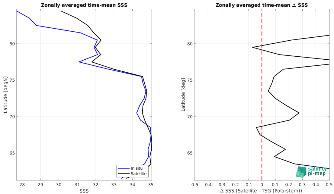
Figure 9: Left panel: Zonal mean SSS from SMOS SSS L3 Arctic v4 - 9 Days (BEC) satellite product (black) and from TSG (Polarstern) (blue). Right panel: Zonal mean of \Delta SSS (Satellite - TSG (Polarstern)) for all the collected Pi-MEP match-up pairs estimated over the full satellite product period.
