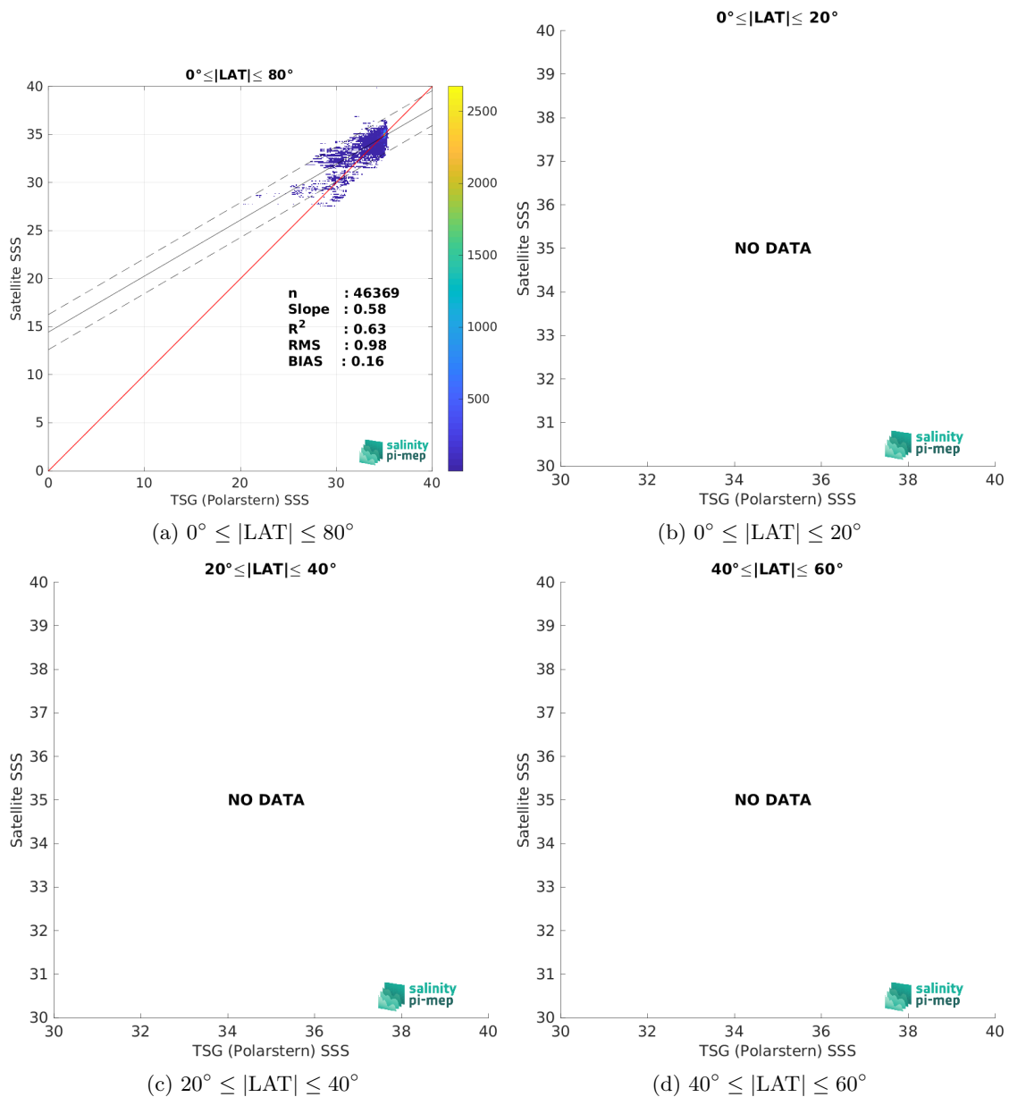
Figure 10: Contour maps of the concentration of SMOS SSS L3 Arctic v4 - 9 Days (BEC) SSS (y-axis) versus TSG (Polarstern) SSS (x-axis) at match-up pairs for different latitude bands. For each plot, the red line shows x=y . The black thin and dashed lines indicate a linear fit through the data cloud and the \pm 95\% confidence levels, respectively. The number match-up pairs n , the slope and R^2 coefficient of the linear fit, the root mean square (RMS) and the mean bias between satellite and in situ data are indicated for each latitude band in each plots.
