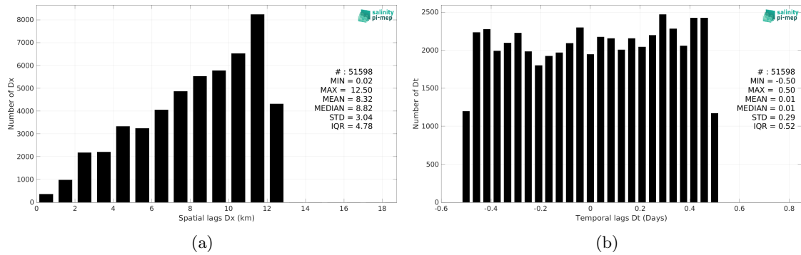
Figure 6: Histograms of the spatial (a) and temporal (b) lags between the location/time of the TSG (Polarstern) measurement and the date of the corresponding SMOS SSS L3 Arctic v4 - 9 Days (BEC) SSS pixel.
