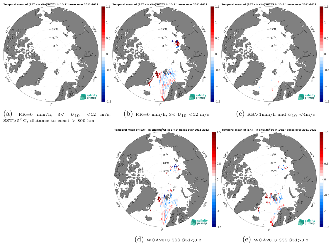
Figure 14: Temporal mean gridded over spatial boxes of size 1^\circ \times 1^\circ of \Delta SSS (SMOS SSS L3 Arctic v4 - 9 Days (BEC) - TSG (Polarstern)) for 5 different subdatasets corresponding to:RR=0 mm/h, 3 < U_{10} < 12 m/s, SST > 5°C, distance to coast > 800 km (a), RR=0 mm/h, 3 < U_{10} < 12 m/s (b), RR > 1mm/h and U_{10} < 4 m/s (c), WOA2013 SSS Std < 0.2 (d), WOA2013 SSS Std > 0.2 (e).
