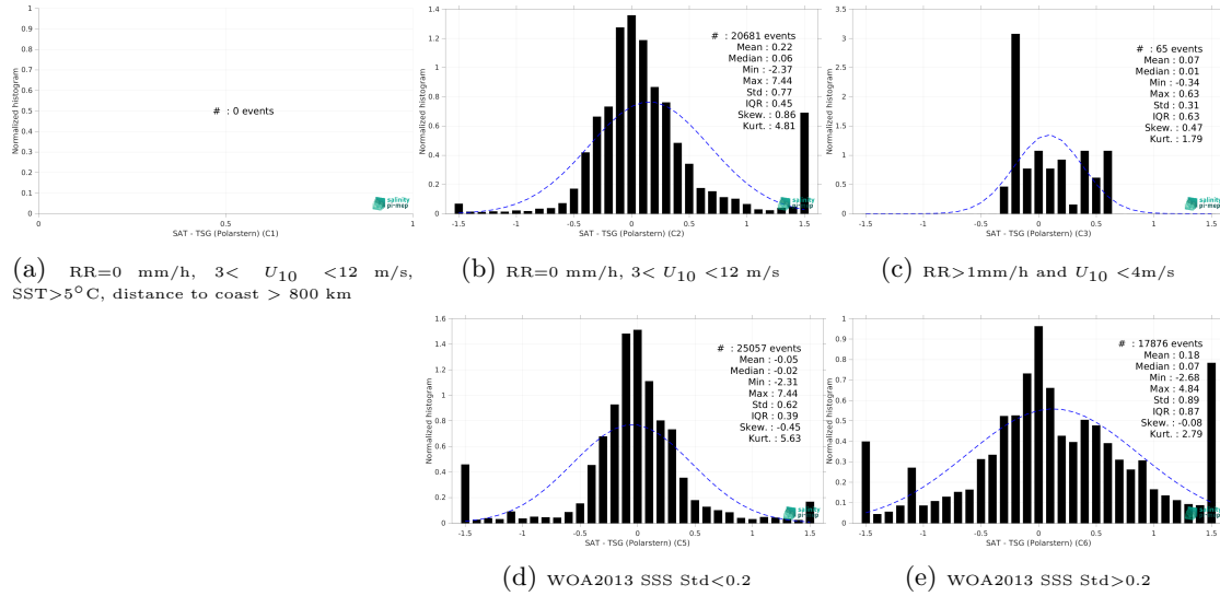
Figure 15: Normalized histogram of \Delta SSS (SMOS SSS L3 Arctic v4 - 9 Days (BEC) - TSG (Polarstern)) for 5 different subdatasets corresponding to: RR=0 mm/h, 3 < U_{10} < 12 m/s, SST > 5°C, distance to coast > 800 km (a), RR=0 mm/h, 3 < U_{10} < 12 m/s (b), RR > 1mm/h and U_{10} < 4 m/s (c), WOA2013 SSS Std < 0.2 (d), WOA2013 SSS Std > 0.2 (e).
