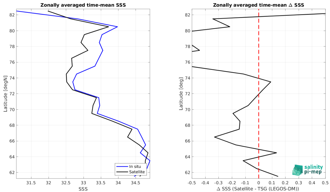
Figure 9: Left panel: Zonal mean SSS from SMOS SSS L3 Arctic v4 - 9 Days (BEC) satellite product (black) and from TSG (LEGOS-DM) (blue). Right panel: Zonal mean of \Delta SSS (Satellite - TSG (LEGOS-DM)) for all the collected Pi-MEP match-up pairs estimated over the full satellite product period.
