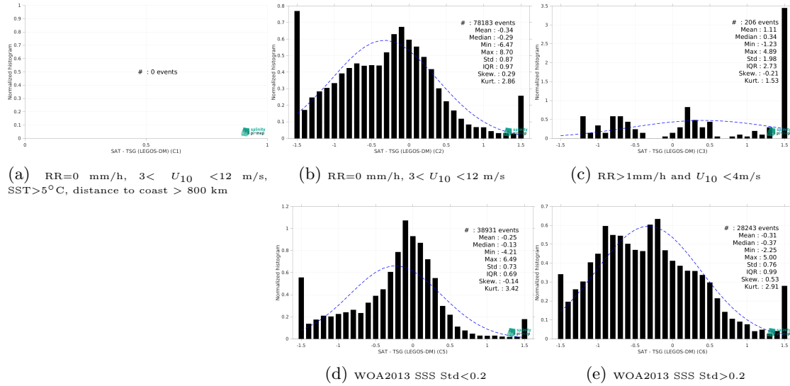
Figure 15: Normalized histogram of \Delta SSS (SMOS SSS L3 Arctic v4 - 9 Days (BEC) - TSG (LEGOS-DM)) for 5 different subdatasets corresponding to: RR=0 mm/h, 3 < U_{10} < 12 m/s, SST > 5°C, distance to coast > 800 km (a), RR=0 mm/h, 3 < U_{10} < 12 m/s (b), RR > 1mm/h and U_{10} < 4 m/s (c), WOA2013 SSS Std < 0.2 (d), WOA2013 SSS Std > 0.2 (e).
