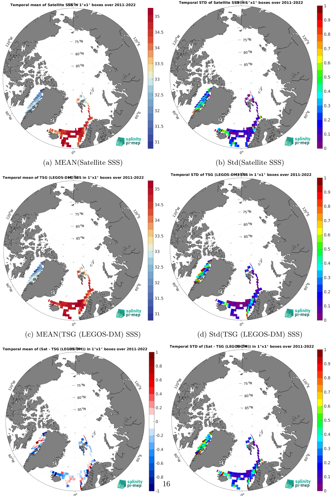
(e) MEAN( \Delta SSS) (Satellite - TSG (LEGOS-DM)) (f) Std( \Delta SSS) (Satellite - TSG (LEGOS-DM)) Figure 7: Temporal mean (left) and Std (right) of SSS from SMOS SSS L3 Arctic v4 - 9 Days (BEC) (top), TSG (LEGOS-DM) (middle), and of \Delta SSS (Satellite - TSG (LEGOS-DM)). Only match-up pairs are used to generate these maps.
