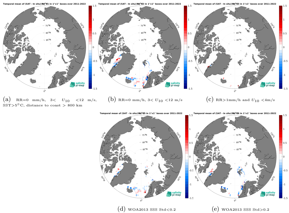
Figure 14: Temporal mean gridded over spatial boxes of size 1^\circ \times 1^\circ of \Delta SSS (SMOS SSS L3 Arctic v4 - 9 Days (BEC) - TSG (LEGOS-DM)) for 5 different subdatasets corresponding to:RR=0 mm/h, 3 < U_{10} < 12 m/s, SST >5^\circ C, distance to coast > 800 km (a), RR=0 mm/h, 3 < U_{10} < 12 m/s (b), RR >1 mm/h and U_{10} < 4 m/s (c), WOA2013 SSS Std <0.2 (d), WOA2013 SSS Std >0.2 (e).
