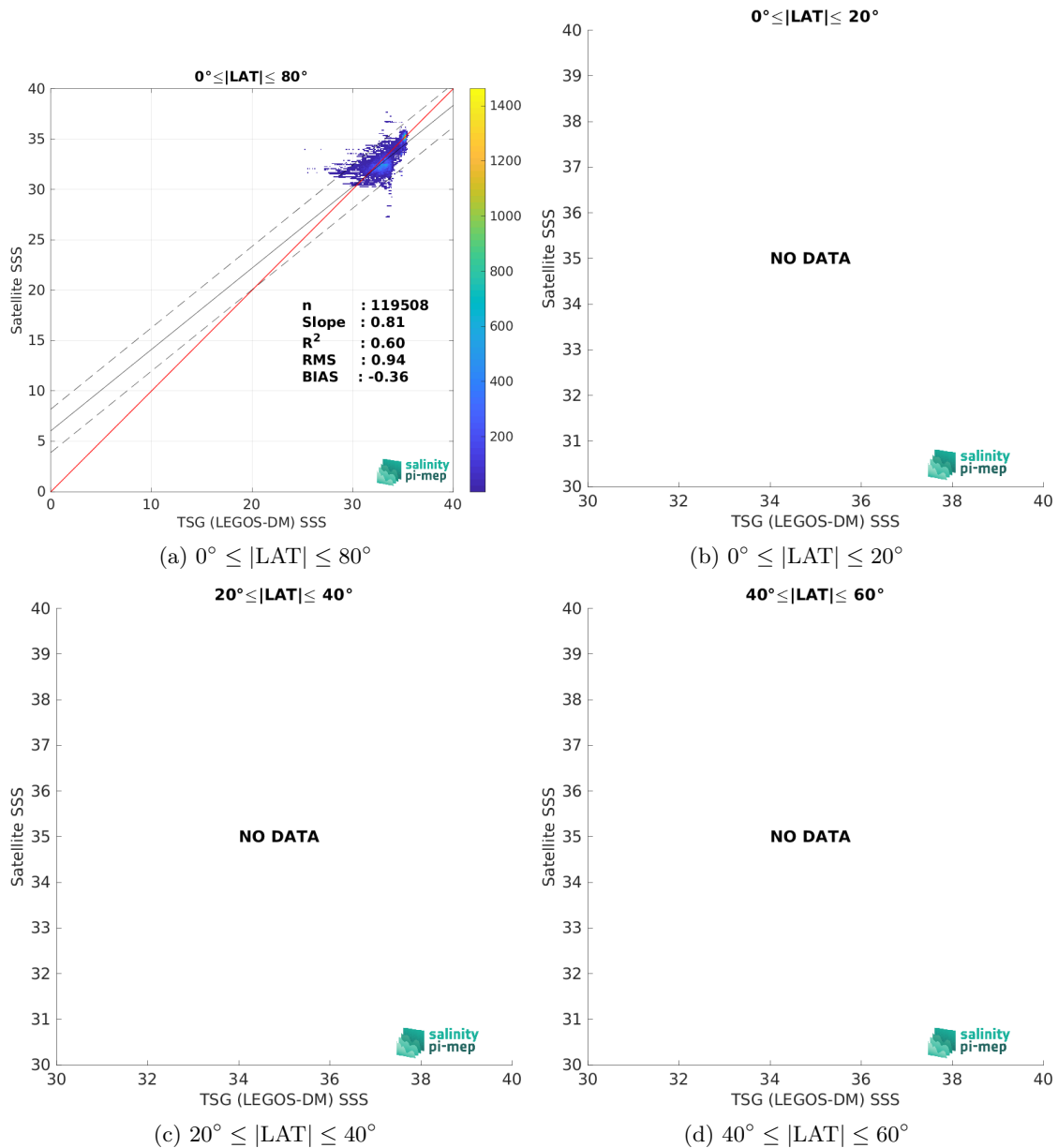
Figure 10: Contour maps of the concentration of SMOS SSS L3 Arctic v4 - 9 Days (BEC) SSS (y-axis) versus TSG (LEGOS-DM) SSS (x-axis) at match-up pairs for different latitude bands. For each plot, the red line shows x=y . The black thin and dashed lines indicate a linear fit through the data cloud and the \pm 95\% confidence levels, respectively. The number match-up pairs n , the slope and R^2 coefficient of the linear fit, the root mean square (RMS) and the mean bias between satellite and in situ data are indicated for each latitude band in each plots.
