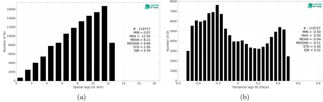
Figure 6: Histograms of the spatial (a) and temporal (b) lags between the location/time of the TSG (LEGOS-DM) measurement and the date of the corresponding SMOS SSS L3 Arctic v4 - 9 Days (BEC) SSS pixel.
