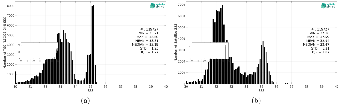
Figure 3: Histograms of SSS from TSG (LEGOS-DM) (a) and SMOS SSS L3 Arctic v4 - 9 Days (BEC) (b) considering all match-up pairs per bins of 0.1 over the Arctic Ocean Pi-MEP region and for the full satellite product period.
