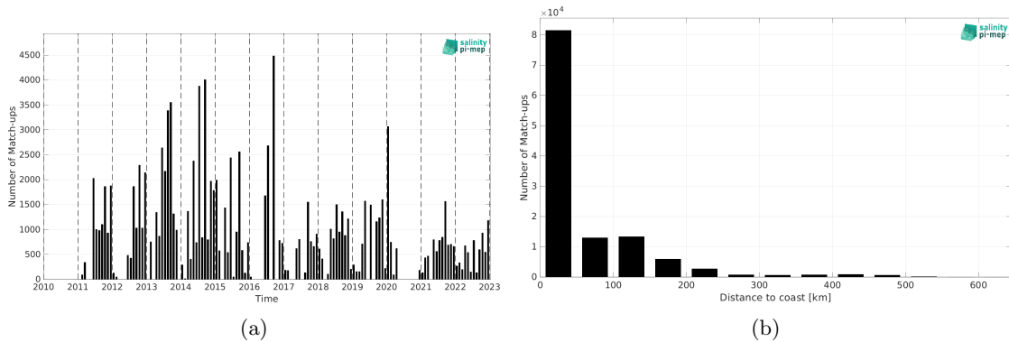
Figure 2: Number of match-ups between TSG (LEGOS-DM) and SMOS SSS L3 Arctic v4 - 9 Days (BEC) SSS as a function of time (a) and as function of the distance to coast (b) over the Arctic Ocean Pi-MEP region and for the full satellite product period.
