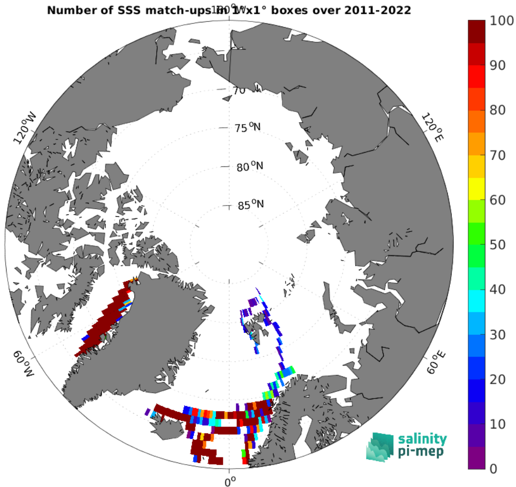
Figure 5: Number of SSS match-ups between TSG (LEGOS-DM) SSS and the SMOS SSS L3 Arctic v4 - 9 Days (BEC) SSS product for the Arctic Ocean Pi-MEP region over 1^\circ \times 1^\circ boxes and for the full satellite product period.
