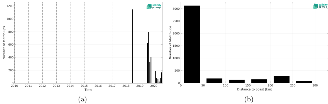
Figure 2: Number of match-ups between TSG (Lauge-Koch) and SMOS SSS L3 Arctic v4 - 9 Days (BEC) SSS as a function of time (a) and as function of the distance to coast (b) over the Arctic Ocean Pi-MEP region and for the full satellite product period.
