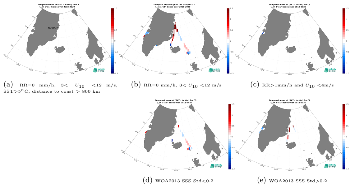
Figure 14: Temporal mean gridded over spatial boxes of size 1^\circ \times 1^\circ of \Delta SSS (SMOS SSS L3 Arctic v4 - 9 Days (BEC) - TSG (Lauge-Koch)) for 5 different subdatasets corresponding to:RR=0 mm/h, 3 < U_{10} < 12 m/s, SST >5^\circ\text{C} , distance to coast > 800 km (a), RR=0 mm/h, 3 < U_{10} < 12 m/s (b), RR >1 mm/h and U_{10} < 4 m/s (c), WOA2013 SSS Std <0.2 (d), WOA2013 SSS Std >0.2 (e).
