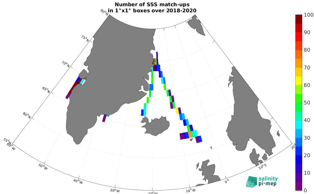
Figure 5: Number of SSS match-ups between TSG (Lauge-Koch) SSS and the SMOS SSS L3 Arctic v4 - 9 Days (BEC) SSS product for the Arctic Ocean Pi-MEP region over 1^\circ \times 1^\circ boxes and for the full satellite product period.
