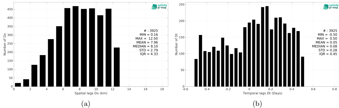
Figure 6: Histograms of the spatial (a) and temporal (b) lags between the location/time of the TSG (Lauge-Koch) measurement and the date of the corresponding SMOS SSS L3 Arctic v4 - 9 Days (BEC) SSS pixel.
