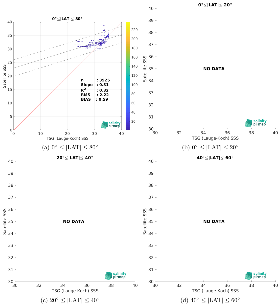
Figure 10: Contour maps of the concentration of SMOS SSS L3 Arctic v4 - 9 Days (BEC) SSS (y-axis) versus TSG (Lauge-Koch) SSS (x-axis) at match-up pairs for different latitude bands. For each plot, the red line shows x=y . The black thin and dashed lines indicate a linear fit through the data cloud and the \pm 95\% confidence levels, respectively. The number match-up pairs n , the slope and R^2 coefficient of the linear fit, the root mean square (RMS) and the mean bias between satellite and in situ data are indicated for each latitude band in each plots.
