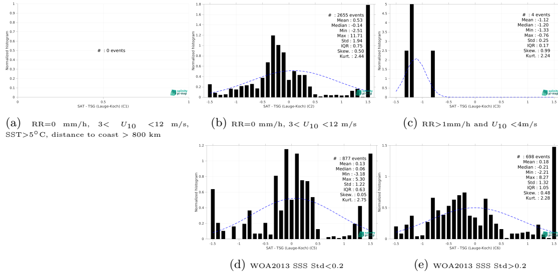
Figure 15: Normalized histogram of \Delta SSS (SMOS SSS L3 Arctic v4 - 9 Days (BEC) - TSG (Lauge-Koch)) for 5 different subdatasets corresponding to: RR=0 mm/h, 3 < U_{10} < 12 m/s, SST>5°C, distance to coast > 800 km (a), RR=0 mm/h, 3 < U_{10} < 12 m/s (b), RR>1mm/h and U_{10} < 4 m/s (c), WOA2013 SSS Std<0.2 (d), WOA2013 SSS Std>0.2 (e).
