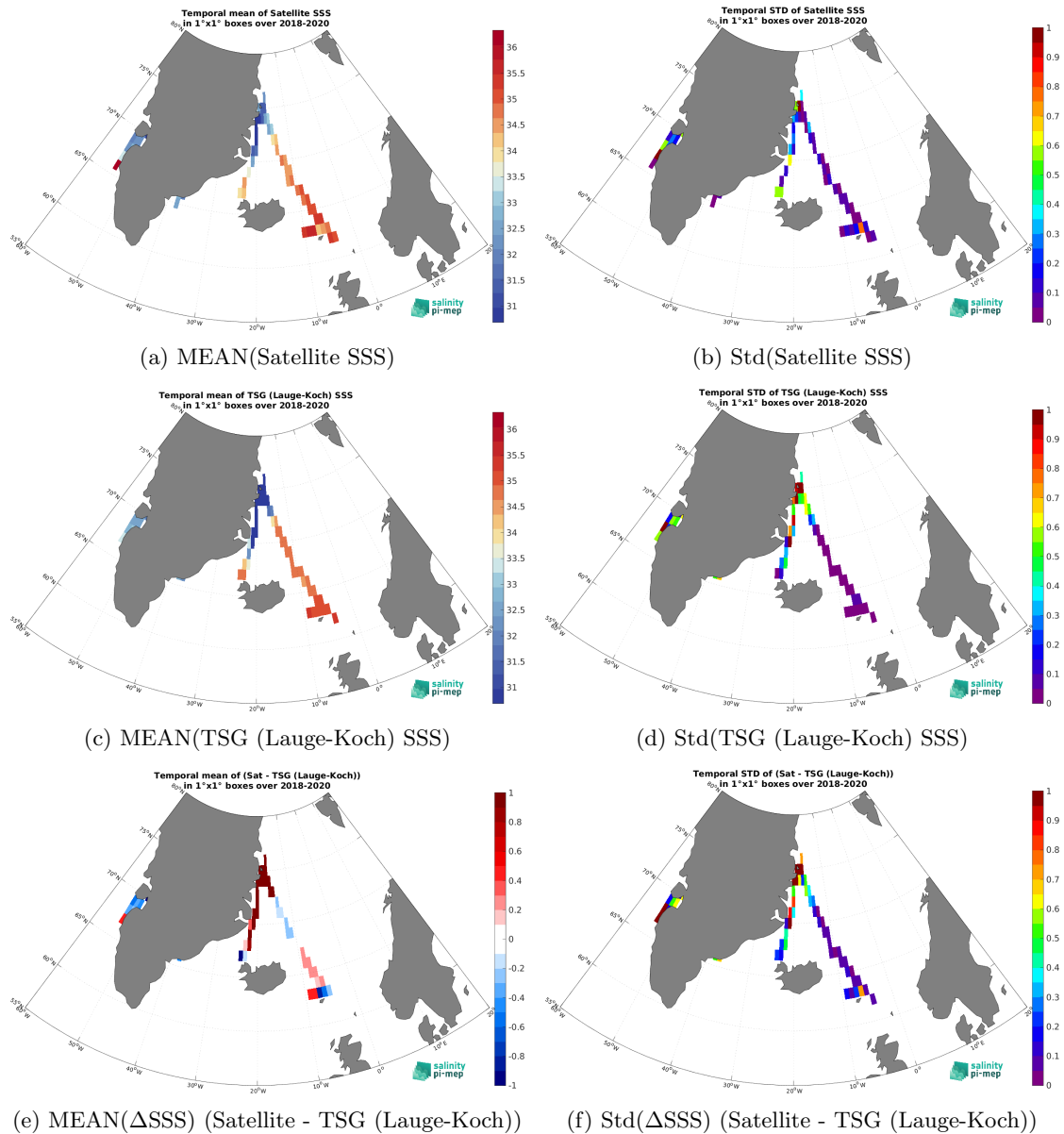
Figure 7: Temporal mean (left) and Std (right) of SSS from SMOS SSS L3 Arctic v4 - 9 Days (BEC) (top), TSG (Lauge-Koch) (middle), and of \Delta SSS (Satellite - TSG (Lauge-Koch)). Only match-up pairs are used to generate these maps.
