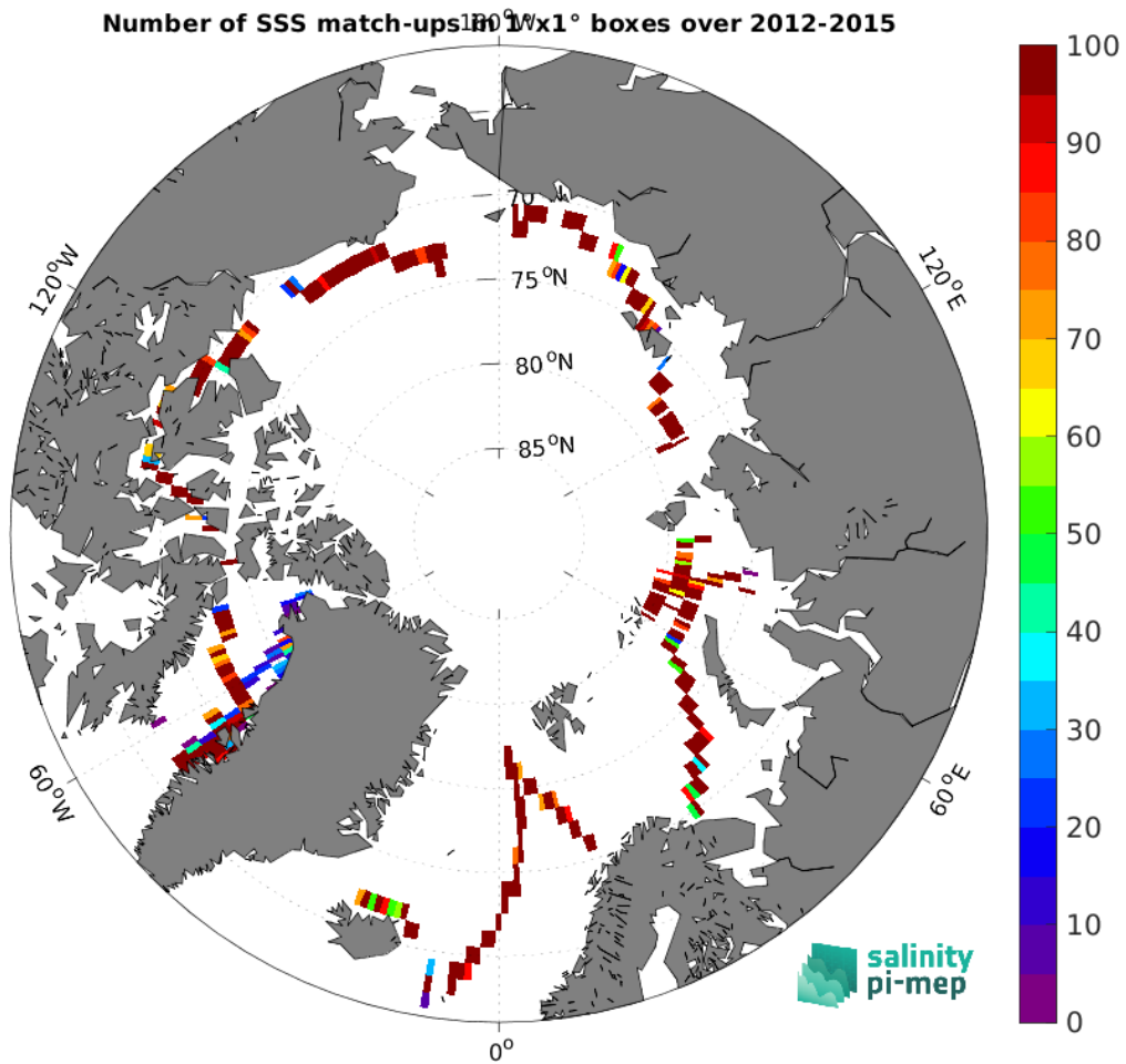
Figure 5: Number of SSS match-ups between TSG (GOSUD-Sailing-ship) SSS and the SMOS SSS L3 Arctic v4 - 9 Days (BEC) SSS product for the Arctic Ocean Pi-MEP region over 1^\circ \times 1^\circ boxes and for the full satellite product period.
