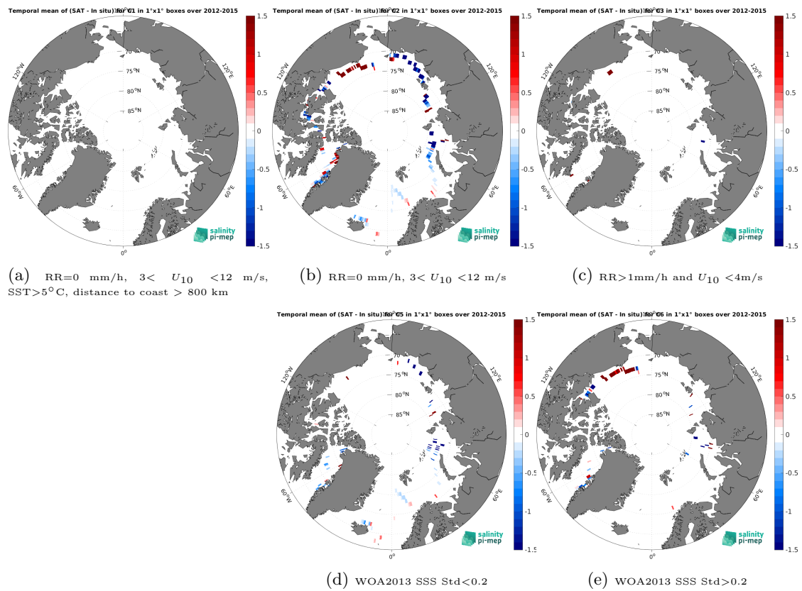
Figure 14: Temporal mean gridded over spatial boxes of size 1^\circ \times 1^\circ of \Delta\text{SSS} (SMOS SSS L3 Arctic v4 - 9 Days (BEC) - TSG (GOSUD-Sailing-ship)) for 5 different subdatasets corresponding to:RR=0 mm/h, 3 < U_{10} < 12 m/s, SST>5°C, distance to coast > 800 km (a), RR=0 mm/h, 3 < U_{10} < 12 m/s (b), RR>1mm/h and U_{10} < 4 m/s (c), WOA2013 SSS Std<0.2 (d), WOA2013 SSS Std>0.2 (e).
