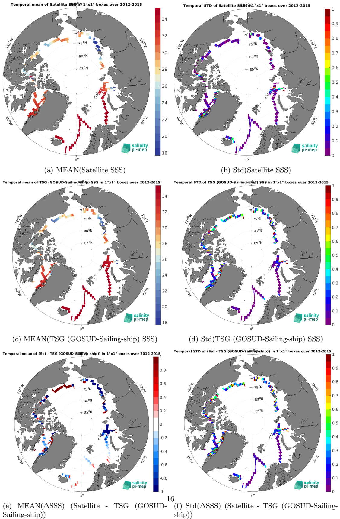
Figure 7: Temporal mean (left) and Std (right) of SSS from SMOS SSS L3 Arctic v4 - 9 Days (BEC) (top), TSG (GOSUD-Sailing-ship) (middle), and of \Delta SSS (Satellite - TSG (GOSUD-Sailing-ship)). Only match-up pairs are used to generate these maps.
