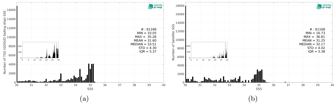
Figure 3: Histograms of SSS from TSG (GOSUD-Sailing-ship) (a) and SMOS SSS L3 Arctic v4 - 9 Days (BEC) (b) considering all match-up pairs per bins of 0.1 over the Arctic Ocean Pi-MEP region and for the full satellite product period.
