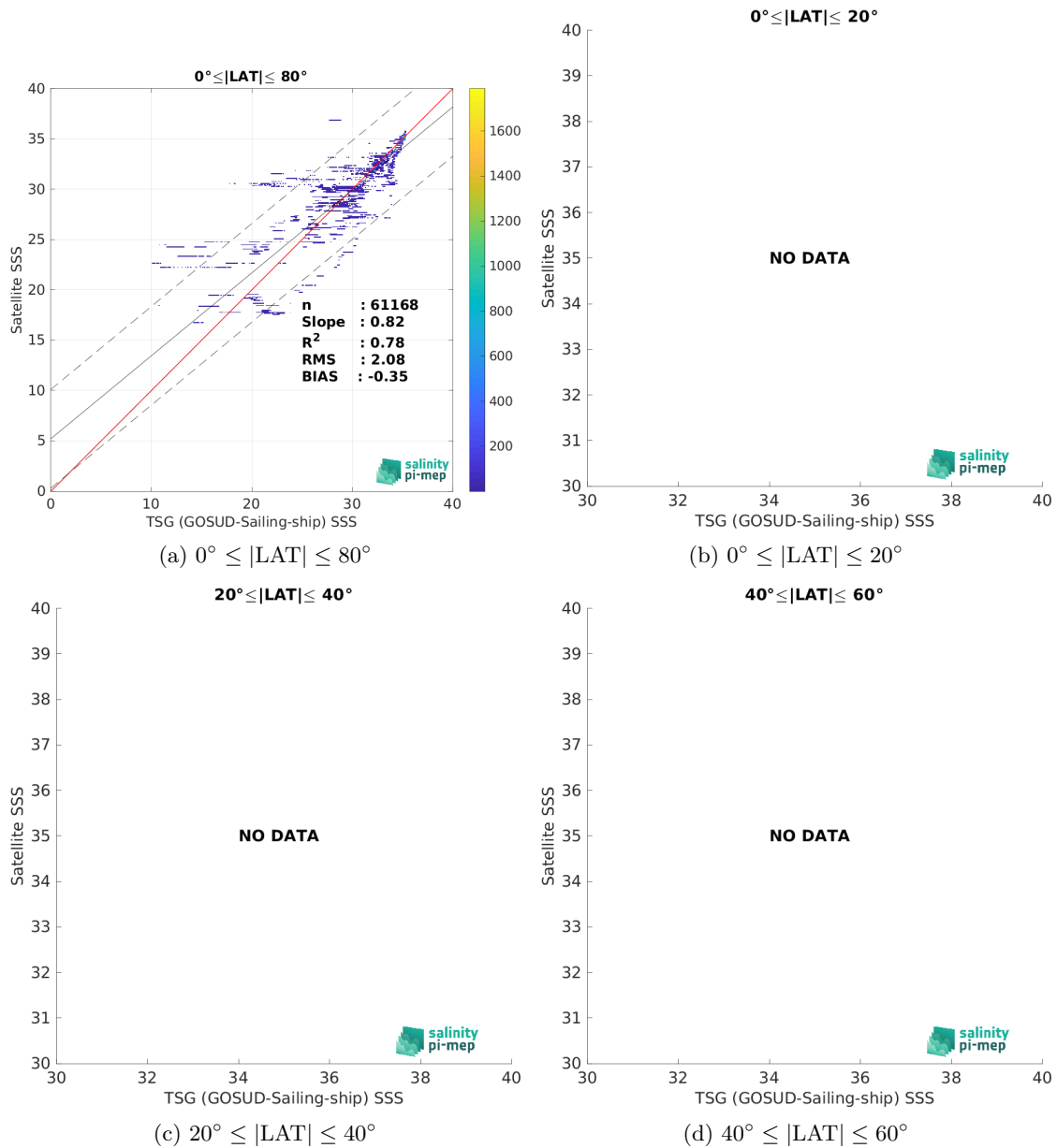
Figure 10: Contour maps of the concentration of SMOS SSS L3 Arctic v4 - 9 Days (BEC) SSS (y-axis) versus TSG (GOSUD-Sailing-ship) SSS (x-axis) at match-up pairs for different latitude bands. For each plot, the red line shows x=y . The black thin and dashed lines indicate a linear fit through the data cloud and the \pm 95\% confidence levels, respectively. The number match-up pairs n , the slope and R^2 coefficient of the linear fit, the root mean square (RMS) and the mean bias between satellite and in situ data are indicated for each latitude band in each plots.
