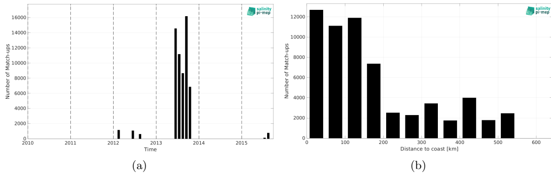
Figure 2: Number of match-ups between TSG (GOSUD-Sailing-ship) and SMOS SSS L3 Arctic v4 - 9 Days (BEC) SSS as a function of time (a) and as function of the distance to coast (b) over the Arctic Ocean Pi-MEP region and for the full satellite product period.
