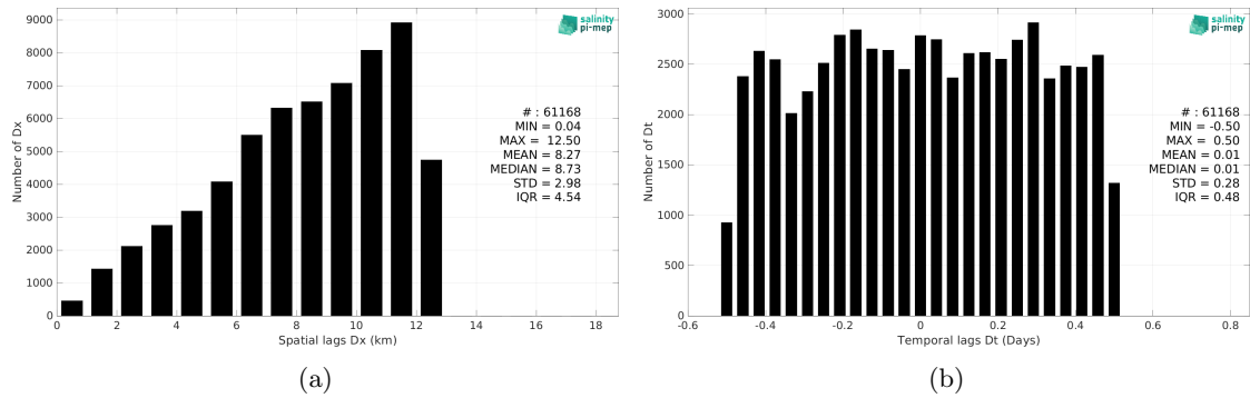
Figure 6: Histograms of the spatial (a) and temporal (b) lags between the location/time of the TSG (GOSUD-Sailing-ship) measurement and the date of the corresponding SMOS SSS L3 Arctic v4 - 9 Days (BEC) SSS pixel.
