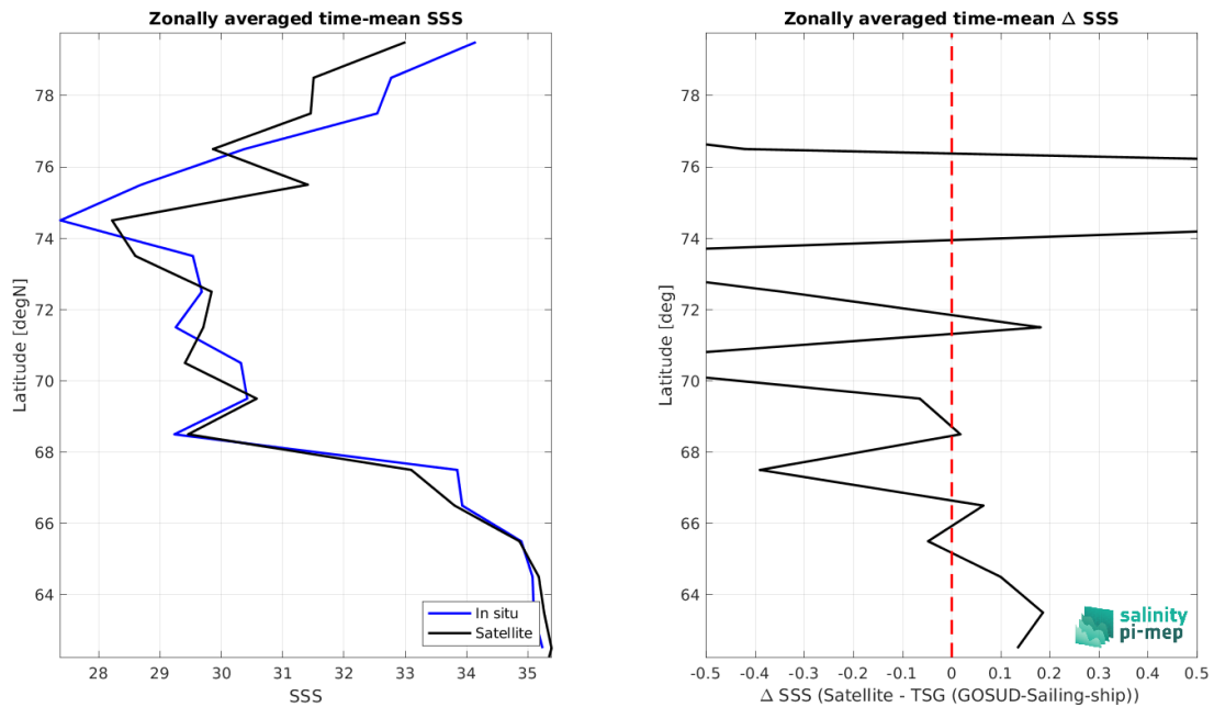
Figure 9: Left panel: Zonal mean SSS from SMOS SSS L3 Arctic v4 - 9 Days (BEC) satellite product (black) and from TSG (GOSUD-Sailing-ship) (blue). Right panel: Zonal mean of \Delta SSS (Satellite - TSG (GOSUD-Sailing-ship)) for all the collected Pi-MEP match-up pairs estimated over the full satellite product period.
