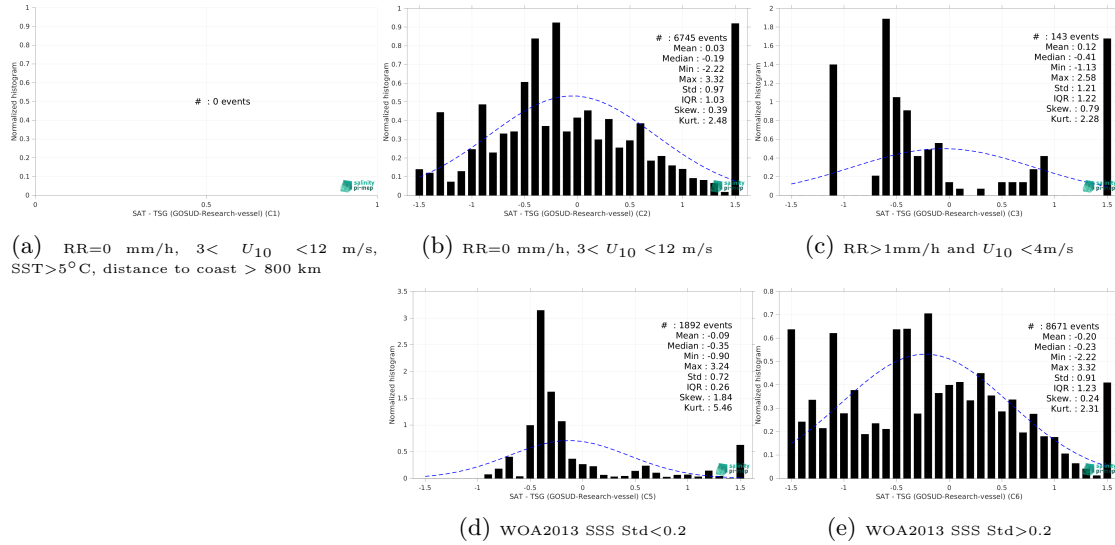
Figure 15: Normalized histogram of \Delta SSS (SMOS SSS L3 Arctic v4 - 9 Days (BEC) - TSG (GOSUD-Research-vessel)) for 5 different subdatasets corresponding to: RR=0 mm/h, 3 < U_{10} < 12 m/s, SST > 5°C, distance to coast > 800 km (a), RR=0 mm/h, 3 < U_{10} < 12 m/s (b), RR > 1mm/h and U_{10} < 4 m/s (c), WOA2013 SSS Std < 0.2 (d), WOA2013 SSS Std > 0.2 (e).
