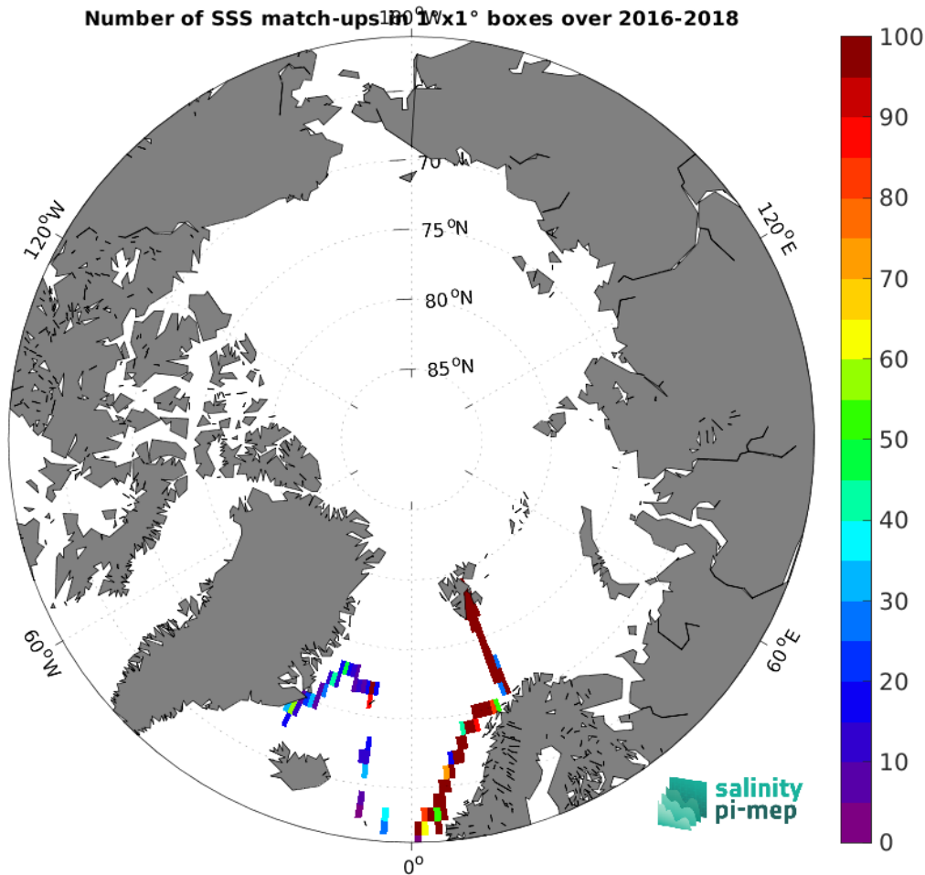
Figure 5: Number of SSS match-ups between TSG (GOSUD-Research-vessel) SSS and the SMOS SSS L3 Arctic v4 - 9 Days (BEC) SSS product for the Arctic Ocean Pi-MEP region over 1^\circ \times 1^\circ boxes and for the full satellite product period.
