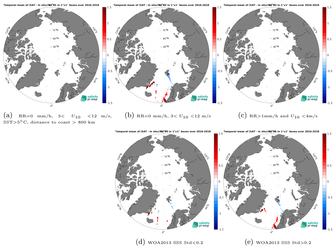
Figure 14: Temporal mean gridded over spatial boxes of size 1^\circ \times 1^\circ of \Delta SSS (SMOS SSS L3 Arctic v4 - 9 Days (BEC) - TSG (GOSUD-Research-vessel)) for 5 different subdatasets corresponding to: RR=0 mm/h, 3 < U_{10} < 12 m/s, SST > 5^\circ\text{C} , distance to coast > 800 km (a), RR=0 mm/h, 3 < U_{10} < 12 m/s (b), RR > 1 mm/h and U_{10} < 4 m/s (c), WOA2013 SSS Std < 0.2 (d), WOA2013 SSS Std > 0.2 (e).
