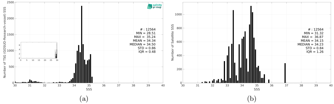
Figure 3: Histograms of SSS from TSG (GOSUD-Research-vessel) (a) and SMOS SSS L3 Arctic v4 - 9 Days (BEC) (b) considering all match-up pairs per bins of 0.1 over the Arctic Ocean Pi-MEP region and for the full satellite product period.
