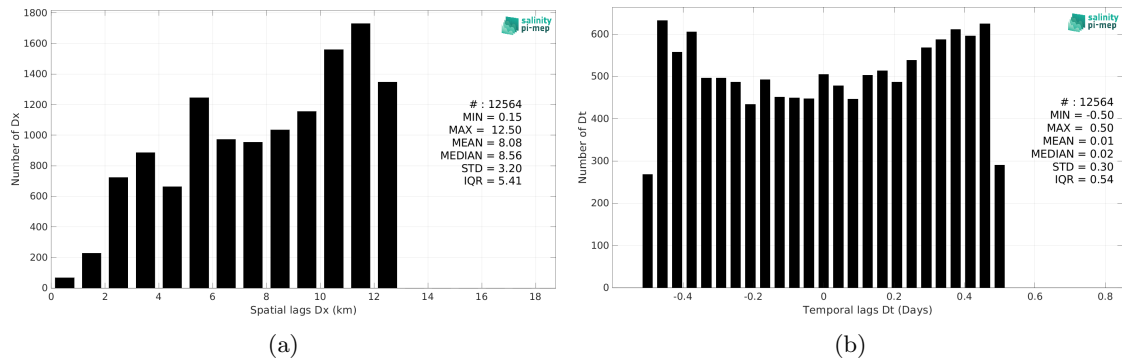
Figure 6: Histograms of the spatial (a) and temporal (b) lags between the location/time of the TSG (GOSUD-Research-vessel) measurement and the date of the corresponding SMOS SSS L3 Arctic v4 - 9 Days (BEC) SSS pixel.
