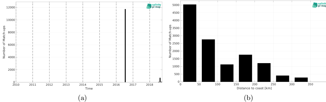
Figure 2: Number of match-ups between TSG (GOSUD-Research-vessel) and SMOS SSS L3 Arctic v4 - 9 Days (BEC) SSS as a function of time (a) and as function of the distance to coast (b) over the Arctic Ocean Pi-MEP region and for the full satellite product period.
