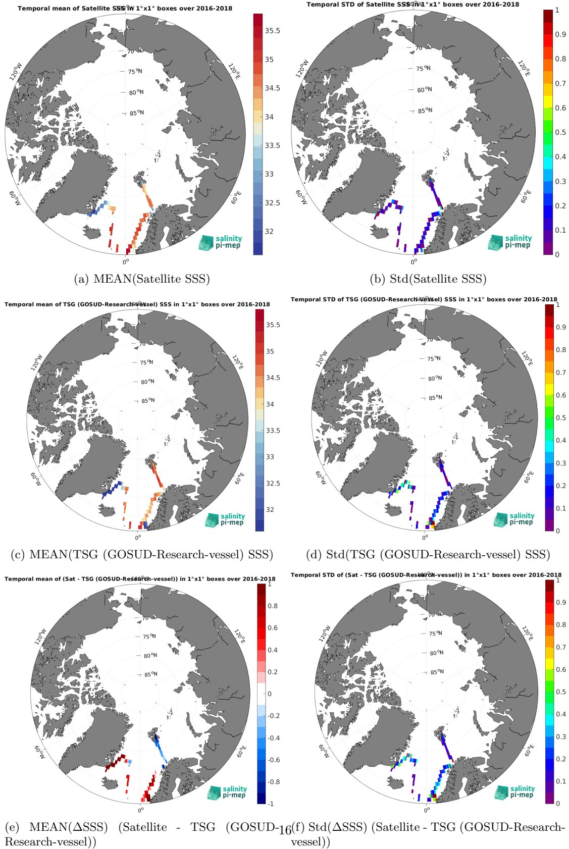
Figure 7: Temporal mean (left) and Std (right) of SSS from SMOS SSS L3 Arctic v4 - 9 Days (BEC) (top), TSG (GOSUD-Research-vessel) (middle), and of \Delta SSS (Satellite - TSG (GOSUD-Research-vessel)). Only match-up pairs are used to generate these maps.
